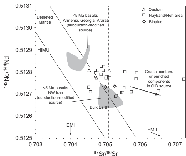
Fig. 5. Nd–Sr isotope composition of samples from Quchan (this study), Binalud (Saadat and Stern, 2012), the Nayband/Neh Fault system (Saadat and Stern, 2010; Pang et al., 2012), and compilations from NW Iran (Kheirkhah et al., 2013) and selected subduction-modified centres in the Caucasus and Eastern Anatolia (Neill et al., 2013a).
