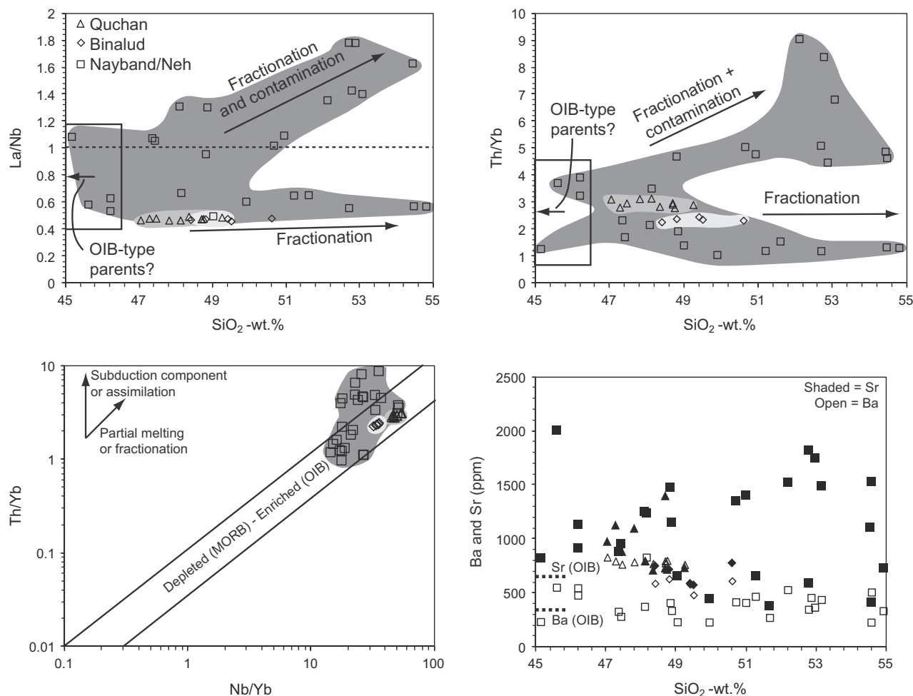
Fig. 7. Trace element variation plots to identify crustal contamination and fractionation effects. (a) La/Nb vs. SiO 2 . (b) Th/Yb vs. SiO 2 . (c) Th/Yb vs. Nb/Yb after Pearce and Peate (1995) . (d) Ba and Sr vs. SiO 2 with OIB values from Sun and McDonough (1989) .
