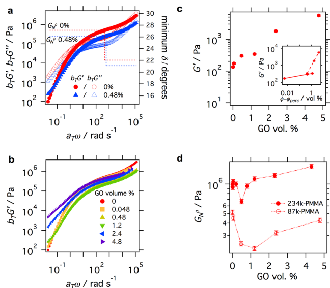
Figure 3. Rheological characterizations of PMMA/GO nanocomposites. (a) G' (solid symbols) and G'' (open symbols) of pure 87k-PMMA and 87k-PMMA/0.48 vol % GO composite as a function of frequency. (b) G' across the full concentration range studied for PMMA composites, as a function of frequency. (a) and (b) subject to TTS at a reference temperature of 200 °C. (c) Build up of G' with GO concentration at a fixed frequency of 0.02512 rad s -1 at a temperature of 200 °C for 87k- and 234k-PMMA composites. Inset shows application of a percolation model with G' as a function of the difference between GO vol % and percolation volume %. (d) The plateau modulus of the PMMA composites as a function of GO concentration.
