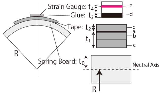
Fig. A1 The detail of the strain applied by using the springboard, where a, b, c, d and e are the superconducting layer, substrate, lamination layer, glue and sensing element of the strain gauge.
