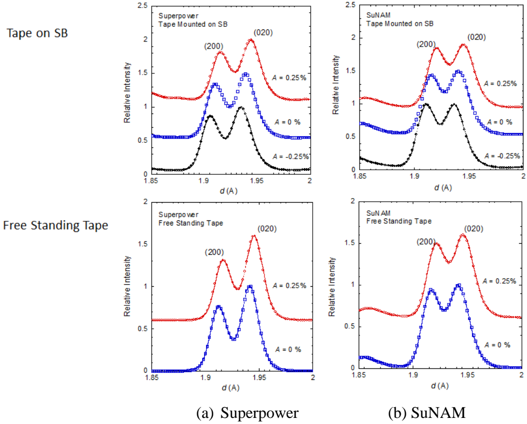
Fig. 4 Diffraction profile of (200) and (020) crystal planes under the axial strains as a function of lattice spacing for two kinds of tapes at room temperature
