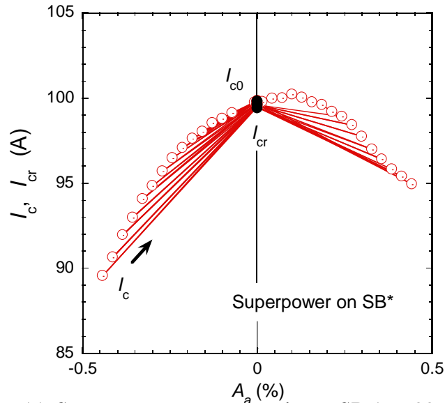
(a) Superpower tape mounted on a SB ( I_{c0}=99.6 A)
