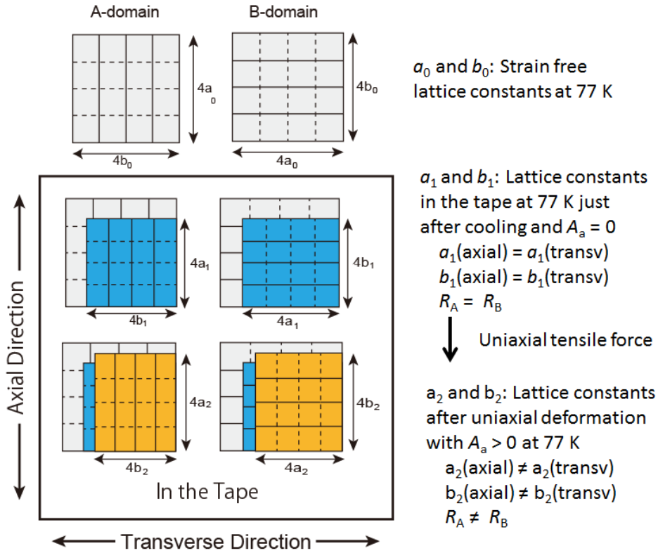
Fig. 11 The change of lattice constants due to the cooling as well as the uniaxial deformation. Here the shape of a 4 x 4 REBCO set of unit cells in the A-domain and in the B-domain of a REBCO tape is given. The dotted lines in the domains denote the direction of the Cu-O chains.
