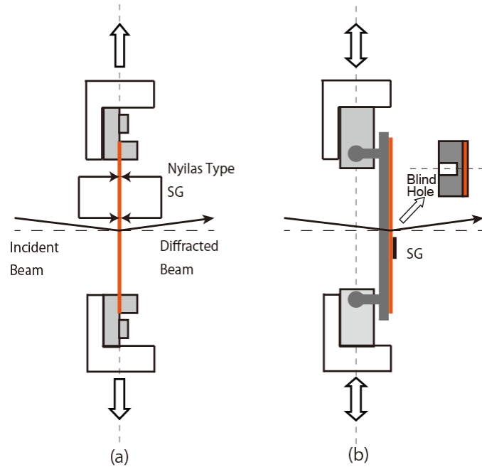
Fig.3 Sample holders for diffraction experiments
