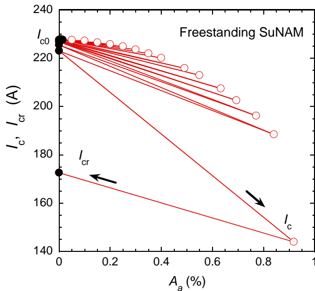
(b) Freestanding SuNAM tape ( I_{c0}=227 A)
