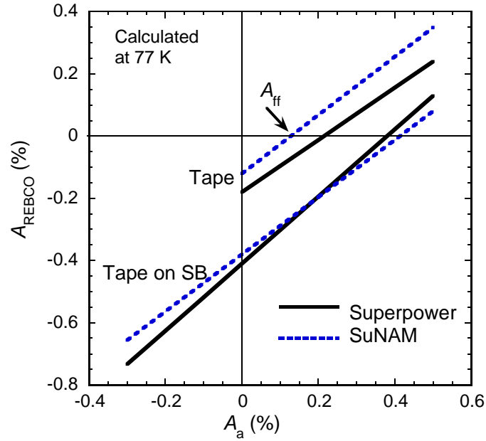
Fig. 7 The calculated local strain exerted on the REBCO layer at 77 K as a function of applied strain for both the Superpower tape and the SuNAM tape when freestanding and when mounted on SB.
