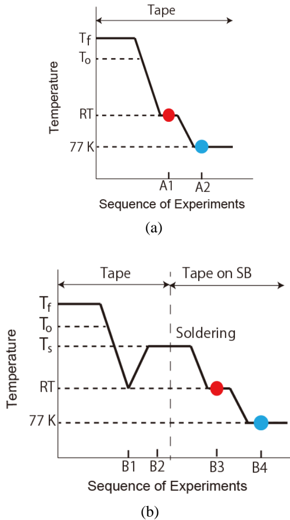
Fig. 2 Thermal history and sample preparation in the present experiments. (a) the free standing tape and (b) the tape mounted on a spring board
