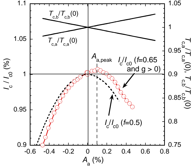
Fig. 12 Schematic relation for the critical current and critical temperature as a function of the applied strain
