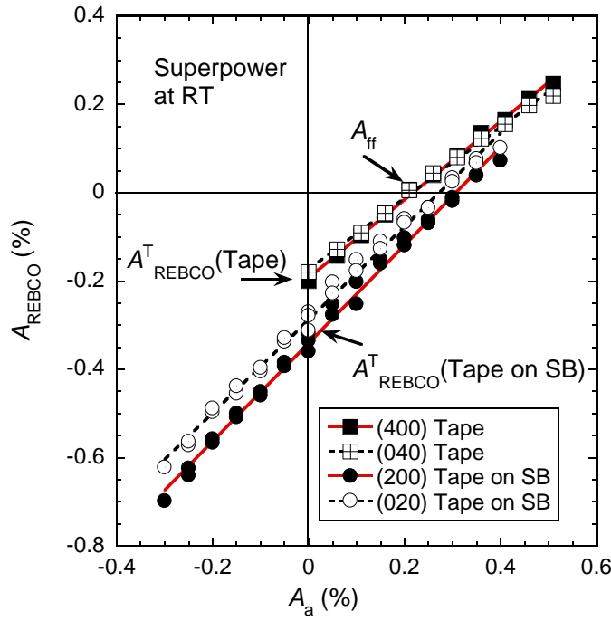
(a) Superpower tape
