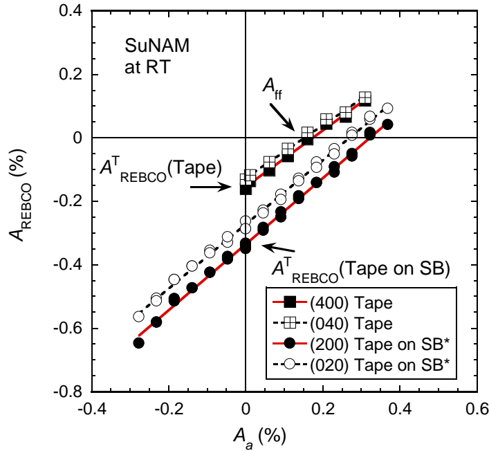
(b) SuNAM tape
