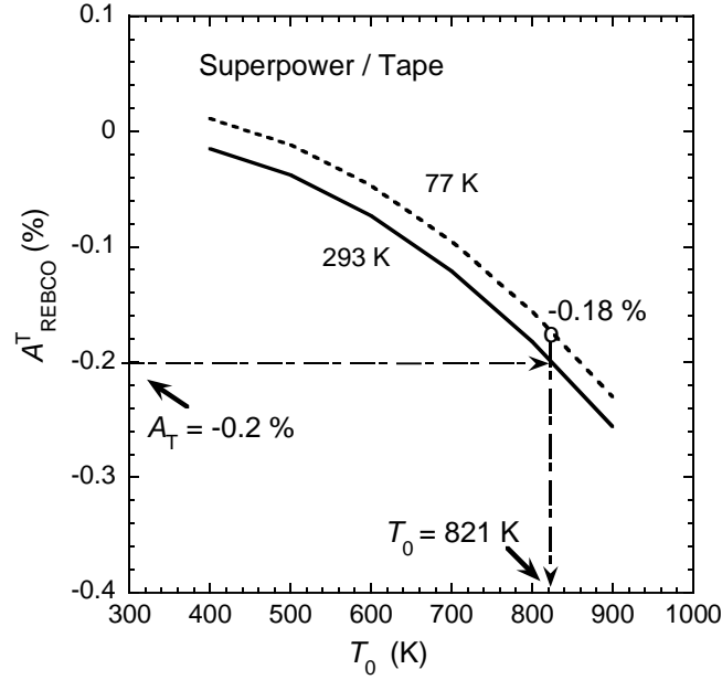
Fig. 6 Thermal strain exerted on the REBCO layer at 293 and 77 K as a function of T_0 in the Superpower tape
