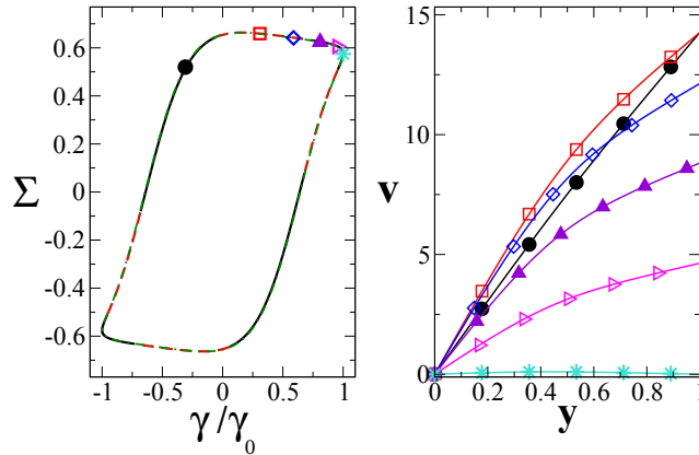
FIG. 12. sRP model with a monotonic constitutive curve in LAOStrain of strain rate amplitude \dot{\gamma}_0 = 20.0 and frequency \omega = 8.0 . Model parameters \beta = 0.7, Z = 75, \eta = 10^{-5} . Cell curvature q = 2 \times 10^{-3} . Number of numerical grid points J = 512 . Left: stress response in the elastic representation. Solid black and red-dashed line: calculation in which the flow is constrained to be homogeneous. Red-dashed region indicates a positive eigenvalue showing instability to the onset of shear banding. Green dot-dashed line: stress response in a full nonlinear simulation that allows banding (almost indistinguishable from homogeneous signal in this case.) Right: Velocity profiles corresponding to stages in the cycle indicated by matching symbols in left panel.
