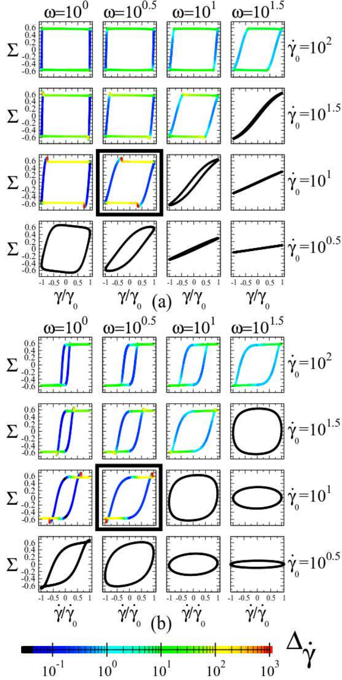
FIG. 6. Lissajous-Bowditch curves in LAOStrain for the nRP model with a non-monotonic constitutive curve. Results are shown in the elastic representation in (a), and the viscous representation in (b). Columns of fixed frequency \omega and rows of fixed strain-rate amplitude \dot{\gamma}_0 are labeled at the top and right-hand side. Colourscale shows the time-dependent degree of shear banding. Model parameters: \beta = 0.4, \eta = 10^{-5} . Cell curvature: q = 10^{-4} . Number of numerical grid points J = 512 . A detailed portrait of the run outlined by the thicker box is shown in Fig. 8.
