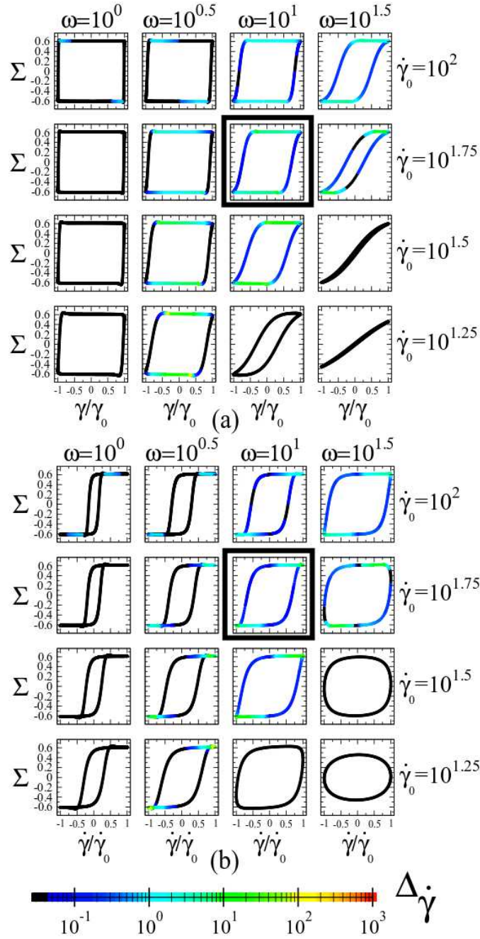
FIG. 7. As in Fig. 6 but for a value of the CCR parameter \beta = 1.0 , for which the fluid's underlying constitutive curve is monotonic. Number of numerical grid points J = 512 . A detailed portrait of the run outlined by the thicker box is shown in Fig. 9.
