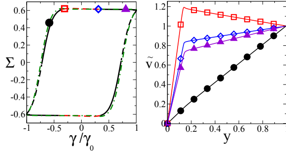
FIG. 9. As in Fig. 8 but for the nRP model with a CCR parameter \beta = 1.0 for which the underlying homogeneous constitutive curve is monotonic, and for a LAOstrain with strain rate amplitude \gamma_0 = 56.2 and frequency \omega = 10.0 . Number of numerical grid points J = 512 .
