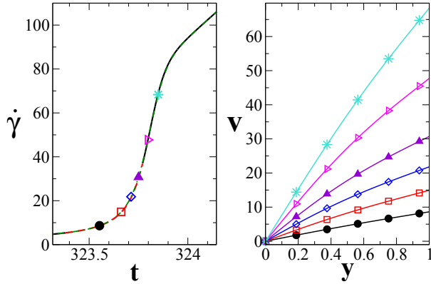
FIG. 22. sRP model with a monotonic constitutive curve in LAOStress of stress amplitude \Sigma_0 = 0.8 and frequency \omega = 0.1 . Model parameters \beta = 0.7, Z = 100, \eta = 3.16 \times 10^{-5} . Cell curvature q = 2 \times 10^{-3} . Number of numerical grid points J = 512 . Left: strain rate signal versus time. Solid black and red-dashed line: calculation in which the flow is constrained to be homogeneous. Red-dashed region indicates a positive eigenvalue showing instability to the onset of shear banding. Green dot-dashed line: stress response in a full nonlinear simulation that allows banding (indistinguishable from homogeneous signal in this case.) Right: Velocity profiles corresponding to stages in the cycle indicated by matching symbols in left panel.
