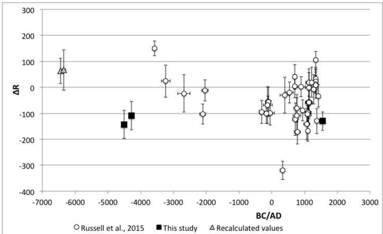
Figure 2: Graph of \Delta R values for Scottish coastal waters through the Holocene showing new values (black squares) and recalculated values (grey triangles) alongside previous values for Scottish waters (white circles: Ascough et al., 2004, 2006, 2007, 2009, Russell et al., 2010, 2011b, 2015).
