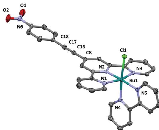
Fig. 4 The cation in the crystal structure of [\mathbf{4Cl}]\text{PF}_6 \cdot 2\text{CH}_3\text{CN} . Hydrogen atoms removed for clarity.
