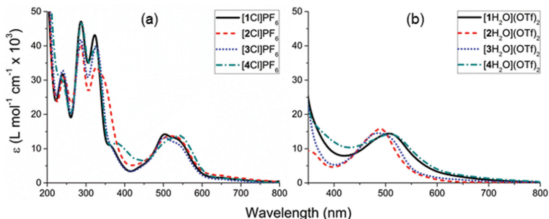
Fig. 6 Electronic absorbance spectra of: (a) complexes [1-4\text{Cl}]\text{PF}_6 in acetonitrile, (b) complexes [1-4\text{H}_2\text{O}](\text{OTf})_2 in an acetone : water (9 : 1) solution.
