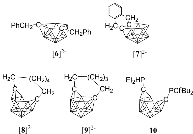
Figure 11. Geometries of nido -dicarbadoecaboranes determined by X-ray crystallography.
