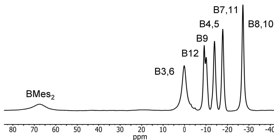
Figure 14: ^{11}\text{B}\{^1\text{H}\} NMR spectrum of [\mathbf{2}]^{2-} in \text{CD}_3\text{CN} with peak assignments based on GIAO-NMR data.
