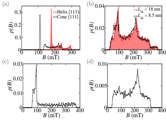
FIG. 4. The p(B) distribution in an applied field of B_a = 150 mT. (a) Helical and conical magnetic structures. (b) The p(B) distribution for the SL magnetic structure with lattice constants L_{\text{sk}} = 8.5 nm and 18 nm. (c),(d) field distributions at stopping sites 0 and 1 respectively, for the SL structure.
