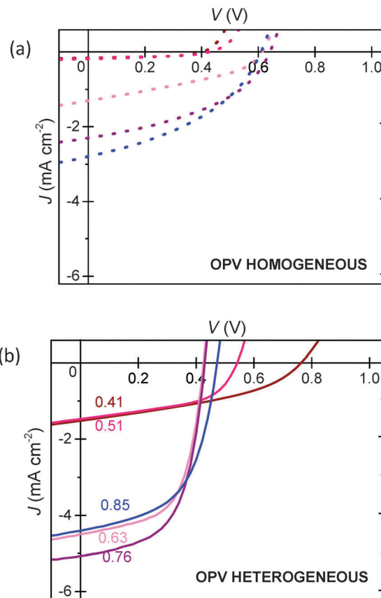
Fig. 6 J - V characteristics of (a) homogeneous and (b) heterogeneous P3HT:PCBM OPVs under AM1.5 illumination with various blend ratios: p_{\text{P3HT}} = 0.41 (brown), 0.51 (red), 0.63 (pink), 0.76 (purple) and 0.85 (blue).
