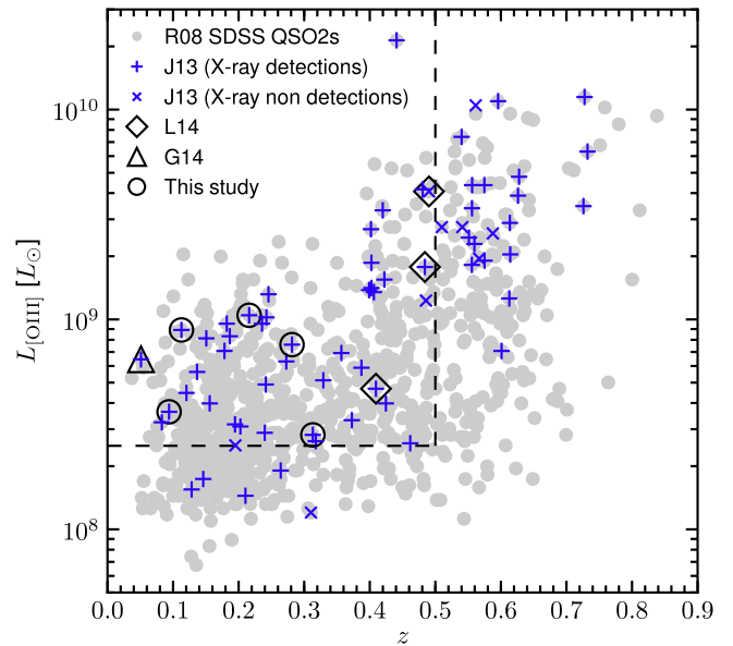
Figure 1. Observed (i.e., extinction-uncorrected) [\text{O III}]\lambda 5007 line luminosity ( L_{[\text{O III}]} ) vs. redshift ( z ). The R08 sample of SDSS-QSO2s is shown as gray dots. The J13 sample of Chandra - and XMM-Newton -observed objects is indicated in blue, with “+” and “x” symbols indicating <10 \text{ keV} detections and non-detections, respectively (according to X-ray analyses in J13 and Vignali et al. 2006, 2010). The dashed lines mark the parameter space used in this work ( z < 0.5 and L_{[\text{O III}]} > 2.5 \times 10^8 L_{\odot} ), for which the J13 sample is broadly representative of the R08 sample. Our NuSTAR -observed subsample of candidate CTQSO2s is highlighted by black points, with circles marking the five recently observed objects presented in this study, diamonds marking the three z \approx 0.4 – 0.5 objects presented in L14, and the triangle marking the low redshift ( z = 0.05 ) object presented in G14.
