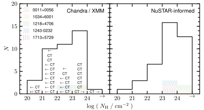
Figure 13. N_H distribution of SDSS-selected QSO2s at z < 0.5 , constructed using only direct constraints from X-ray spectral analyses. The five NuSTAR -observed objects with enough > 10 keV counts for X-ray spectral analyses are marked by the hatched regions. Left panel: a measurement of the N_H distribution from existing soft X-ray ( < 10 keV) Chandra and XMM-Newton constraints. CT candidates, identified as such in J13 and LaMassa et al. (2014) primarily using the indirect X-ray:[O III] luminosity ratio diagnostic, are labeled as “CT.” Sources with upper/lower limits in N_H are marked with arrows. Right panel: prediction for the true N_H distribution of SDSS-QSO2s based on the results of this broad-band NuSTAR plus soft X-ray study; see Section 5.2.
