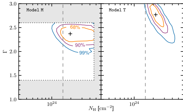
FIG. 8.— Intrinsic photon index ( \Gamma ) versus (line-of-sight) column density ( N_{\text{H}} ) confidence contours for SDSS J1218+4706. The contours outline the 68%, 90% and 99% confidence regions, and the best-fit value is marked by a black cross. We show results for two models (Model M and Model T; left and right panels). The individual models are detailed in Section 4.1.1. The gray shaded region indicates the parameter ranges for which Model M is not valid. The best-fit column densities are CT ( N_{\text{H}} > 1.5 \times 10^{24} cm ^{-2} ), and the 90% CL lower N_{\text{H}} limits lie just below and just above the CT threshold (gray dashed line) for Model M and Model T, respectively.
