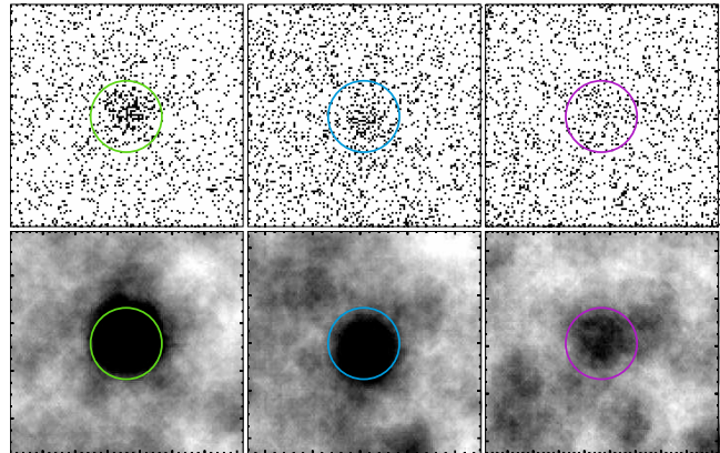
FIG. 3.— NuSTAR 8–24 keV images for the three objects detected in this energy band: SDSS J1218+4706, 1243-0232 and 1713+5729 (left to right, respectively). Top row: unsmoothed photon images. Bottom row: images smoothed with a top hat function of radius 14 pixels, corresponding to 34''.5 (for aesthetic purposes only). The 45'' radius source apertures are shown, centered on the SDSS positions. The major tickmarks indicate 1 arcmin offsets in right ascension (R.A.; horizontal axis) and declination (Decl.; vertical axis).
