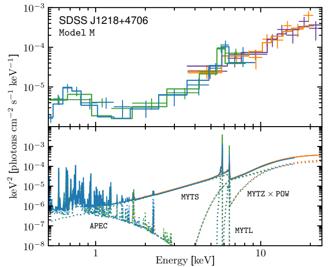
FIG. 7.— Unfolded NuSTAR plus XMM-Newton spectrum, in E F_E units, for SDSS J1218+4706. The data are shown in the upper panel, grouped to a minimum significance of 2\sigma per bin for visual purposes. The NuSTAR FPMA and FPMB data are shown in purple and orange, respectively. The MOS (obsID 0203270201) and PN (obsID 0400560301) data are shown in green and blue, respectively. The best-fit MYTORUS-based model (Model M; described in Section 4.1.1) is shown binned to match the data (solid lines, upper panel) and in full detail (lower panel).
