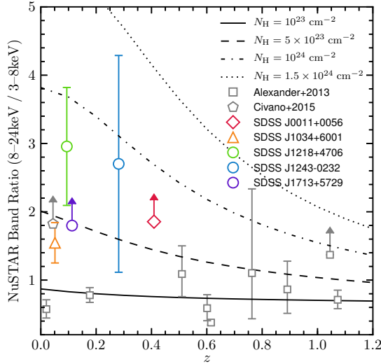
FIG. 10.— NuSTAR band ratio ( BR_{\text{Nu}} ) versus z . The circles, the diamond and the triangle indicate the candidate CTQSO2s presented in this work, L14 and G14, respectively, which are detected at 8–24 keV; 90% CL error bars and limits are shown. For comparison, gray squares show the first 10 AGNs detected in the NuSTAR serendipitous survey (Alexander et al. 2013); 68% CL error bars are shown. The gray pentagon marks a CT AGN identified with NuSTAR in the COSMOS field (F Civano et al., submitted); a 90% CL lower limit is shown. The tracks show model predictions for BR_{\text{Nu}} for four absorbing column densities in the range N_{\text{H}} = (0.1\text{--}1.5) \times 10^{24} \text{ cm}^{-2} . The BR_{\text{Nu}} constraints for SDSS J1218+4706, 1243–0232 and 1713+5729 are higher than that of the confirmed CTQSO2 SDSS J1034+6001, and suggest large absorbing columns.
