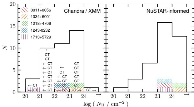
FIG. 13.— The N_{\text{H}} distribution of SDSS-selected QSO2s at z < 0.5 , constructed using only direct constraints from X-ray spectral analyses. The five NuSTAR -observed objects with enough > 10 keV counts for X-ray spectral analyses are marked by the hatched regions. Left panel: a measurement of the N_{\text{H}} distribution from existing soft X-ray ( < 10 keV) Chandra and XMM-Newton constraints. CT candidates, identified as such in J13 and LaMassa et al. (2014) primarily using the indirect X-ray:[O III] luminosity ratio diagnostic, are labeled as “CT”. Sources with upper/lower limits in N_{\text{H}} are marked with arrows. Right panel: Prediction for the true N_{\text{H}} distribution of SDSS-QSO2s, based on the results of this broad-band NuSTAR plus soft X-ray study; see Section 5.2.
