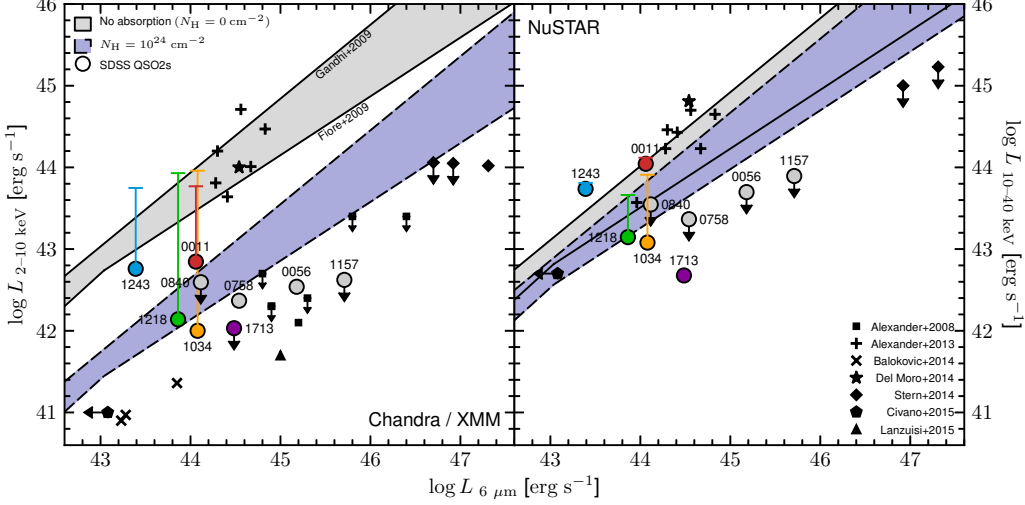
FIG. 11.— Observed (i.e., uncorrected for absorption) X-ray luminosity for the rest-frame 2–10 keV and 10–40 keV bands (left and right hand panels, respectively) versus rest-frame 6 \mu\text{m} luminosity (in \nu L_\nu units). The circles indicate the NuSTAR -observed SDSS-selected candidate CTQSO2s presented in this work, L14, and G14 ( z = 0.05\text{--}0.49 ); colored circles mark the NuSTAR -detected sources. The X-ray luminosities for the candidate CTQSO2s are taken from best-fitting spectral models where possible. Otherwise, they have been determined from photometry, assuming an unabsorbed power law model with \Gamma = 0.3 (as described in Section 3.1). For the three L14 objects (SDSS J0011+0056, 0056+0032 and 1157+6003), the values have been adjusted for consistency with this work. Other NuSTAR -observed objects are shown, including: NuSTAR extragalactic survey AGNs (+ symbols; z = 0.02\text{--}2.92 ; Alexander et al. 2013), three CT Seyfert 2 AGNs (x symbols; z \approx 0.01 ; Baloković et al. 2014), a heavily obscured quasar identified in the ECDFS field (star; z \approx 2 ; Del Moro et al. 2014), three luminous and heavily obscured WISE -selected AGNs (diamonds; z \approx 2 ; Stern et al. 2014), and a CT AGN identified in the COSMOS field (pentagon; z = 0.044 ; F Civano et al., submitted). For the latter object, we show an upper limit in L_{6\mu\text{m}} , since we have assumed that the mid-IR emission is AGN-dominated. Additionally, for the 2–10 keV band we compare with sources studied at < 10 keV with Chandra or XMM-Newton : the candidate CT quasars presented in Alexander et al. (2008; squares; z \approx 2 ), and a candidate heavily CT AGN identified in the COSMOS field (triangle; z = 0.35 ; Lanzuisi et al. 2015b). For four of the NuSTAR -observed candidate CTQSO2s, vertical lines indicate the intrinsic (i.e., corrected for absorption) X-ray luminosities obtained from X-ray spectral analyses. We compare all of the data with two intrinsic relations for the 2–10 keV band (solid black lines), those of Fiore et al. (2009) and Gandhi et al. (2009). Following L14 and Stern et al. (2014), the relations have been extrapolated to 10–40 keV assuming \Gamma = 1.8 , and the dashed lines show the effect of absorption by N_{\text{H}} = 10^{24} \text{ cm}^{-2} gas. The different X-ray:mid-IR ratios for the Fiore et al. (2009) and Gandhi et al. (2009) relations means that the former provides a more conservative estimate of the CT absorption threshold. The majority of the NuSTAR -observed candidate CTQSO2s have low X-ray:mid-IR ratios, suggesting CT levels of photoelectric absorption.
