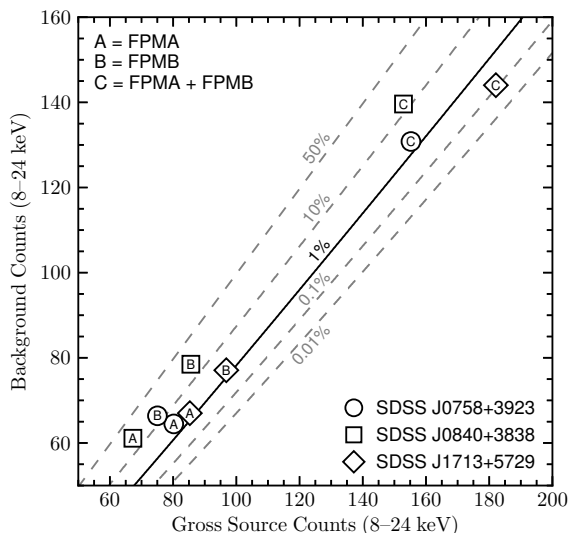
FIG. 2.— NuSTAR photometry at 8–24 keV for the faintest three sources, SDSS J0758+3923, 0840+3838 and 1713+5729 (circles, squares and diamonds, respectively). Gross source counts and background counts (scaled to the source aperture) are shown. The dashed lines indicate tracks of constant Poisson no-source probability (a good approximation of P_B , given the large background counts considered here; Weisskopf et al. 2007). The solid black line shows our adopted detection threshold of P_B = 1\% . Only SDSS J1713+5729 is detected: while it is not detected in the individual FPMs, the increased sensitivity in FPMA+B (i.e., the combined FPMA+FPMB data) results in a significant detection, with P_B = 0.22\% .
