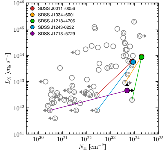
FIG. 12.— Intrinsic (i.e., absorption-corrected) rest-frame 2–10 keV luminosity ( L_{2-10 \text{ keV}}^{\text{in}} , or L_{\text{X}} ) versus N_{\text{H}} for SDSS-selected QSO2s, as measured from X-ray spectral analyses. The grey open circles show the constraints in the literature, all directly measured from X-ray spectral fitting at soft X-ray energies ( < 10 \text{ keV} ; J13; LaMassa et al. 2014). Sources with evidence for being CT, primarily based on the indirect X-ray:[O III] luminosity ratio diagnostic, are marked with a “C”. The colored circles show our constraints for the five NuSTAR -observed candidate CTQSO2s detected at high energies ( > 10 \text{ keV} ), from the broad-band NuSTAR plus soft X-ray spectral analyses presented in this study, L14, and G14. The colored lines indicate the significant increase in both L_{\text{X}} and N_{\text{H}} for these five objects between the soft X-ray constraints in the literature and the NuSTAR plus soft X-ray studies. We note that for SDSS J1243–0232 the increase in L_{\text{X}} shown (blue line) may be an overestimate. a
