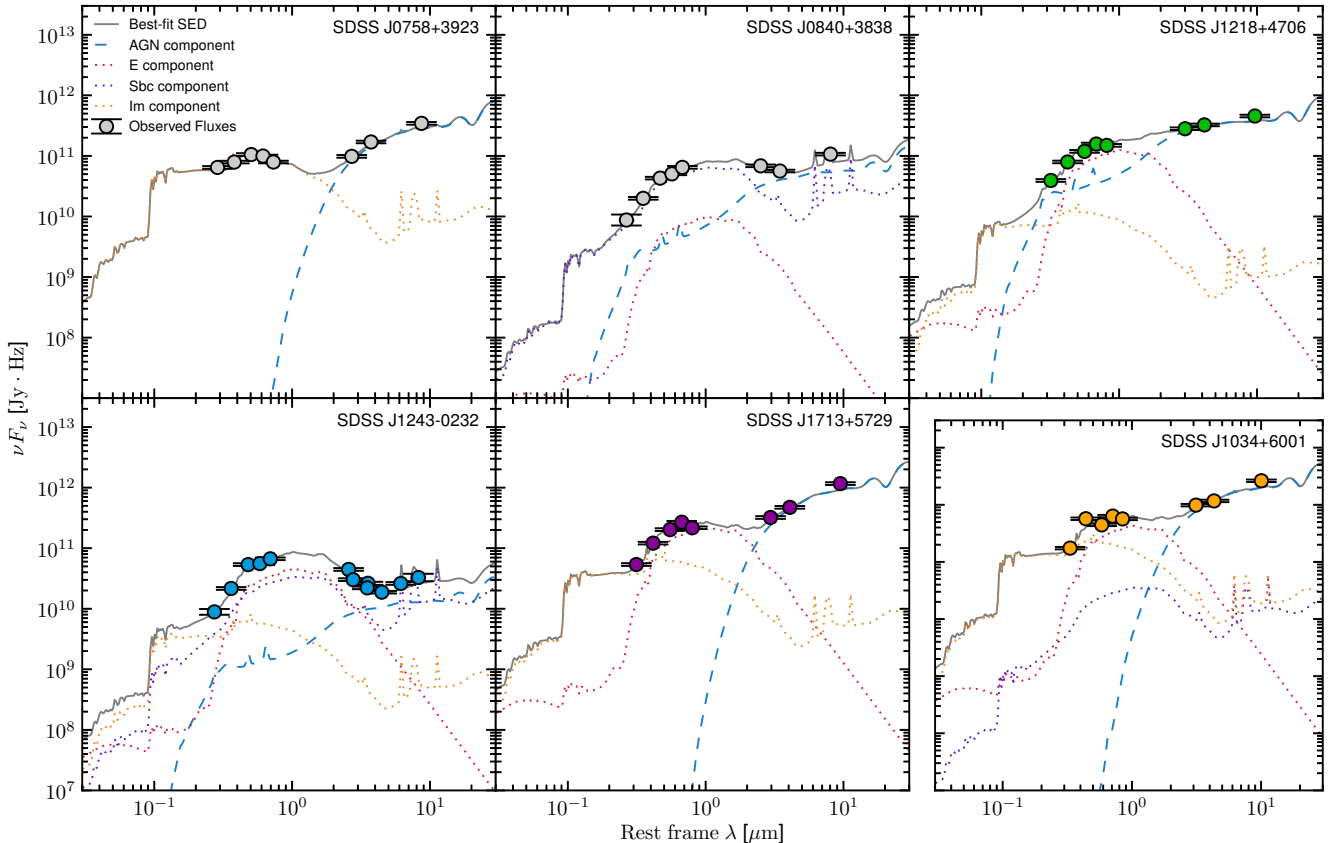
FIG. 4.— Near-UV to mid-IR spectral energy distributions (SEDs) for the five candidate CTQSO2s presented in this work, and the one (SDSS J1034+6001) presented in G14. AGN (blue dashed curve) and galaxy (dotted curves) templates were combined in the best-fit modeling of the photometric data (colored circles for the sources detected at 8–24 keV with NuSTAR , and grey circles for the 8–24 keV non-detections), following Assef et al. (2008, 2010, 2013). The three galaxy templates correspond to an old stellar population (“elliptical” or E; red), ongoing star formation (“spiral” or Sbc; purple), and a starburst population (“irregular” or Im; orange). The gray curve shows the combined model solution. The systems are all AGN-dominated in the mid-IR waveband based on this analysis, except for SDSS J1243–0232, which has comparable contributions from the AGN and the host galaxy; see Table 3.
