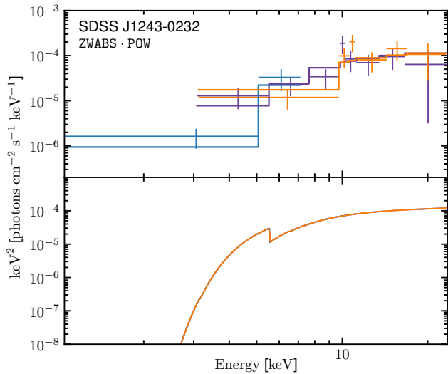
FIG. 9.— Unfolded NuSTAR (purple and orange for FPMA and FPMB, respectively) plus Chandra (blue) X-ray spectrum for SDSS J1243–0232. The best-fit absorbed power law (ZWABS · POW) model is shown. The panel layout, units and data binning follow that of Figure 7.
