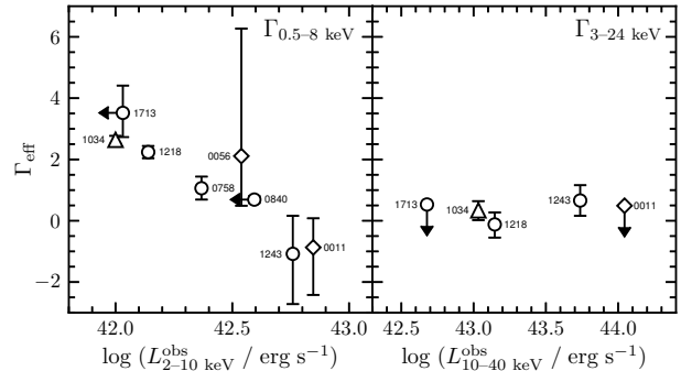
FIG. 6.— Observed X-ray properties of the NuSTAR -observed candidate CTQSO2 sample. Left panel: properties measured at low energies with Chandra and XMM-Newton . Right panel: properties measured at high energies with NuSTAR . Only detected sources are shown. Circles, diamonds and the triangle indicate the objects presented in this work, L14, and G14, respectively. The effective photon index ( \Gamma_{\text{eff}} ), which provides a basic description of the overall X-ray spectral shape, was obtained by fitting an unabsorbed power law model to the data for each source. The rest-frame X-ray luminosities ( L_{\text{X}}^{\text{obs}} ; bottom axis) are observed values, i.e. uncorrected for absorption. For the five objects presented in this paper, the luminosities correspond to those in Table 3. For the L14 and G14 objects the luminosities have been calculated using the same methodology: spectral modeling where possible, or photometry following the procedure outlined in Section 3.1. In the cases of the X-ray faint sources SDSS J0011+0056 and SDSS J1713+5729, the \Gamma_{\text{eff}} for 3–24 keV was estimated from the NuSTAR band ratio ( \text{BR}_{\text{Nu}} ; see Section 4.2).
