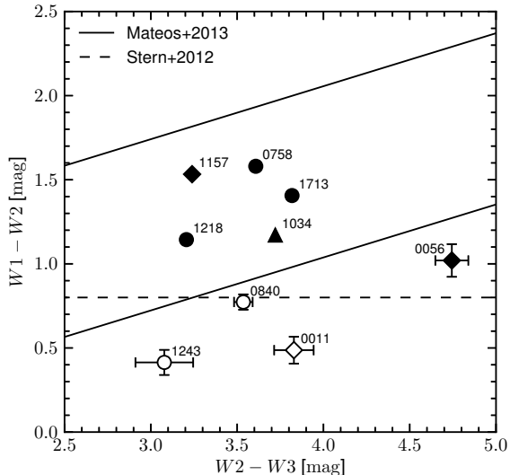
FIG. 5.— WISE color-color diagram for the NuSTAR -observed SDSS-selected candidate CTQSO2s from this study (circles), G14 (triangle) and L14 (diamonds). We compare with the AGN color cut of Stern et al. (2012; W1 - W2 \geq 0.8 ) and the AGN ‘wedge’ of Mateos et al. (2013). The filled and empty symbols mark sources which are strongly AGN-dominated ( \hat{a} \gtrsim 0.9 ) and less AGN-dominated ( \hat{a} \lesssim 0.6 ), respectively, at mid-IR wavelengths according to our SED modeling. For the five objects that lie within the AGN wedge, the error bars are smaller than the symbols.
