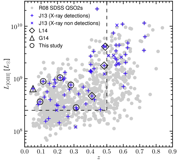
FIG. 1.— Observed (i.e., extinction-uncorrected) [O III] \lambda 5007 line luminosity ( L_{[\text{O III}]} ) versus redshift ( z ). The R08 sample of SDSS-QSO2s is shown as grey dots. The J13 sample of Chandra - and XMM-Newton -observed objects is indicated in blue, with ‘+’ and ‘x’ symbols indicating < 10 \text{ keV} detections and non-detections, respectively (according to X-ray analyses in J13 and Vignali et al. 2006, 2010). The dashed lines mark out the parameter space used in this work ( z < 0.5 and L_{[\text{O III}]} > 2.5 \times 10^8 L_{\odot} ), for which the J13 sample is broadly representative of the R08 sample. Our NuSTAR -observed subsample of candidate CTQSO2s is highlighted by black points, with circles marking the five recently observed objects presented in this study, diamonds marking the three z \approx 0.4\text{--}0.5 objects presented in L14, and the triangle marking the low redshift ( z = 0.05 ) object presented in G14.
