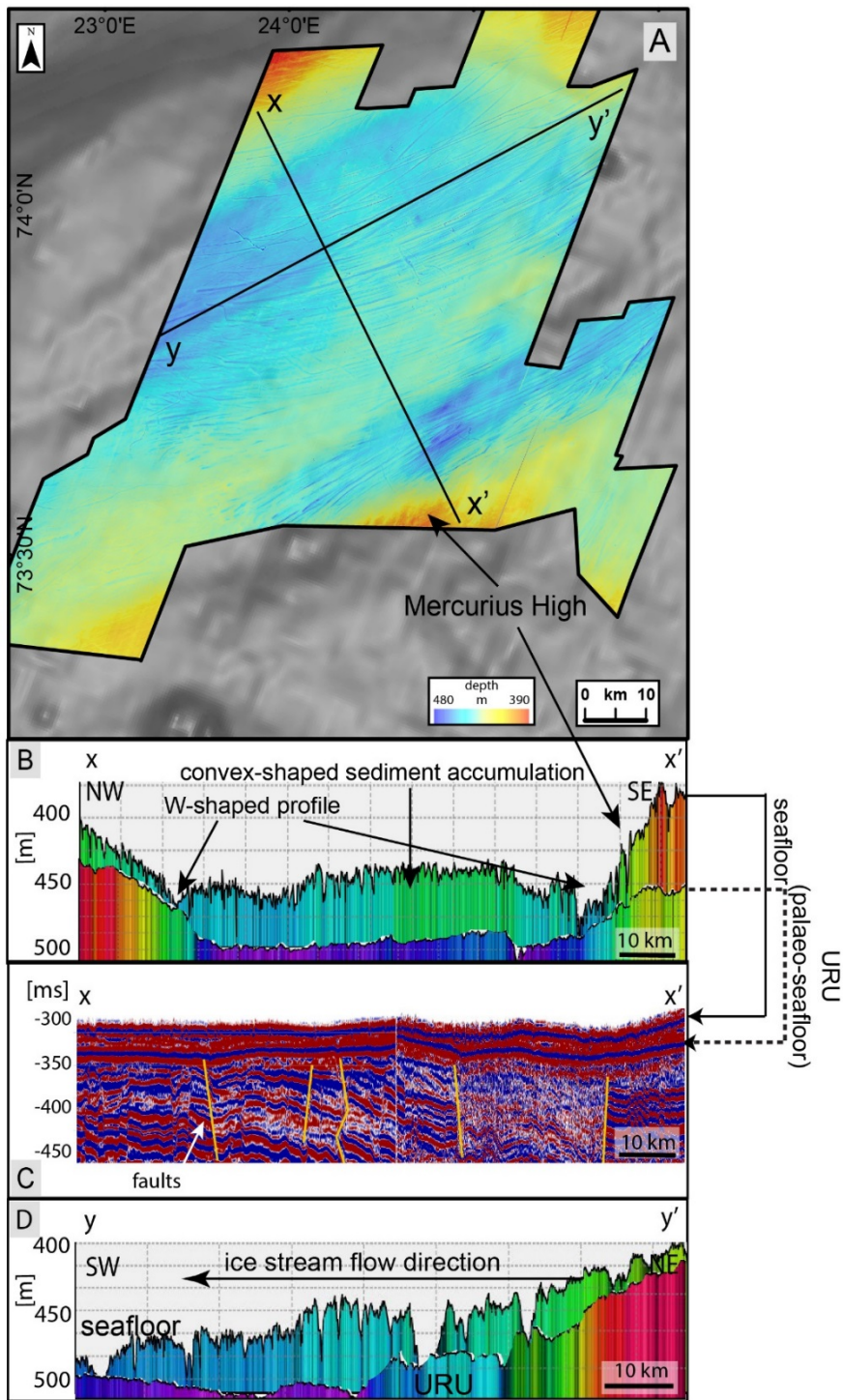
Figure 3. (A) Large-scale bathymetry of the modern seafloor in central Bjørnøyrenna. (B) Topography of the seafloor and the URU shows two overdeepenings on both surfaces and a convex-shaped sediment accumulation in the central part of the seafloor (colour-scaled to elevation). (C) Seismic profile indicating the location of the seafloor and the URU, as well as
