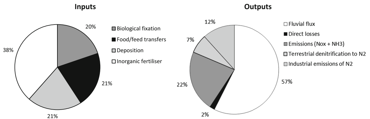
Fig. 5 Proportions of N inputs and outputs projected for 2020
