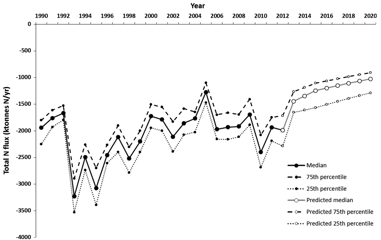
Fig. 4 The time series of the stochastic total N budget between 1990 and 2012 with the projection to 2020. NB by the convention of the study a negative flux is a source from the UK
