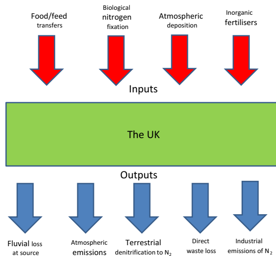
Fig. 1 Schematic representation of the total N budget for the UK
