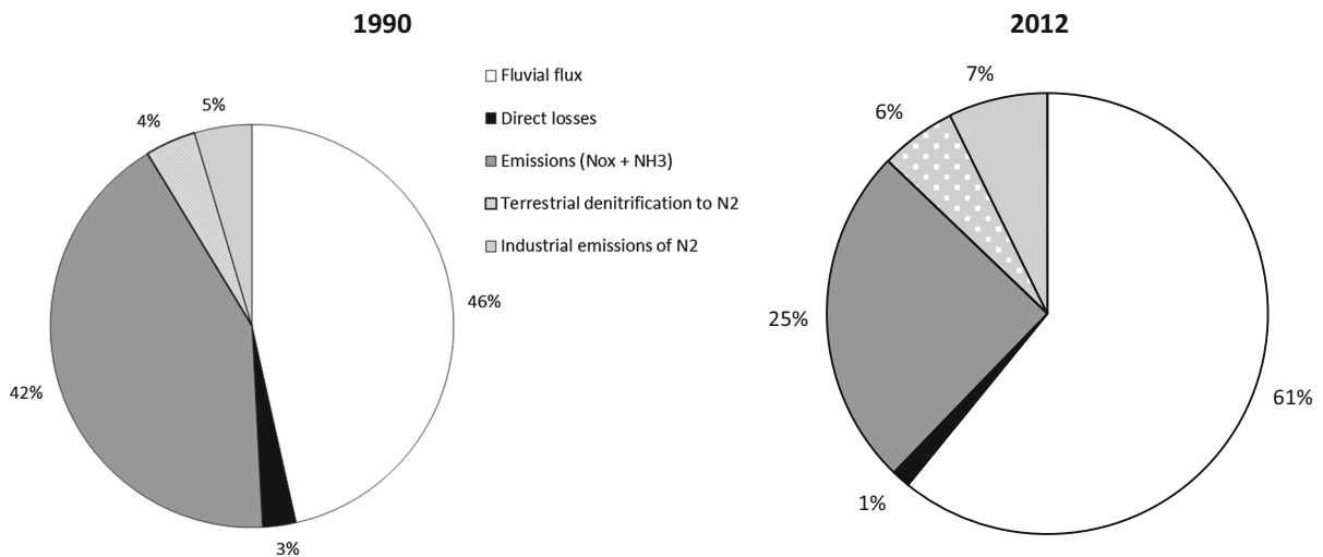
Fig. 3 Proportions of N outputs in 1990 and 2012
