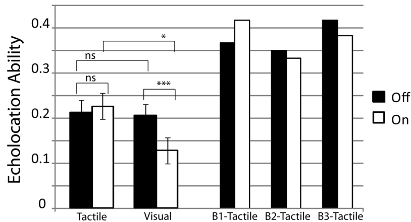
Figure 3. Visual sensory stimulation (but not tactile sensory stimulation) impairs people's ability to echolocate. Left hand side: Performance of sighted participants ( N = 44 ). Tactile– Tactile sensory stimulation. Visual– Visual sensory stimulation. Bars indicate averages across participants, error bars indicate standard errors across participants. Right hand side: Performance of blind echo-expert participants B1–B3 (narrow bars), who only took part in tactile conditions. * p < 0.05 ; ** p < 0.01 ; *** p < 0.001 ; ns = non-significant
