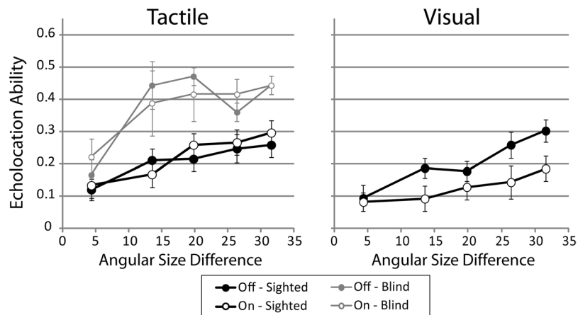
Figure 2. Visual sensory stimulation (but not tactile sensory stimulation) impairs people’s ability to echolocate. Data for sighted and blind participants are plotted in black and grey lines, respectively. Tactile– Tactile sensory stimulation. Visual– Visual sensory stimulation. Filled and open symbols denote stimulation ‘off’ and ‘on’ respectively. Data are plotted as a function of the angular size difference between the reference and comparison disks. The reference disk was 25.4 cm in diameter. The five comparison disks had diameters of 5.1 cm, 9 cm, 13.5 cm, 17.5 cm and 22.9 cm, resulting in angular size differences between the reference and the comparison disks of approximately 31.6°, 26.4°, 19.8°, 13.5° and 4.3°. Symbols are means and error bars are standard errors across participants.
