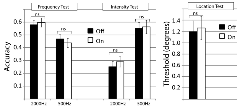
Figure 4. Visual sensory stimulation has no effect on people's ability to detect changes in sound frequency, intensity or location. Performance of sighted participants in auditory control experiments: Frequency ( n = 26 ) and Intensity ( n = 25 ) discrimination conducted at both 2000 and 500 Hz, and Location discrimination ( n = 22 ). Bars indicate averages across participants; error bars indicate standard errors across participants. * p < 0.05 ; ** p < 0.01 ; *** p < 0.001 ; ns = non-significant
