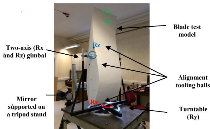
Figure 9 – Blade test model setup within the laboratory. The turntable and gimbal allowed rotation in Rx, Ry and Rz. The mirror provided a line of sight to the underside of the blade and the tooling balls allowed quick alignment to the CAD model
