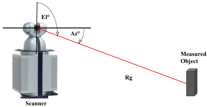
Figure 4 – CLR scanner showing azimuth, elevation and range measurement capabilities
