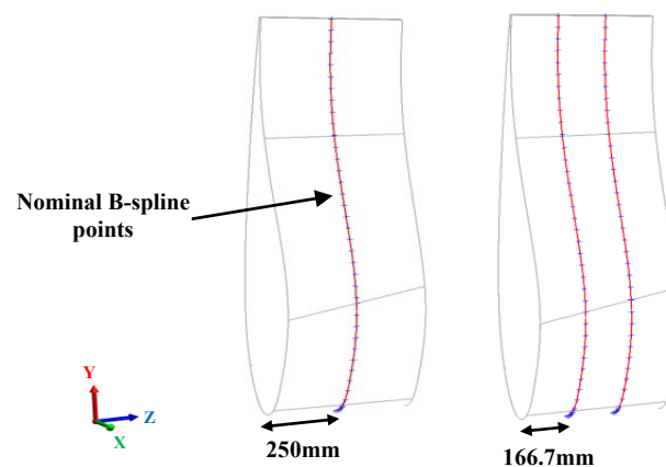
Figure 12 – Left, the single B-spline arrangements (Experiment 1), 250mm from the root end of the cross-section. Right, the double B-spline arrangement (Experiment 2), evenly distributed 166.7mm from the root end
