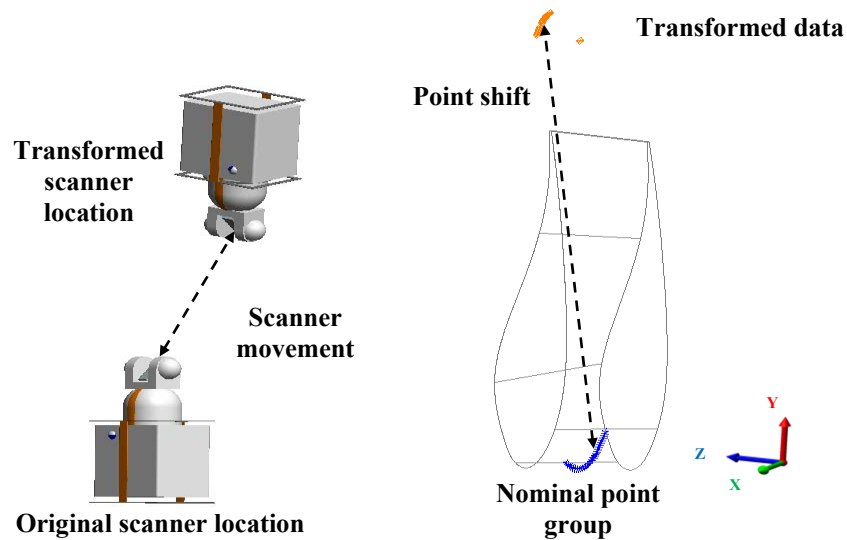
Figure 13 –Huge point shifts and scanner movements were found when implementing a 20^\circ Rz offset; the offset was deemed inappropriate
