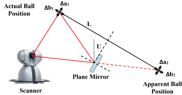
Figure 6 – Tooling ball alignment, needed in order to create a mirror plane in SA [20]
