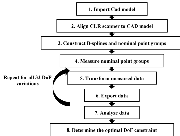
Figure 10 – Experimental procedure used to measure and analyze each constrained DoF variation to establish the optimal data alignment solution
