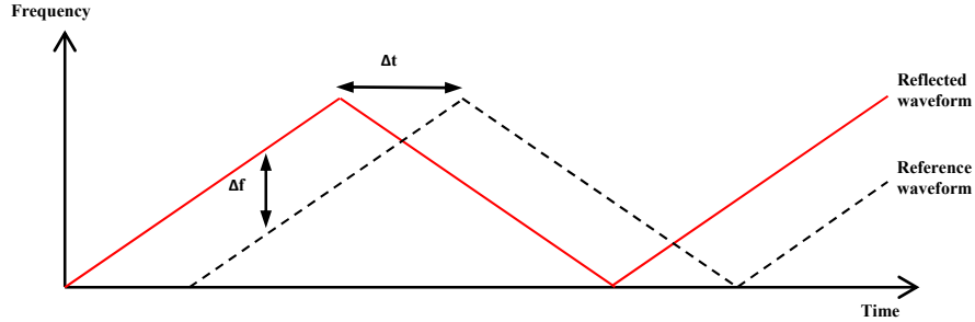
Figure 3 – Comparison of the reflected laser signal with the controlled reference signal. \Delta f can be calculated due to a base frequency 200THz and a fixed wavelength of 1500nm [8]
