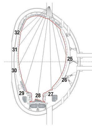
FIG. 2. Lines of sight of bolometer system, installed on JET
