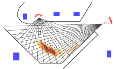
FIG. 1. Illustration of the lines of sight of the SXD bolometer system on MAST-U
