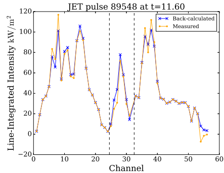
FIG. 4. Comparison of measured intensity and expected intensity, back calculated from the emissivity profile. The channels belonging to the new system (KB5F) are inside the dashed lines. The vertical channels of the existing system are on the left of the plot, the horizontal channels on the right.
