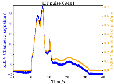
FIG. 3. Comparison of channel 3 of the existing JET system (KB5V, dark blue) and channel 26 of the new system (KB5F, light orange). Note that the zero point on the KB5F axis has been shifted to avoid the two traces overlapping too closely.
