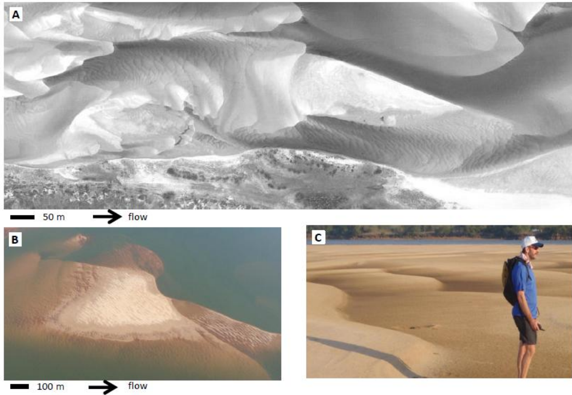
Figure 4. Examples of abandoned dunes. A) Aerial photographs of abandoned dune fields in areas sheltered by bars, South Saskatchewan River, Canada. B) and C) abandoned dunes on mid-channel bars, Río Paraná, Argentina.
