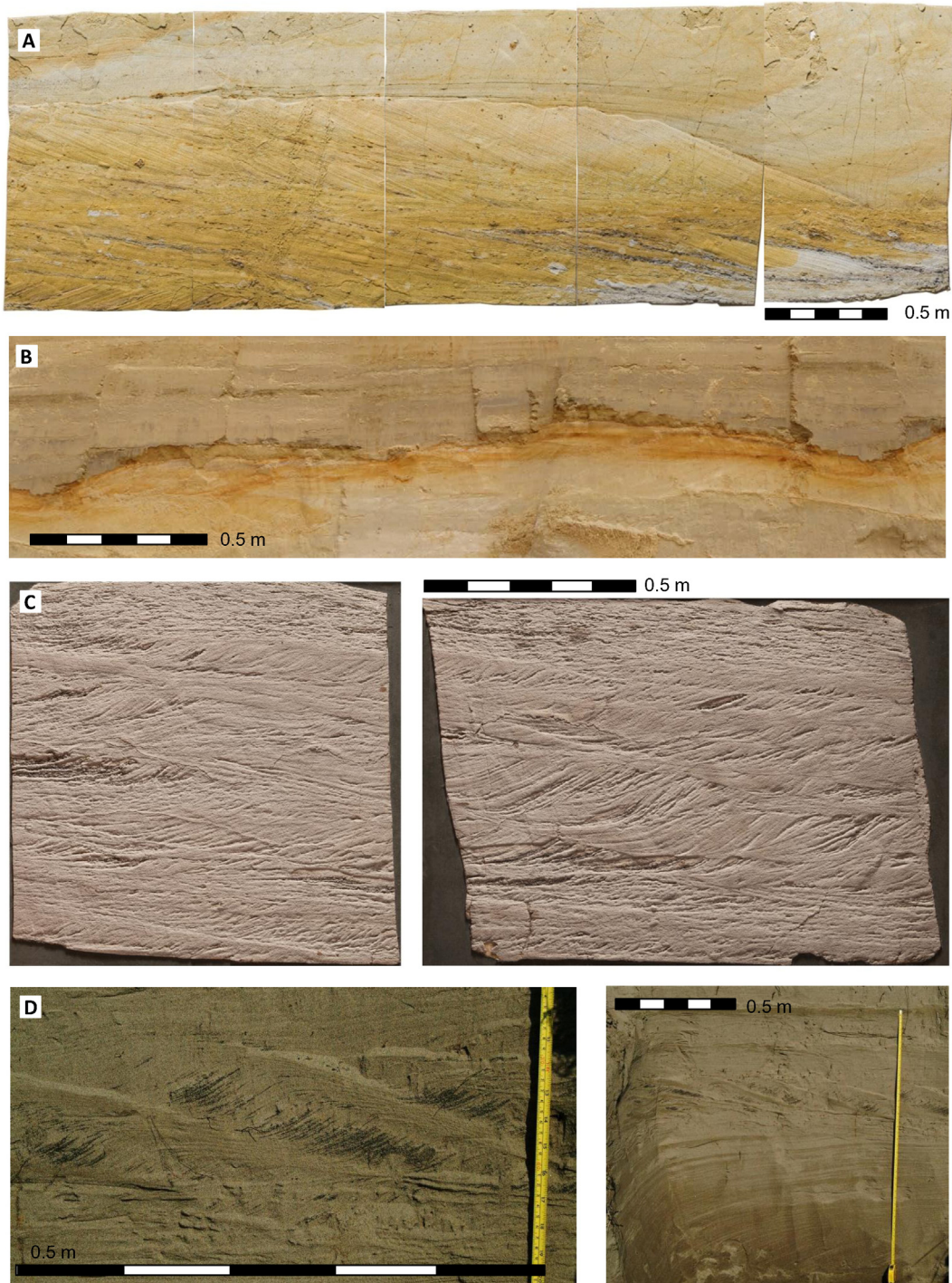
Fig. 5. Examples of form-sets. A) Lacquer peels of a preserved dune deposits within a river channel that are buried underneath turbidite deposits that originated from a channel bank breach failure (see Martinius and Van den Berg, 2011 ; their Fig. 3.5.8). B) Form-sets preserved under fine-grained deposits in an Oxbow lake that was abandoned suddenly. Flow right to left. Mid-Pleistocene deposits near Brügggen, Germany. Height of the dunes is approximately 0.1 m. C) Lacquer peels of climbing dune sets from lower Pliocene deposits, Tagebau Hambach, Germany. Note that the topsets cannot be traced consistently through-out the profile, which indicates variations between stoss-erosional and stoss-depositional styles of dune climbing. The two peels are adjacent to each other and represent a 45° corner, which implies that the actual inclinations of the strata and bedding are steeper than apparent in these photographs. D) Small, approximately 0.1 m high, stoss-depositional climbing dunes preserved in medium sand deposits (approx. 250 \mu\text{m} ) of the braided South Saskatchewan River, Canada. Flow right to left, close-up section about 1 m long. Black grains are organic particles deposited on the dune lee slopes. Note the climbing dunes lie above a series of low-angle, bar-scale, downstream-dipping strata (lower 0.5 m of the section, right photo). These low-angle strata represent sedimentation on the downstream side of a bar, with the climbing dunes thus developing in this region of decelerating flow with locally enhanced vertical rates of sedimentation.
