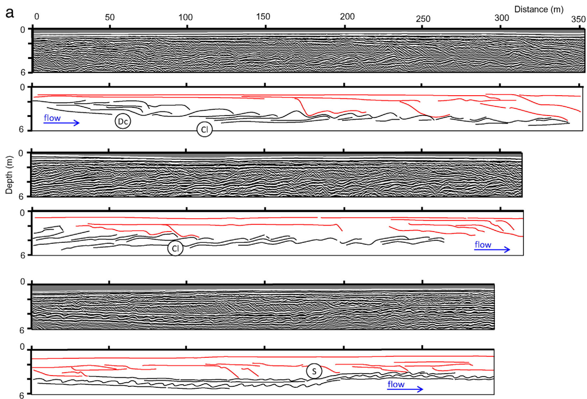
Fig. 2. Examples of form-sets in GPR images from the Río Paraná, Argentina, with interpretative line diagrams below each GPR panel. All profiles are oriented in the downstream direction. The red lines indicate the overlying bar deposits, while the black lines indicate bar trough deposits that include the dune form-sets. Cl denotes climbing sets, formed in cases where dune migration was low compared to the vertical aggradation. Dc denotes down-climbing sets formed in cases where dunes migrate down a larger-scale lee slope. R denotes reactivated form-sets, and S denotes superimposed dune fields, both of which imply multiple periods of activity of the dune form-sets.
