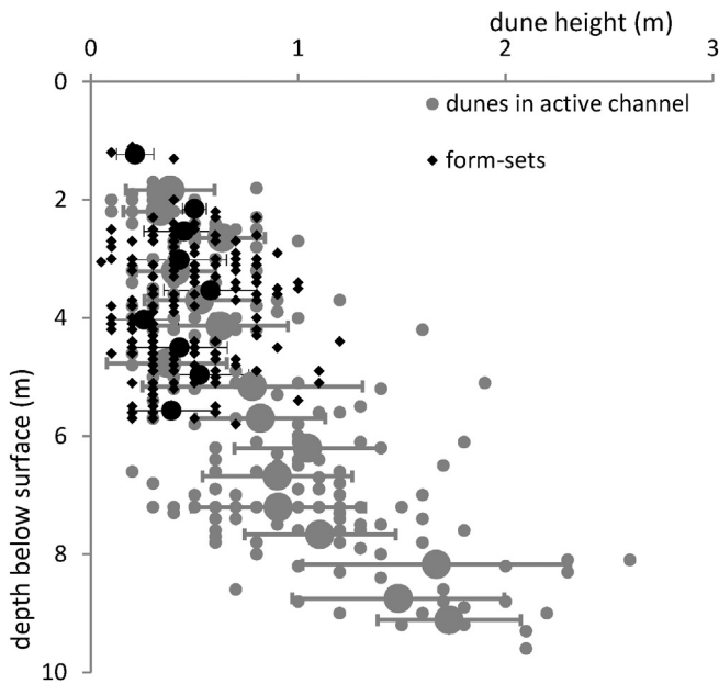
Fig. 3. A comparison of the heights of active dunes (Río Paraná near Corrientes) plotted against flow depth relative to the water surface during a near-average flow, and thicknesses of all form-sets identified in the GPR images with respect to the height of the bar surface. Error bars are standard deviation around means calculated per half meter depth interval.
