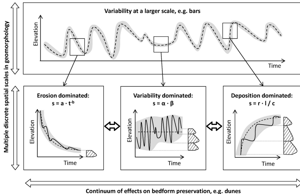
Fig. 6. Three paradigms for preservation in a sedimentary system (delimited in time and space) that experiences variability in erosional scour that is: dominance of erosion of a deposit (e.g. Gilluly, 1969), dominance of variability as a control on thickness distributions (e.g. Paola and Borgman, 1991), and dominance of deposition (e.g. Sorby, 1859; Allen, 1970). Equations are presented as examples of different shapes of trends described in literature, but are likely to vary between locations, times, and geomorphic settings. s is the thickness of the preserved layer (m), a and b are constants that describe the exponential loss of sedimentary strata over time, t is time, \gamma is a constant that describes the relation between the bedform height and trough scour depth, and \beta represents the variability in bedform height, L is the bedform length (m), r is the flux of sediment to the bed ( m s^{-1} ), and c is the celerity of the bedform along the bed ( m s^{-1} ).
