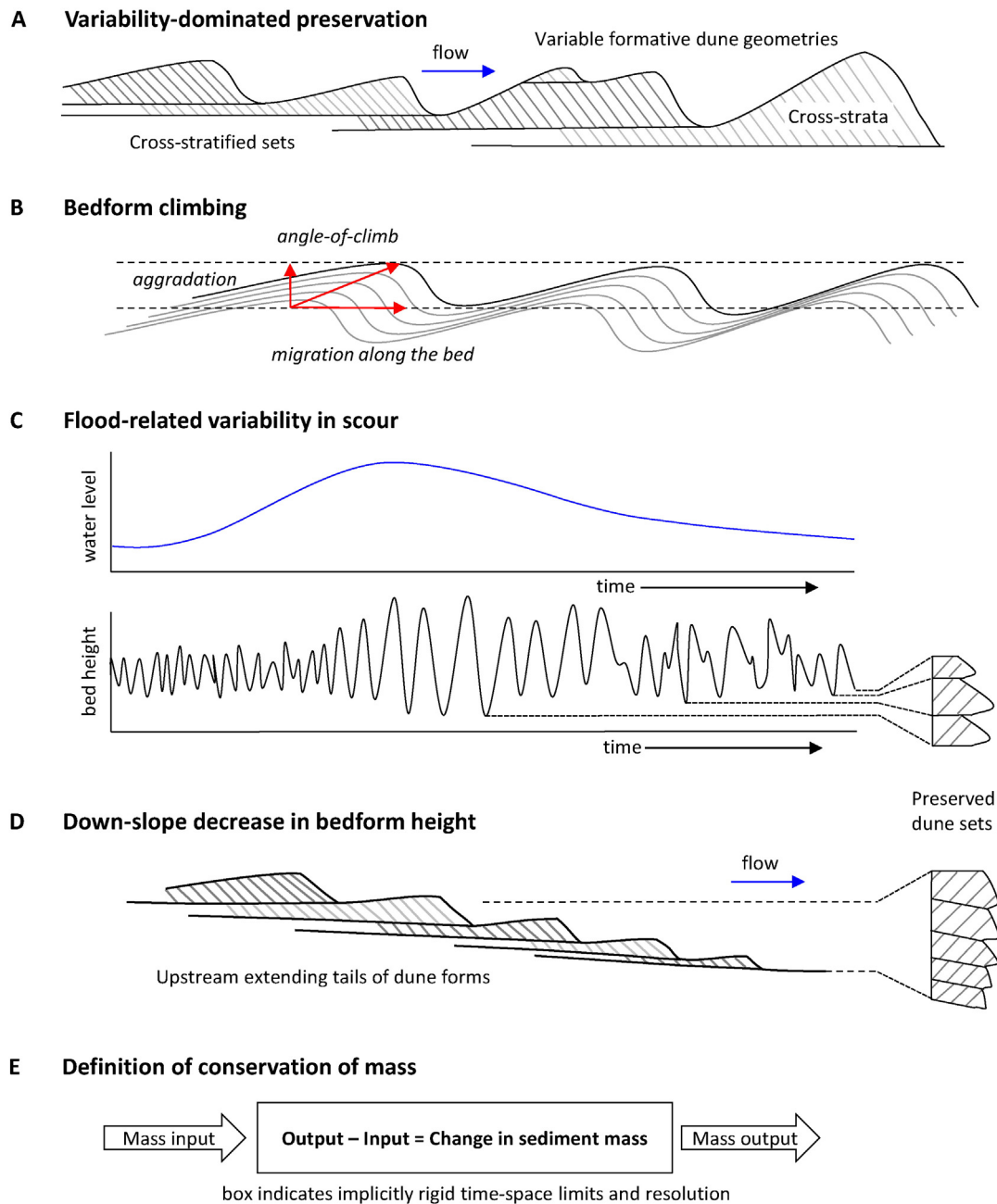
Fig. 1. Illustrations of fundamental processes that control the preservation of dune sets: A) the role of bedform scour variability; B) the role of aggradation as a control on preserved set thickness; C) dune development during a flood wave and its effect on dune preservation (after Kleinhans, 2002); D) decrease in bedform height (and set thickness) as dunes migrate down larger-scale lee slopes (e.g. Rubin and Hunter, 1982); E) schematic diagram of conservation of mass in bedform migration.
