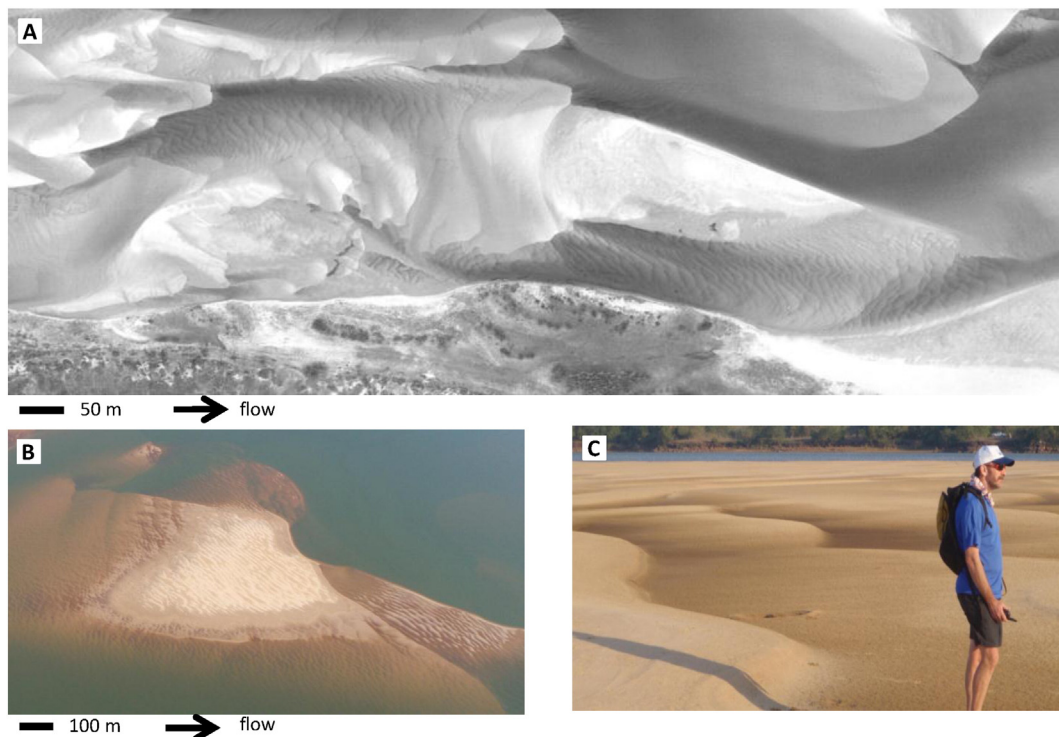
Fig. 4. Examples of abandoned dunes. A) Aerial photographs of abandoned dune fields in areas sheltered by bars, South Saskatchewan River, Canada. B and C) Abandoned dunes on mid-channel bars, Río Paraná, Argentina.
