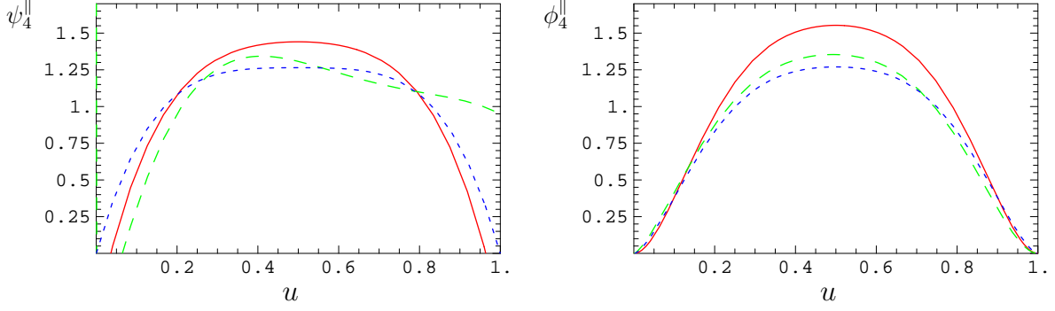
Figure 1: [Colour online] Left panel: \psi_4^{\parallel} , (3.26), as a function of u for the central value of the hadronic parameters, for \mu = 1 \text{ GeV} . Solid [red] line: \psi_{4;\rho}^{\parallel} , dashed [green]: \psi_{4;K^*}^{\parallel} , short-dashed [blue]: \psi_{4;\phi}^{\parallel} . Right panel: same for \phi_4^{\parallel} , (3.28).
