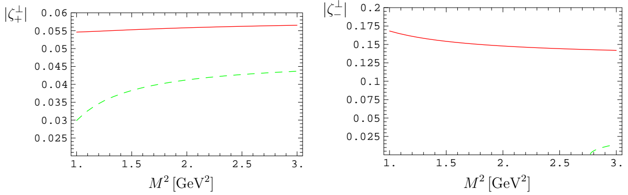
Figure F: [Colour online] |\zeta_+^\perp|_D (left) and |\zeta_-^\perp|_D (right), for the \rho , from the sum rules (C.15) and (C.17). Solid [red] curves: PP ( s_0 = 1.2 \text{ GeV}^2 ), dashed [green] curves: MP sum rules ( s_0 = 1.0 \text{ GeV}^2 ).
