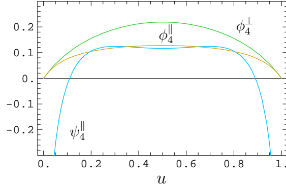
Figure 3: [Colour online] Renormalon-model predictions for \phi_{4;\rho}^{\parallel,\perp} and \psi_{4;\rho}^{\parallel} ; \psi_{4;\rho}^{\perp} = 0 in the renormalon model.
