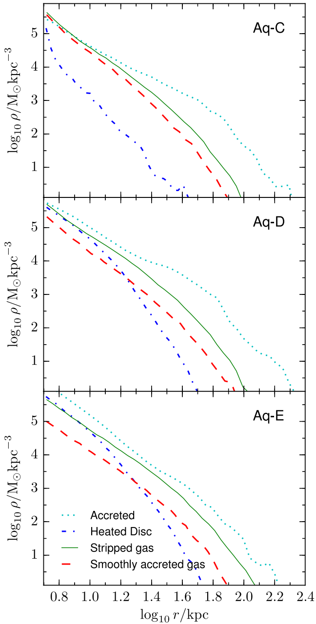
Figure 4. Spherically averaged density profiles of halo stars in the accreted and three in situ components for Aq-C (top), Aq-D (centre) and Aq-E (bottom).
