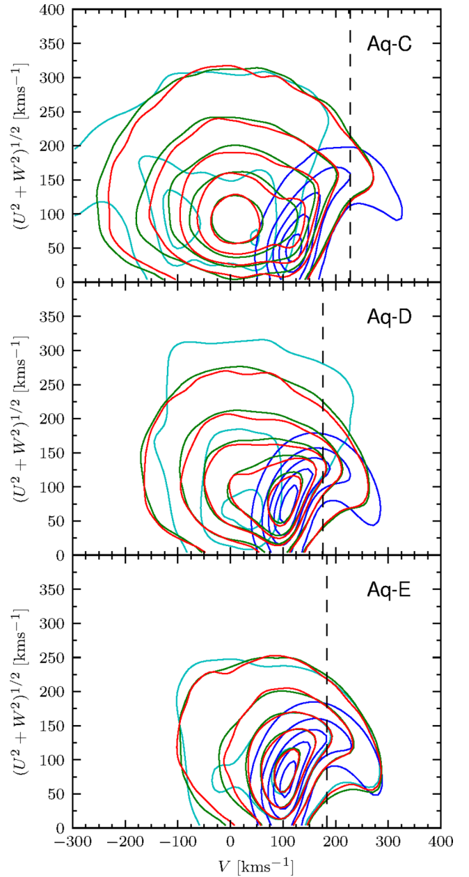
Figure 5. Toomre diagrams of the whole stellar halo. For stripped-gas, smooth-gas and heated disc in situ halo stars (red, green and dark blue, respectively), contours mark the regions enclosing 10, 30, 50, 70 and 90 per cent of the stellar mass. For the accreted halo (cyan), only 10, 50 and 90 per cent levels are shown. The dashed vertical line marks the rotation velocity of the disc at 8 kpc.
