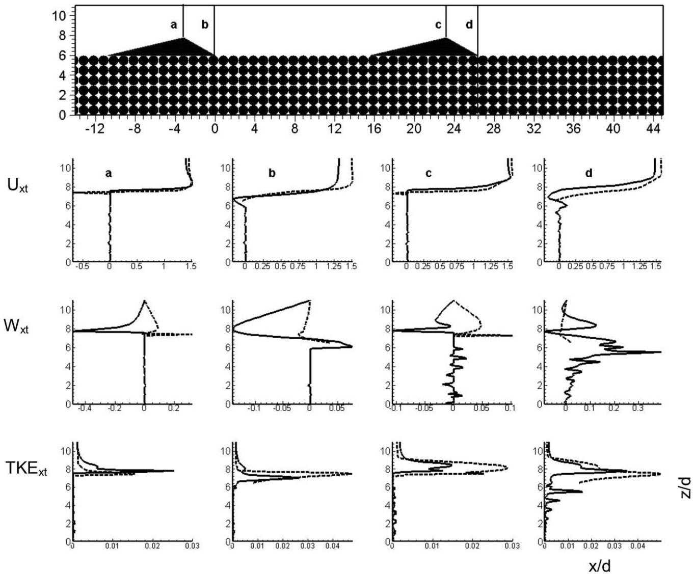
Figure 7. Velocity profiles from the crest of the downstream dune for flow over two impermeable dunes in sequence over an impermeable bed (dashed) and a permeable bed (solid). Columns a–d represent locations downstream (a) at the crest of the dune; (b) at the base of the leeslope of the upstream bed form; (c) at the crest of the second dune, and; (d) at the base of the leeslope of the downstream dune for nondimensionalized downstream velocity ( U_{xt} ) (row 2), nondimensionalized vertical velocity ( W_{xt} ) (row 3) and nondimensionalized turbulent kinetic energy ( TKE_{xt} ) (row 4).
