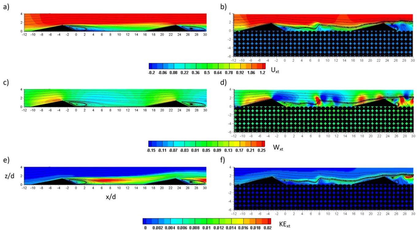
Figure 6. The predicted flow over two bed forms in sequence over an impermeable bed (a, c, and e) and over a permeable bed (b, d, and f) for (a and b) nondimensionalized downstream velocity ( U_{xt} ), (c and d) the nondimensionalized vertical velocity ( W_{xt} ), and (e and f) nondimensionalized turbulent kinetic energy (TKE _{xt} ). In all plots, the profile is taken down the midline of the domain ( y/w = 0.5 ) with x/d on the abscissa axis and z/d is on the ordinate axis. Flow is from left to right.
