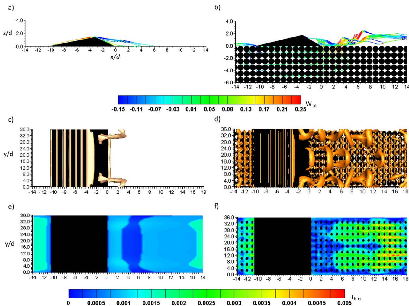
Figure 3. (a, c, and e) The predicted flow over a single dune placed on an impermeable bed and (b, d, and f) permeable bed for a series of streamlines colored with nondimensionalized vertical velocity ( W_{xt} ) (a and b); the Q criterion (thresholded at 3.5) (c and d) and the near-bed shear stress (e and f). In (a) and (b), the profile is taken down the midline of the domain ( y/w = 0.5 ) with x/d on the abscissa axis and z/d is on the ordinate axis. In (c)–(f), a plan view is applied with x/d on the abscissa axis and y/d is on the ordinate axis. Flow is from left to right.
