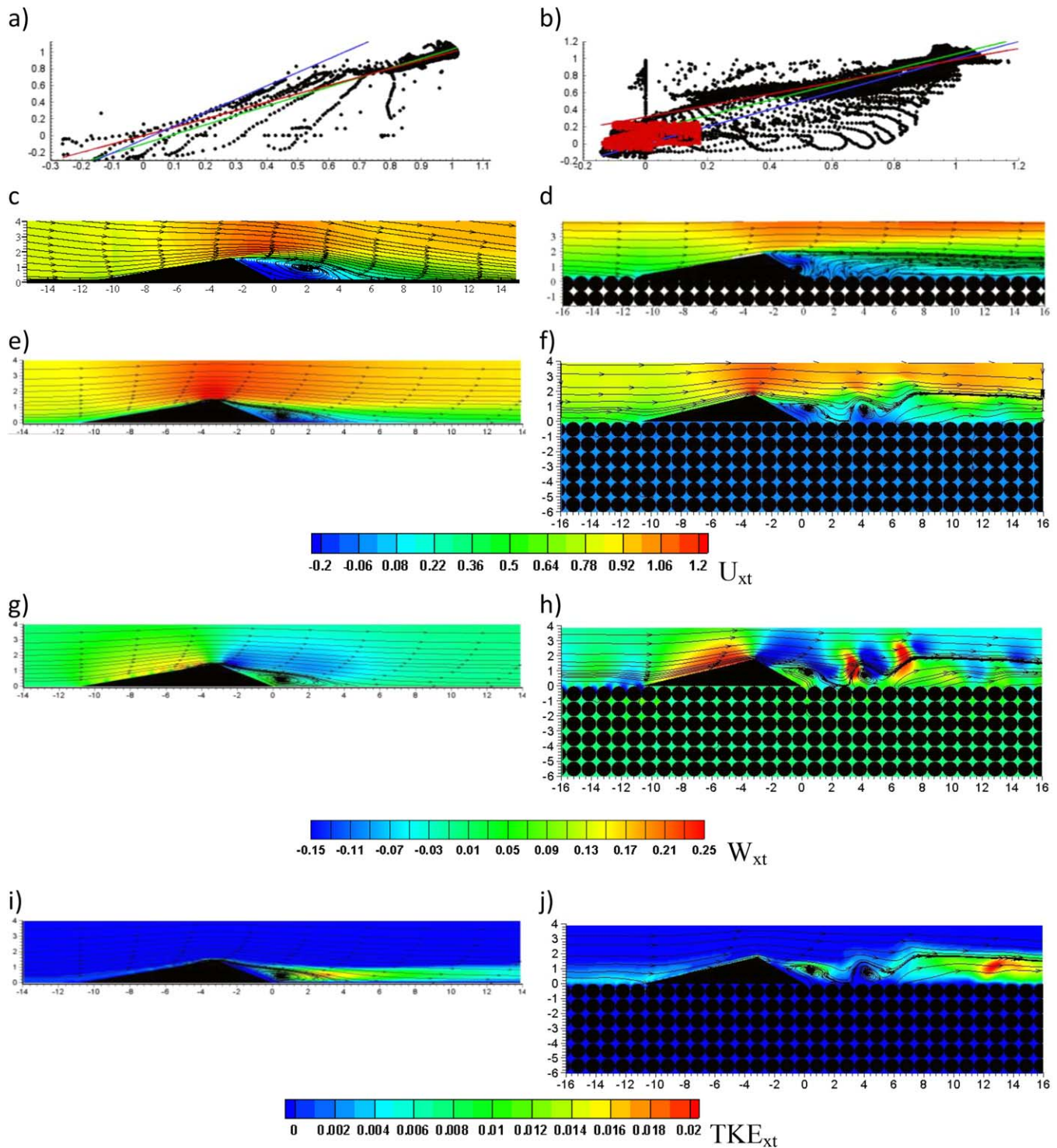
Figure 1. Flow over a single impermeable dune over: (a, c, e, g, and i) an impermeable bed and (b, d, h, h, and j) a permeable bed. The velocity results have been nondimensionalized with respect to the inlet velocity ( U_0 ), while the turbulent kinetic energy is nondimensionalized with the square of inlet velocity. The axes are nondimensionalized with the diameter of the spheres used to represent porous bed. The results are shown for the validation test between the modeled and experimental results of Blois et al. [2014] (a and b) where the modeled velocity is on the x axis and the experimental data on the y axis. The black markers represent the geo-located points, the green line the Reduced Major Axis (RMA) regression line, the red line the linear trend line and the blue line: 1:1 line. The red markers represent flow within the bed for pores in the vicinity of the bed form. The interpolated whole flow fields of the nondimensionalized downstream velocity ( U_{xt} ) from the experimental results of Blois et al. [2014] (c and d) can be compared to the modeled nondimensionalized downstream ( U_{xt} ) modeled (e and f). (g and h) The modeled nondimensionalized vertical ( W_{xt} ) and (i and j) nondimensionalized turbulent kinetic energy TKE_{xt} are also shown. The major flow characteristics are reported in Table 2 for comparison with the other numerical experiments. The flow is from right to left.
