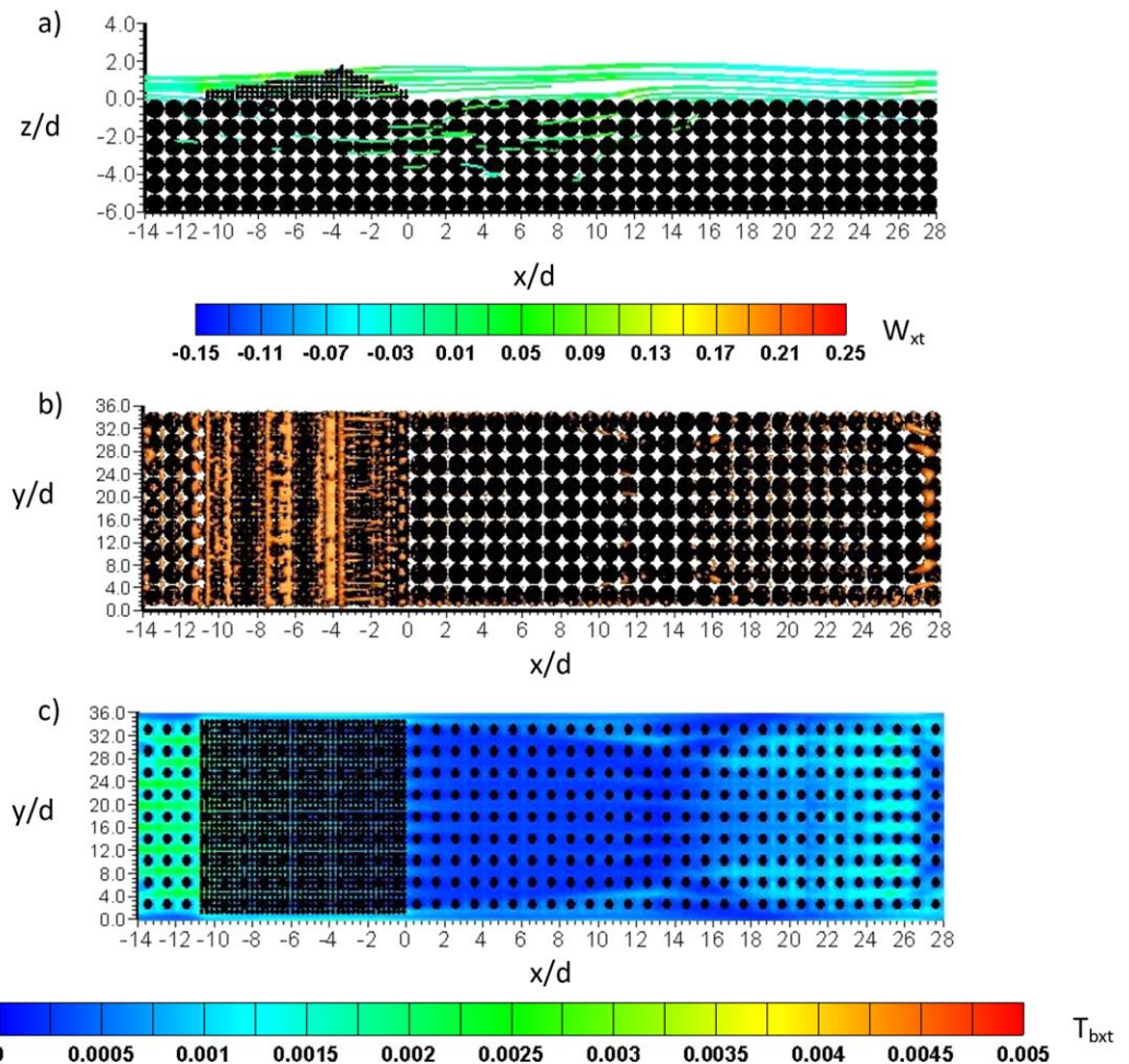
Figure 5. The predicted flow over a single permeable dune placed on a permeable bed for (a) a series of streamlines coloured with the nondimensionalized vertical velocity ( W_{xt} ); (b) the Q criterion (thresholded at 3.5) and; (c) the nondimensionalized near-bed shear stress. In (a) the profile is taken down the midline of the domain ( y/w = 0.5 ) with x/d on the abscissa axis and z/d is on the ordinate axis. In (c) and (b), a plan view is applied with x/d on the abscissa axis and y/d is on the ordinate axis. Flow is from left to right.
