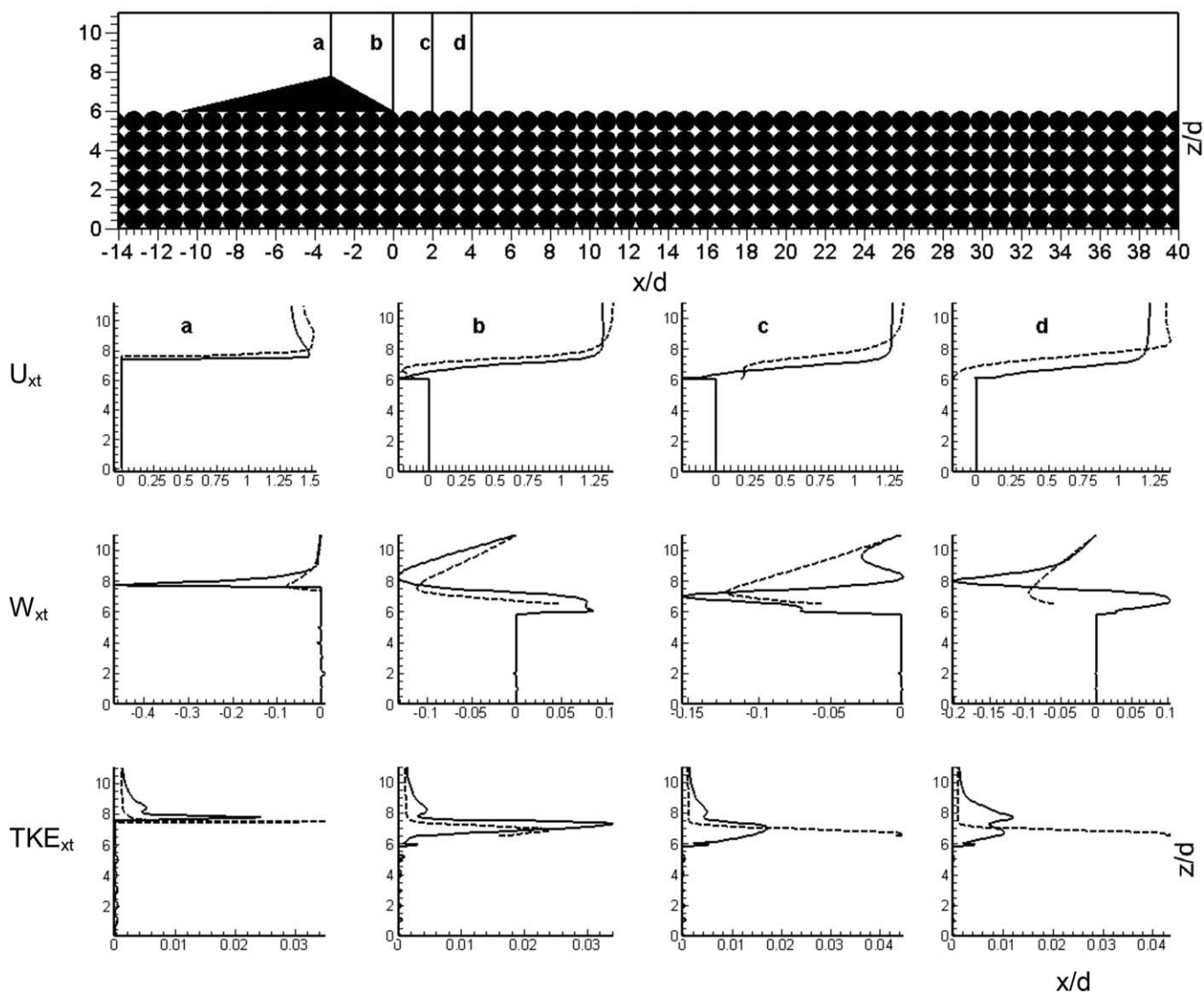
Figure 2. The velocity profiles from the crest of the dune downstream for flow over an impermeable dune over an impermeable bed (dashed) and a permeable bed (solid). Columns a–d represent locations downstream: with (a) at the crest of the dune; (b) at the end of the dune; (c) 2 x/d from end of dune, and; (d) 4 x/d from end of dune for nondimensionalized downstream velocity ( U_{xt} ) (row 2), nondimensionalized vertical velocity ( W_{xt} ) (row 3), and nondimensionalized turbulent kinetic energy ( TKE_{xt} ) (row 4).
