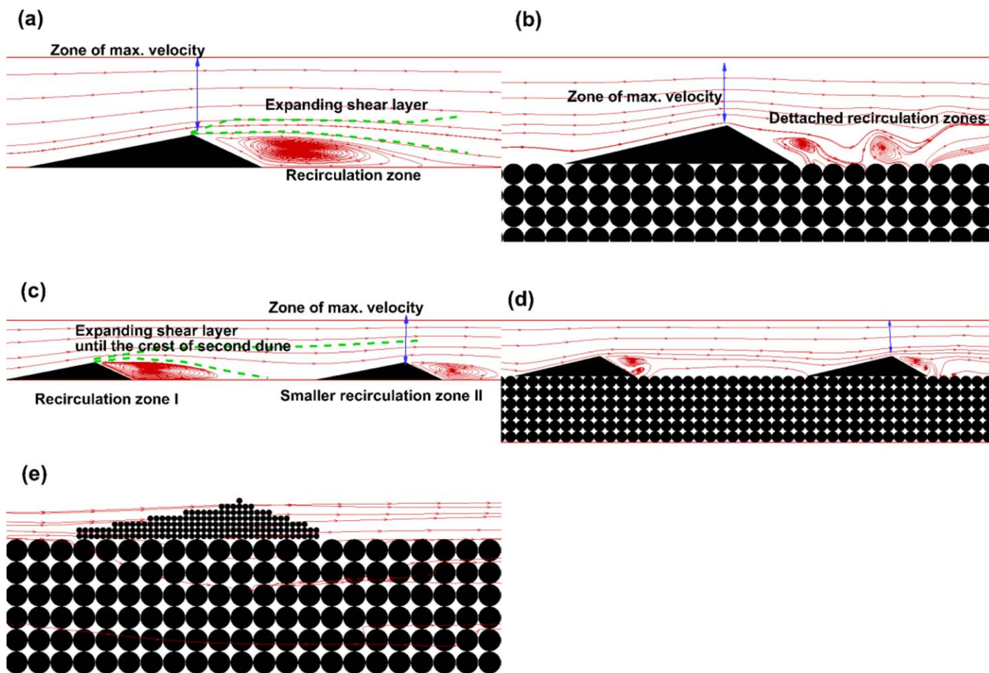
Figure 9. A schematic model of flow over dunes depending on the im/permeability of the dune, the bed or both for either a single dune or a series of dunes. The flow structures associated with the different bed forms are discussed in the text.
