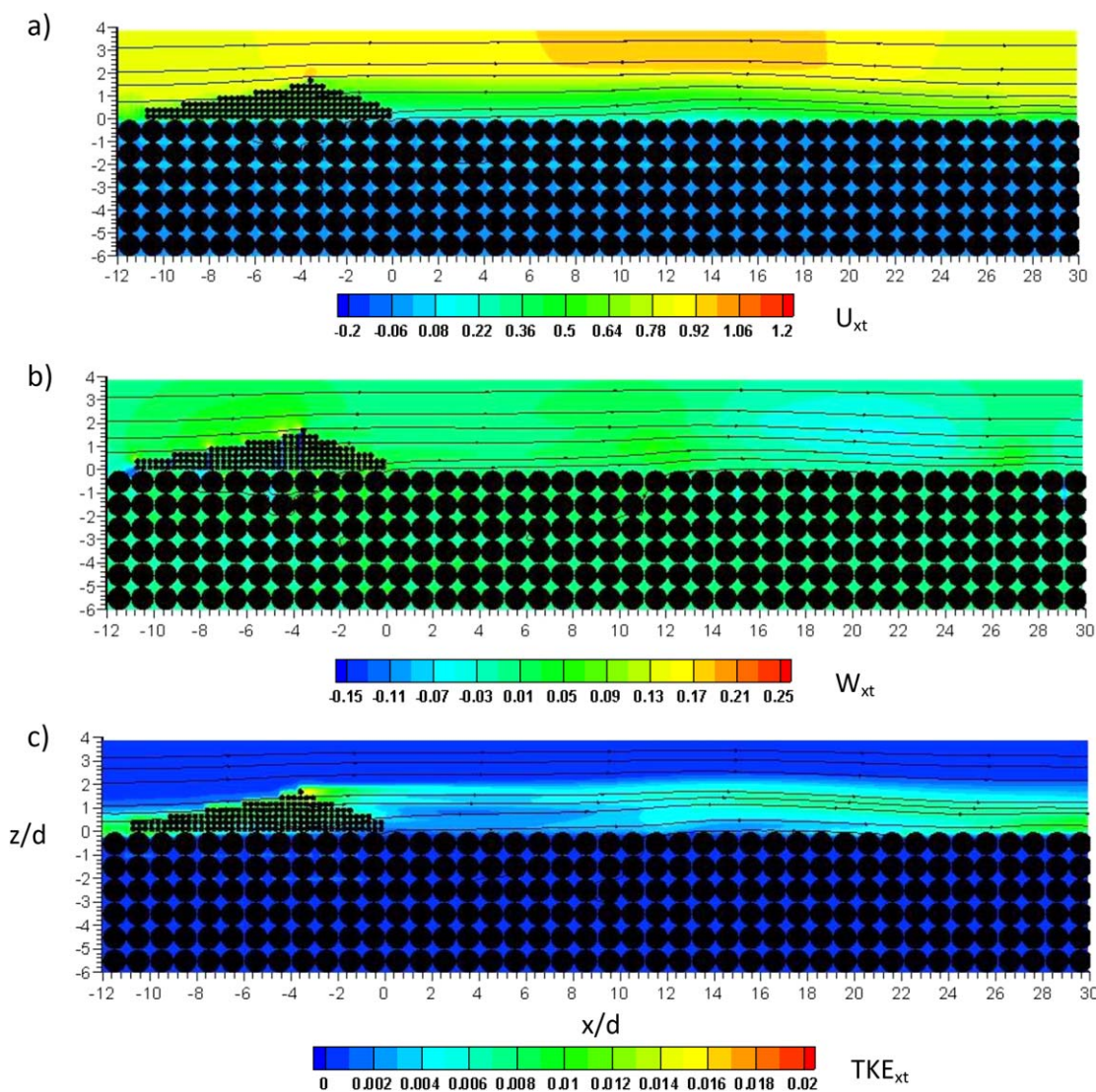
Figure 4. (a) The modeled flow over a permeable dune over a permeable bed for; (b) nondimensionalized downstream velocity ( U_{xt} ) nondimensionalized vertical velocity ( W_{xt} ) and (b), nondimensionalized turbulent kinetic energy ( TKE_{xt} ). In all plots, the profile is taken down the midline of the domain ( y/i = 0.5 ) with x/d on the abscissa axis and z/d is on the ordinate axis. The major flow characteristics are reported in Table 2 for comparison with the other numerical experiments. Flow is from left to right.
