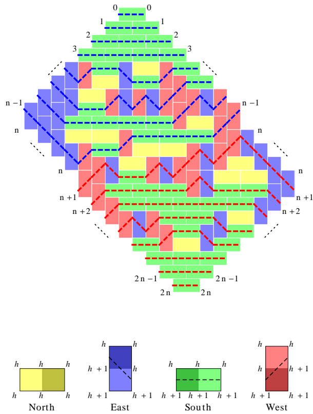
Figure 4: The level lines including the height function around the boundary. The heights change in the interior only when crossing a level line. The bottom figure shows the height change for each individual domino.
