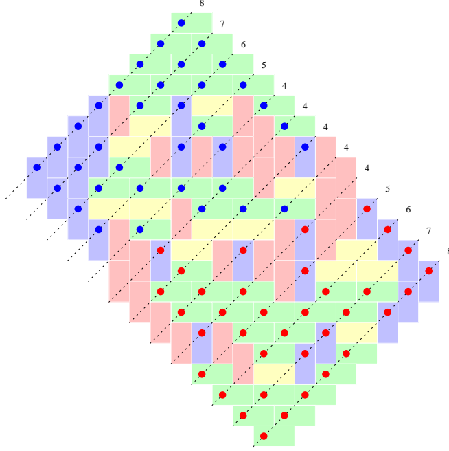
Figure 6: The red and blue L particles. The blue L particles correspond to Aztec diamond A while the red particles correspond to Aztec diamond B see Figure 1. The numbers represent the total number of particles on each line \xi = 2s
