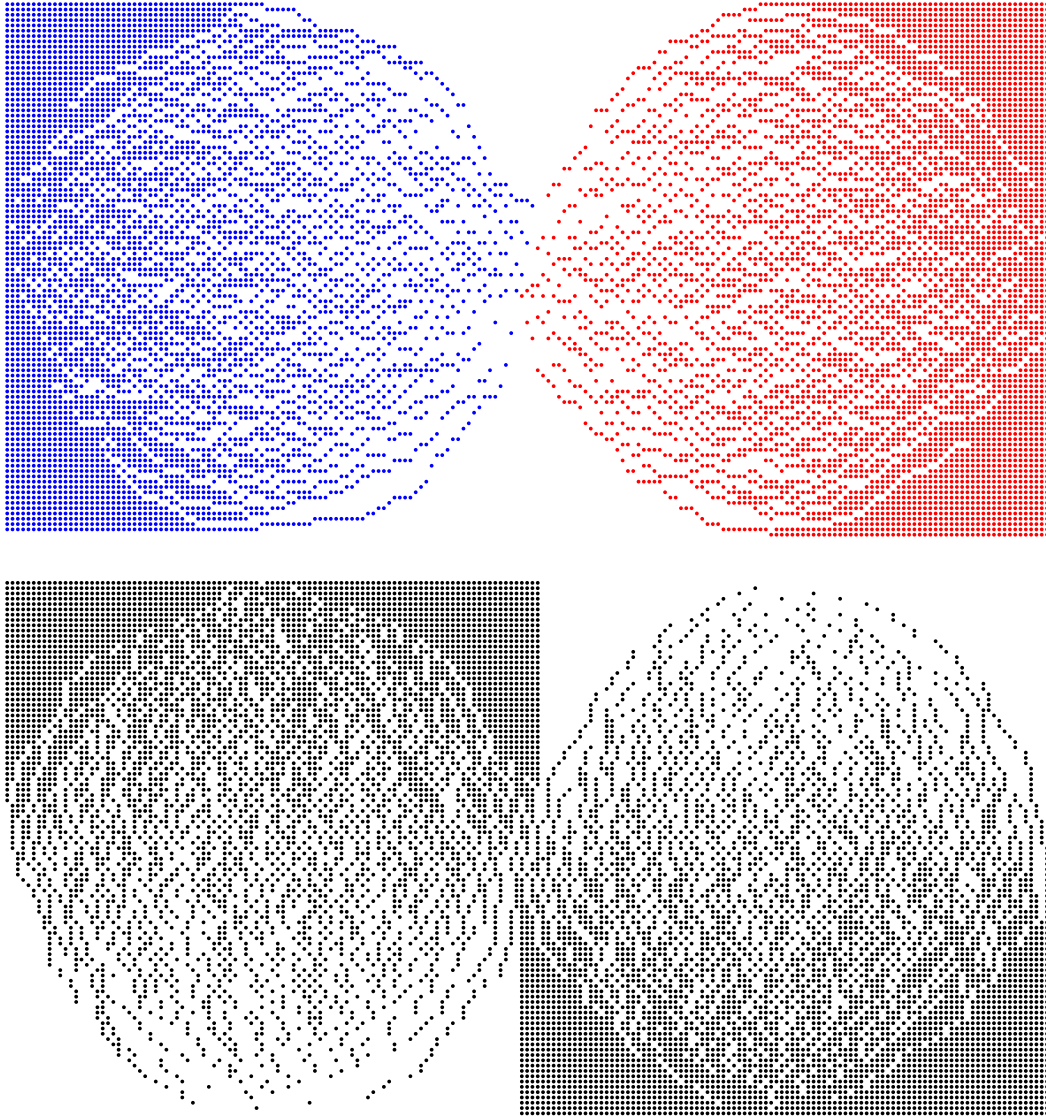
Figure 9: The top picture shows the blue and red \mathbb{L} -particles for the simulation of Figure 8: a particle is created each time a line \{\xi = 2s\} traverses a blue or green domino, as in Figure 8 (or, alternatively, crosses a level line); then blue particles belong to an A -level line and a red particles to a B -level line. The bottom picture shows the \mathbb{K} -particles for the same simulation in Figure 8: a particle is created each time a line \{\eta = 2r + 1\} traverses a red or green domino, as in Figure 8 (or, alternatively, crosses a level line).
