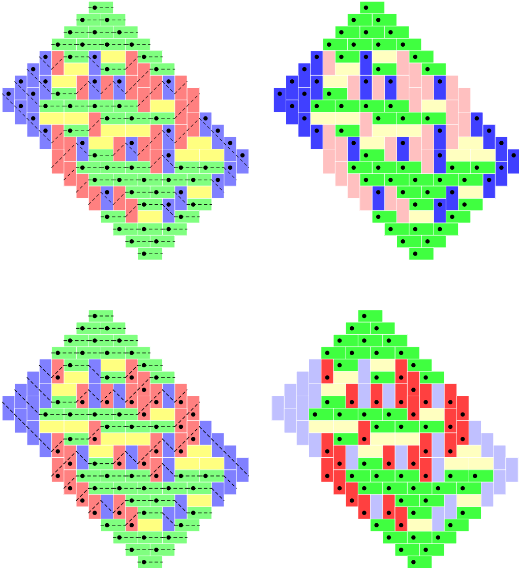
Figure 5: The top figures show the \mathbb{L} particle process using the level lines (on the left) and the dominos on the right. There is an \mathbb{L} particle for every green (south) and blue (east) domino. The bottom figures show the \mathbb{K} particle process. There is a \mathbb{K} particle for every green (south) and red (west) domino.
