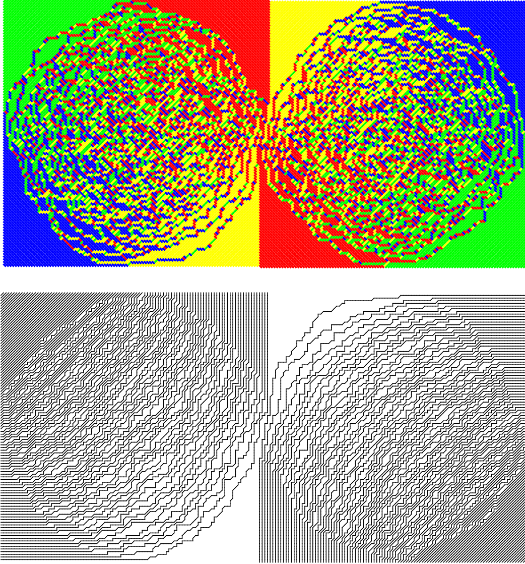
Figure 8: A simulation of a double Aztec diamond with n = 100 and \rho = 4 with the weight a of vertical and horizontal tiles equal to 1. Both figures are rotated by \pi/4 counter-clockwise. For this simulation, the top figure shows the underlying domino tiling while the bottom figure shows the level lines. The simulation was made using the generalized domino shuffle [23].
