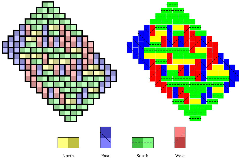
Figure 3: Random Tiling of a double Aztec diamond with n = 8 and \rho = 4 . The figure on the left shows the underlying checkerboard structure while the figure on the right shows the same tiling with the level lines. These are shown explicitly for the four types of dominos in the bottom figure. These level lines are the same as the DR lattice paths [21].
