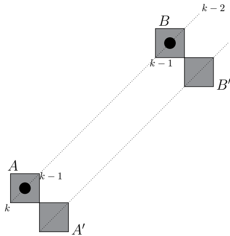
Figure 13: Between the two gray squares labeled A and B the height function stays constant; therefore the line between A and B contains no dots.
