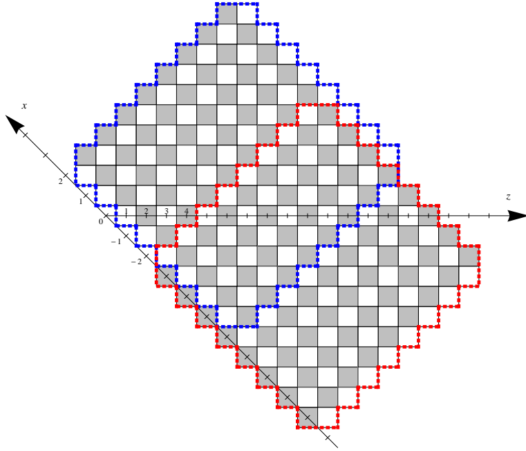
Figure 2: Double Aztec diamond with n = 8 and overlap \rho = 4 with the (z, x) coordinates of the Aztec diamond.
