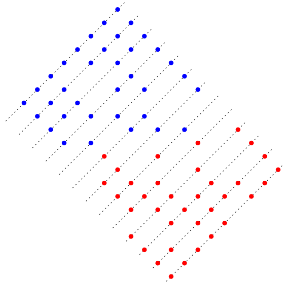
Figure 7: The interlacing system of blue and red dots. The \rho + 1 lines, \{\xi = 2s\} \in A \cap B and \{\xi = 2(n - \rho)\} \in A , contain \rho dots. All the other lines contain more dots. See Proposition 1.3 for more details on the interlacing.
