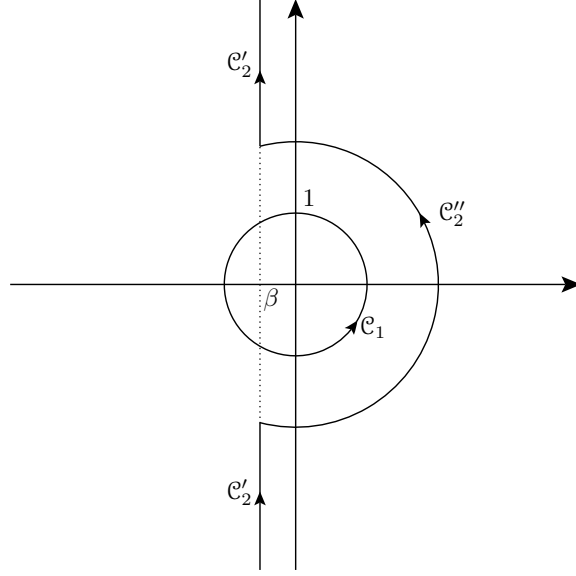
Figure 15: The contour paths
