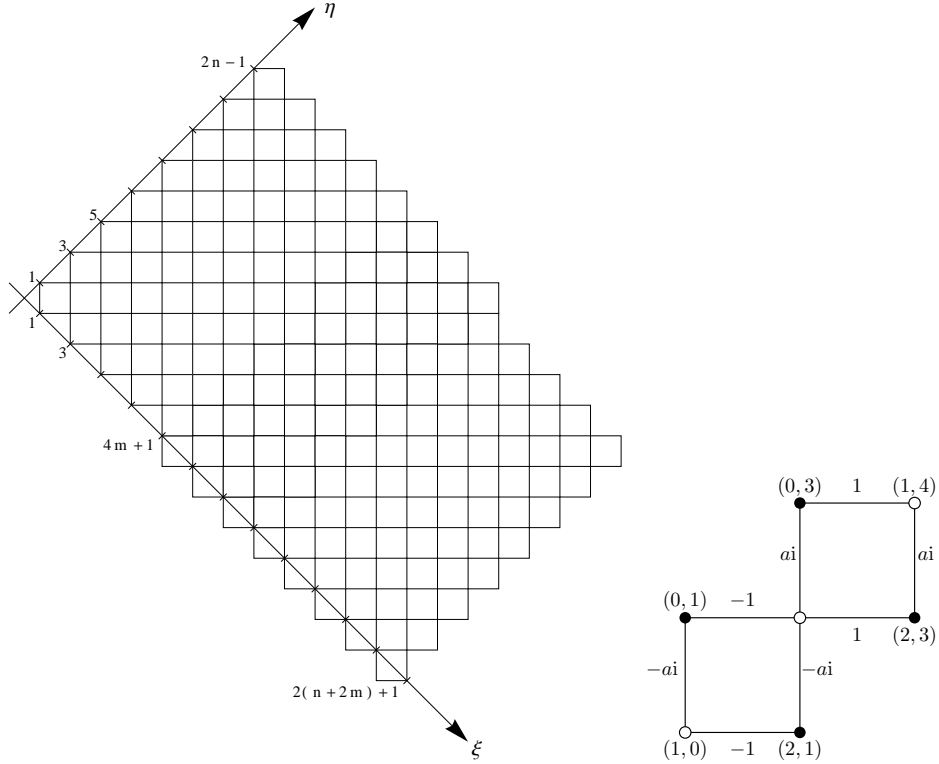
Figure 10: The left hand figure shows the dual graph of the double Aztec diamond with n = 8 and m = 4 in the (\xi, \eta) co-ordinates. The right hand figure shows the weights, Kasteleyn orientation, black and white vertices for the two most left squares, with (\xi, \eta) -coordinates.
