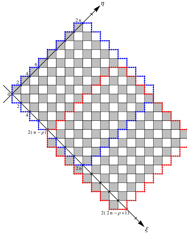
Figure 1: Double Aztec diamond with n = 8 and overlap \rho = 4 , with the (\xi, \eta) coordinates with Aztec diamond A enclosed by the blue dotted line and Aztec diamond B enclosed by the red dotted line. The overlap contains \rho lines (through black squares) \xi = 2s for n - \rho < s \leq n .
