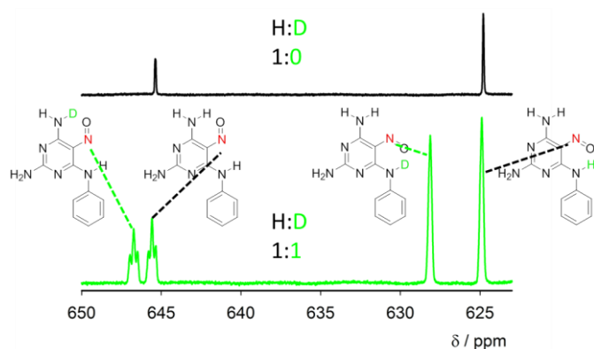
Fig. 4 Nitroso group region of ^{15}\text{N} NMR spectrum of compound 1 in DMSO (black spectrum) and of compound 1 recrystallized from \text{H}_2\text{O}/\text{D}_2\text{O} mixture (1:1) and dissolved in DMSO (green spectrum). The assignment of the signals is based on a comparison with spectra with a different H:D ratio and with spectra of similar model compounds (details in the SI). Expansion of the spectra with the signal assignments is depicted in the SI (Figure S6).
