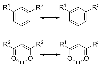
Fig. 1 The interrelation between the resonance-assisted hydrogen bond and \pi -electron delocalisation.
