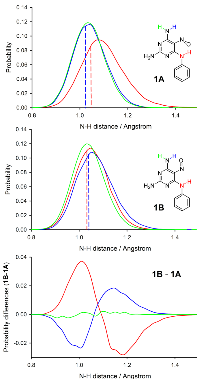
Fig. 3 Probability distributions (sampled by 0.02 Å) and their differences of N–H bond distances obtained from PIMD simulations of both rotamers of compound 1 . The dashed lines indicate geometry optimised N–H distance. No rotation of the NH 2 group around the C–N bond was observed during the PIMD simulations. Every 10 ps PIMD simulation took ca 10 days on 128 computational cores.
