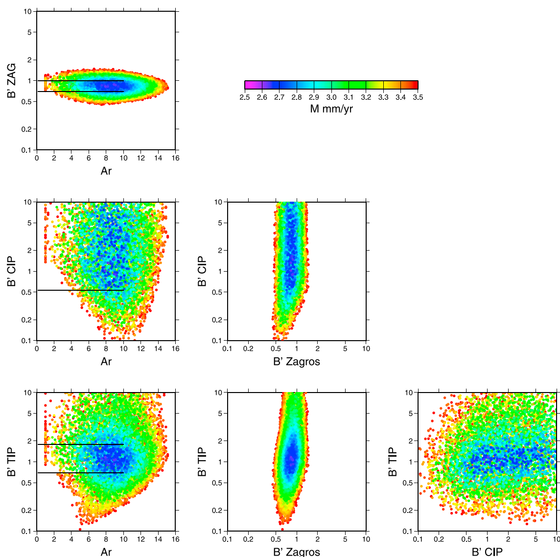
Figure 7. Weighted misfits M (equation (12)) for 100,000 random combinations of Ar and B' in the Turkish-Iranian Plateau ( B'_{TIP} ), Central Iranian Plateau ( B'_{CIP} ), and Zagros, ( B'_{ZAG} ). In each panel, colored dots (scale at top) show the minimum value of M obtained in the two-dimensional slice through the four-dimensional parameter space. Horizontal lines in the left-hand column show the ranges of B' for which M is lower than for the best-fitting solution for the homogeneous sheet with n = 3 .
