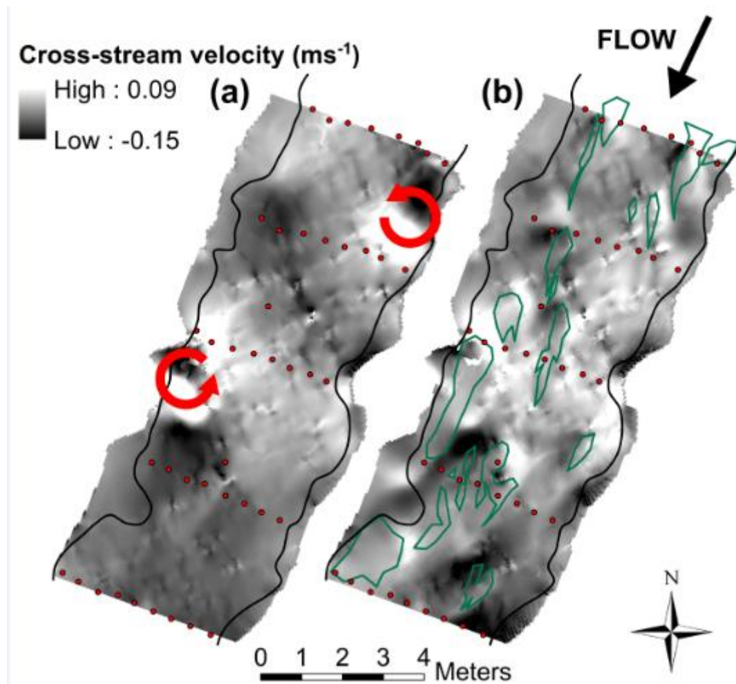
Figure 9: Depth-averaged cross-stream velocity predictions for the (a) unvegetated and (b) vegetated channel. Vegetation patches shown in green. Flow recirculation regions shown in red.
