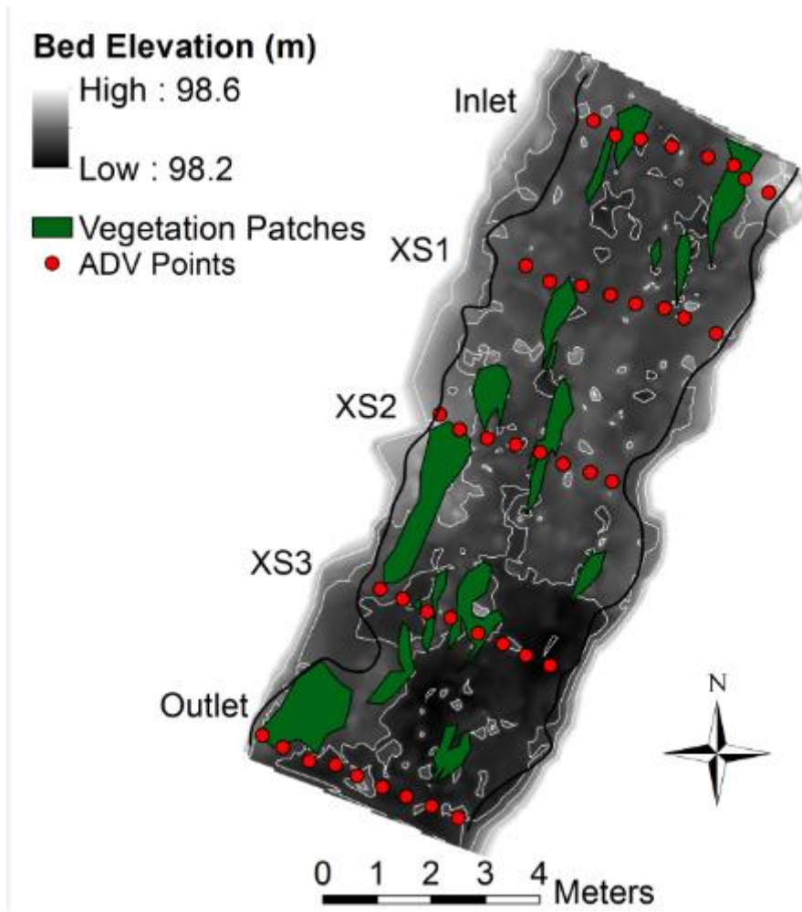
Figure 1: Field setup. Green patches represent vegetation, red circles show ADV points and the contour map shows the topography
