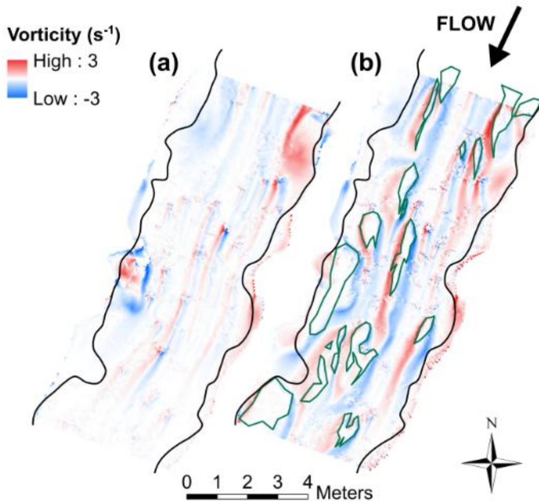
Figure 13: Vorticity plots for the (a) unvegetated and (b) vegetated channels. Vegetation patches shown in green.
