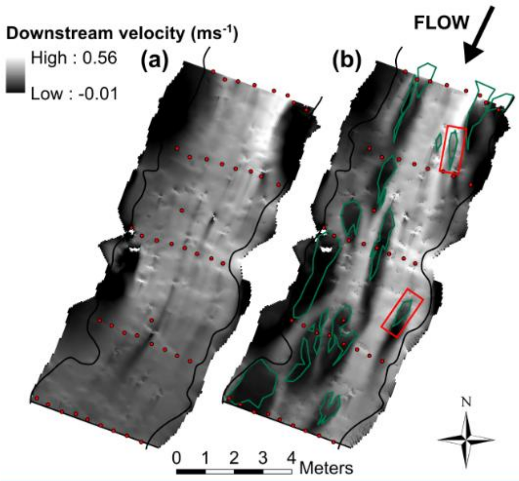
Figure 8: Depth-averaged downstream velocity predictions for the (a) unvegetated and (b) vegetated channel. Vegetation patches shown in green with two similar patches shown in red boxes.
