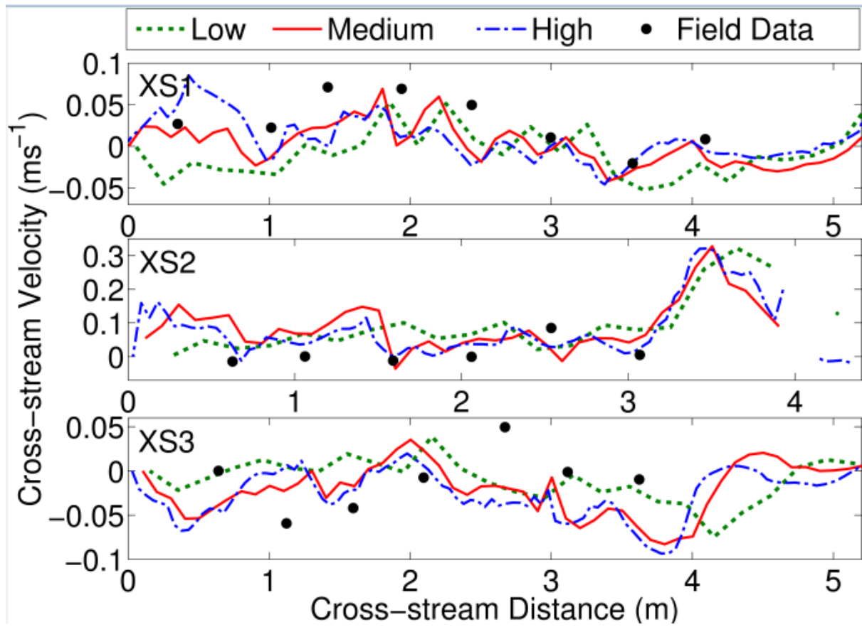
Figure 7: Cross-stream velocity profiles at cross-sections 1,2 and 3 for low, medium and high resolution.
