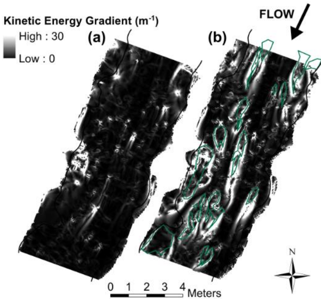
Figure 12: Kinetic energy gradient for the (a) unvegetated and (b) vegetated channels. Vegetation patches shown in green.
