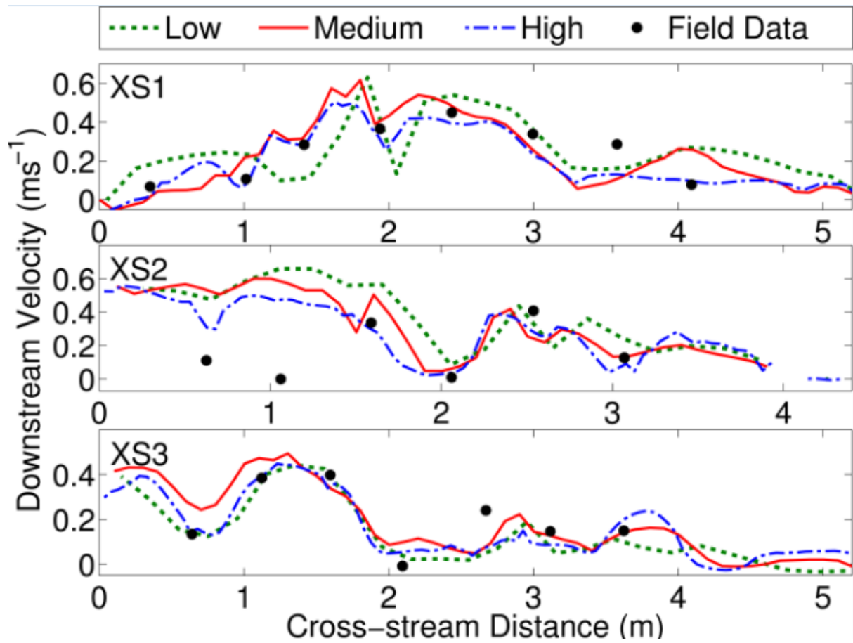
Figure 6: Downstream velocity profiles at cross-sections 1,2 and 3 for low, medium and high resolution.
