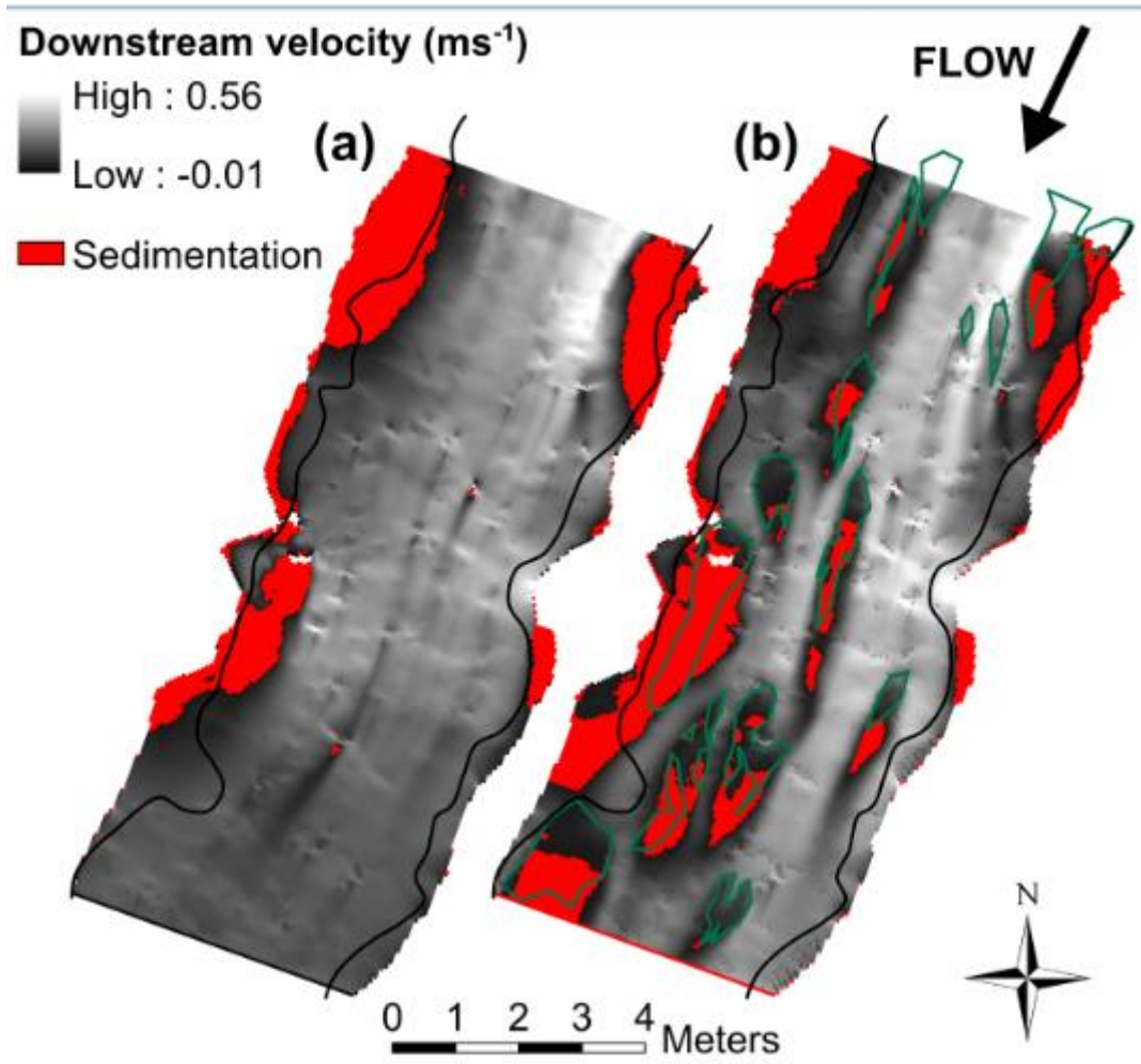
Figure 11: Inferred deposition patterns for the (a) unvegetated and (b) vegetated channels using the approach of de Lima et al. (2015). Areas of deposition are shown in red. Vegetation patches shown in green.
