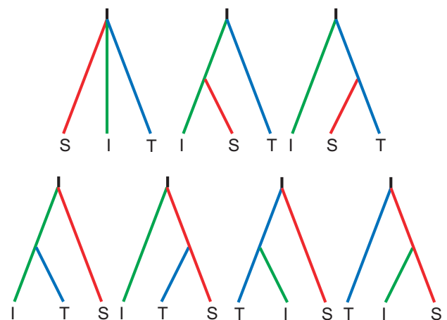
Figure 2 Graphical representation of the seven scenarios considered with approximate Bayesian computation using the software DIYABC. See Table 3 and Supplementary Table S7 and Supplementary Figures S4 and S5 for the results of the analysis.
