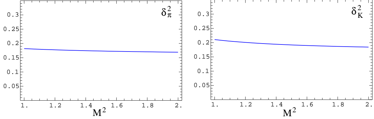
Figure 8: Left panel: \delta_\pi^2 as a function of the Bore parameter from the sum rule (D.5); s_0 = 0.8 \text{ GeV}^2 . Right panel: the same for \delta_K^2 ; s_0 = 1.1 \text{ GeV}^2 .
