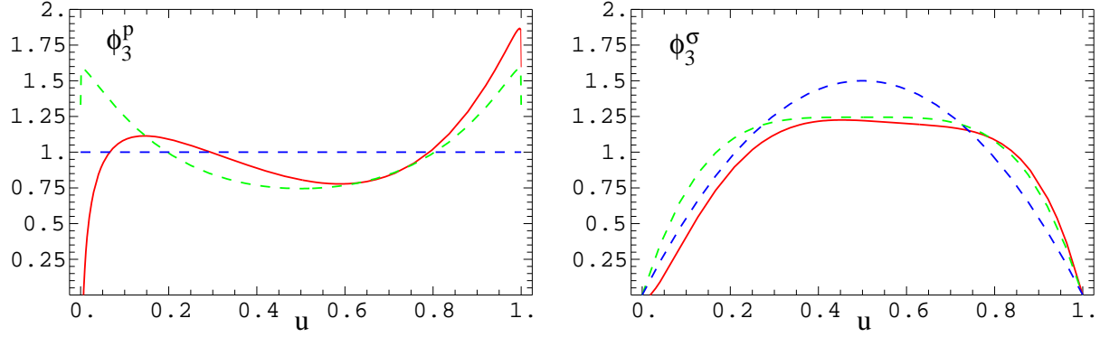
Figure 1: Left panel: \phi_3^p as a function of u for the central value of the hadronic parameters, for \mu = 1 GeV. Red (solid) line: \phi_{3;K}^p , green (long dashed): \phi_{3;\pi}^p , blue (short dashed): asymptotic DA. Right panel: same for \phi_3^\sigma .
