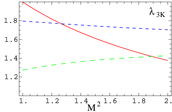
Figure 7: \lambda_{3K} as a function of the Borel parameter, calculated from the non-diagonal sum rule (C.16) (red, solid line), the pure-parity diagonal sum rule (C.14) (green, long dashes) and the mixed-parity diagonal sum rule (C.15) (blue, short dashes); s_0 = 1.1 \text{ GeV}^2 ; \lambda_{3\pi} = 0 by virtue of G-parity.
