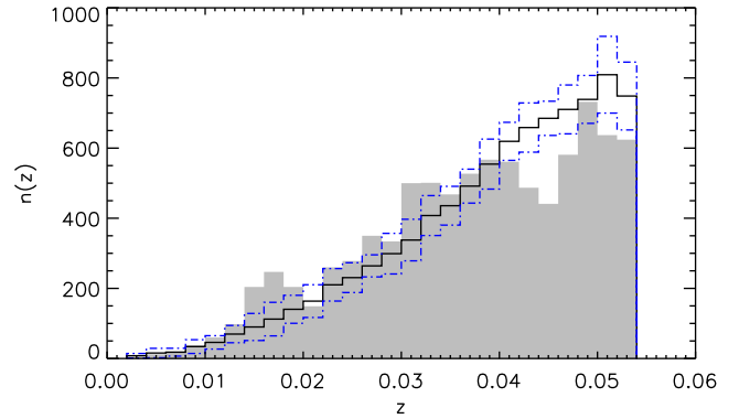
Figure 6. The mean redshift distribution of our 20 GigggleZ mocks (black histogram), along with the standard deviation (blue dot-dashed histograms), compared to 6dFGSv (solid grey histogram).
