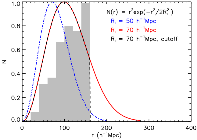
Figure 5. Radial number distribution N(r) of the Gaussian filters we use for measuring the 6dFGSv bulk flow. The filters have (i) R_1 = 50 h^{-1} \text{Mpc} radius (blue dot-dashed line), (ii) R_1 = 70 h^{-1} \text{Mpc} radius (red solid line), and (iii) R_1 = 70 h^{-1} \text{Mpc} radius with a cut-off at 160 h^{-1} \text{Mpc} , corresponding to the redshift cut of the data (black dashed). The distribution of the data is shown by the grey histogram for comparison.
