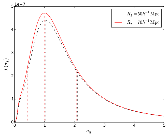
Figure 12. Likelihood of the value of \sigma_8 from our bulk flow measurement, after marginalising over \Omega_m . The black dashed curve is for the MV R_1 = 50 h^{-1} Mpc measurement, and the red curve is for R_1 = 70 h^{-1} Mpc. The dotted lines indicate the maximum of the likelihood and 68.27 per cent confidence levels.
