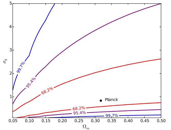
Figure 11. The likelihood-based confidence levels on \Omega_m and \sigma_8 , obtained from the 6dFGSv MV bulk flow measurement with R_1 = 70 h^{-1} Mpc. The black point indicates the best-fitting values found by Planck , used as the fiducial values in this work. The result for R_1 = 50 h^{-1} Mpc is very similar to this plot.
