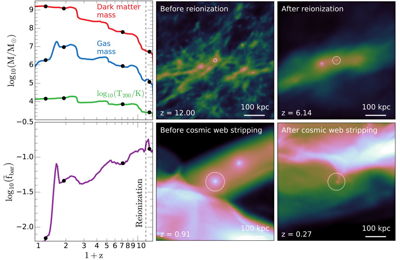
Figure 3. Evolution of a cosmic web stripped system from the V01-L1 simulations, with M_{200} \sim 10^{9.1} M_{\odot} at redshift z = 0 . The left-hand panels show the evolution of (from top to bottom) the dark mass and gas mass within r_{200} ; the logarithm of the virial temperature, T_{200} \sim 10^4 \text{ K} (V_{200}/17 \text{ km s}^{-1})^2 , and (bottom panel) the gas mass fraction ( M_{\text{gas}}/M_{200} ) in units of the universal value, f_{\text{bar}} = \Omega_b/(\Omega_0 + \Omega_b) . The four panels on the right show snapshots of the evolution, at the times indicated by the solid circles in the left-hand panels. Note how reionization heats up the gas at early times, reducing the halo baryon content. In this particular example, the system loses essentially all of its bound mass after passing through a dense region of the cosmic web at z \sim 0.6 .
