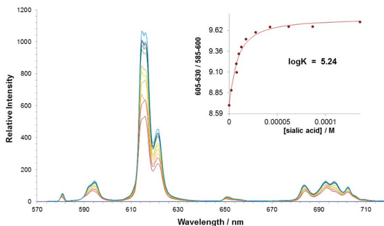
Figure 5 Variation of the europium (III) emission profile of [\text{Eu.L}^1]^+ as a function of added sialic acid. ( 5\ \mu\text{M} , \lambda_{\text{exc}} = 352\ \text{nm} , MeOH). Inset shows fit to experimental data, following iterative least squares fitting to a 1:1 binding model.
