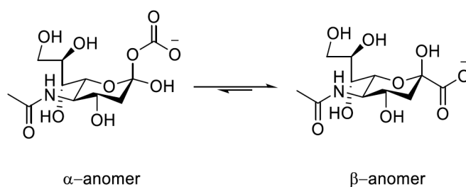
Figure 1 Structure of sialic acid (Neu-5-Ac) showing the \alpha - and \beta -pyranose forms; pK_a = 2.6 ( \text{H}_2\text{O} , I = 0.1 , 298K).
