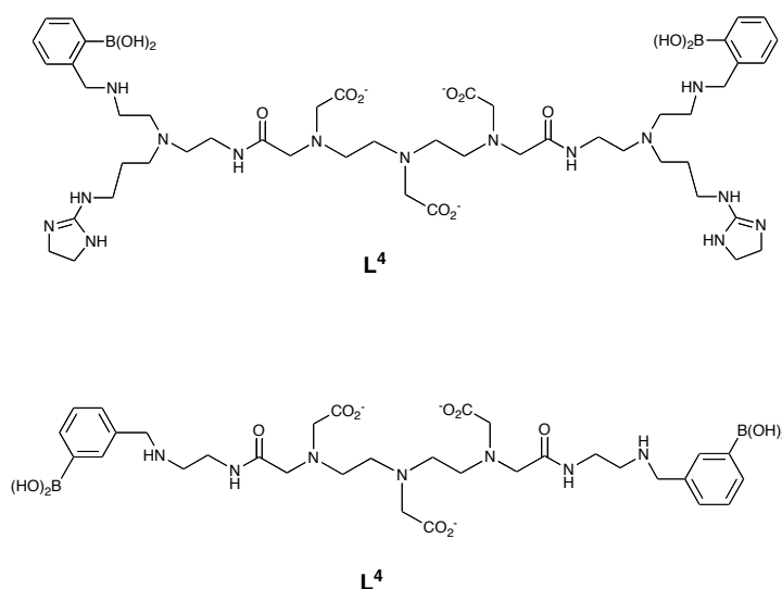
Figure 4 DTPA-bis amide (DTPA – diethylenetriamine pentaacetic acid) ligands used in Gd-based MRI contrast agents for sialic acid detection. 5
