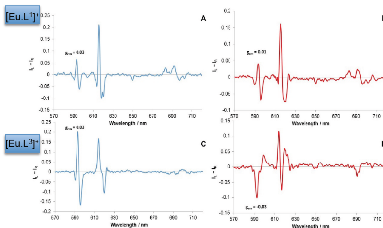
Figure 10 Induced CPL spectra for [\text{Eu.L}^1]^+ following the addition of A : 2 mM sialic acid; B : 2 mM sialic acid methyl ester (MeOH, \lambda_{\text{exc}} = 352 nm, 295 K). Induced CPL spectra for [\text{Eu.L}^3]^+ following the addition of C : 2 mM sialic acid; D : 2 mM sialic acid methyl ester (MeOH, \lambda_{\text{exc}} = 356 nm, 295 K). The g_{\text{em}} values are given for the same \Delta J = 1 transition at 593 nm.
