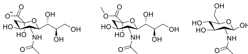
Figure 9 Structures of sialic acid ( left ), the corresponding methyl ester ( centre ) and N-acetyl-D-glucosamine ( right ).
