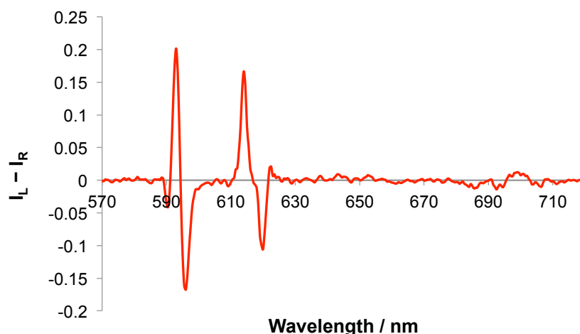
Figure 8 CPL spectrum of [\text{Eu.L}^3]^+ following addition of sialic acid (5 \mu\text{M} complex, 50 \mu\text{M} anion, \lambda_{\text{exc}} = 356 \text{ nm} , MeOH).
