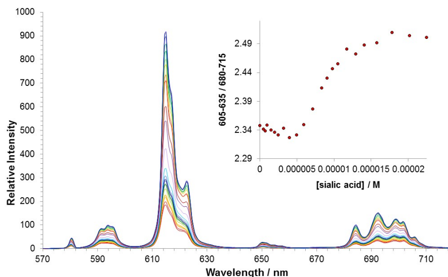
Figure 7 - Variation of the europium (III) emission profile of [\text{Eu.L}^3]^+ as a function of added sialic acid. ( 5 \mu\text{M} , \lambda_{\text{exc}} = 356 \text{ nm} , MeOH).
