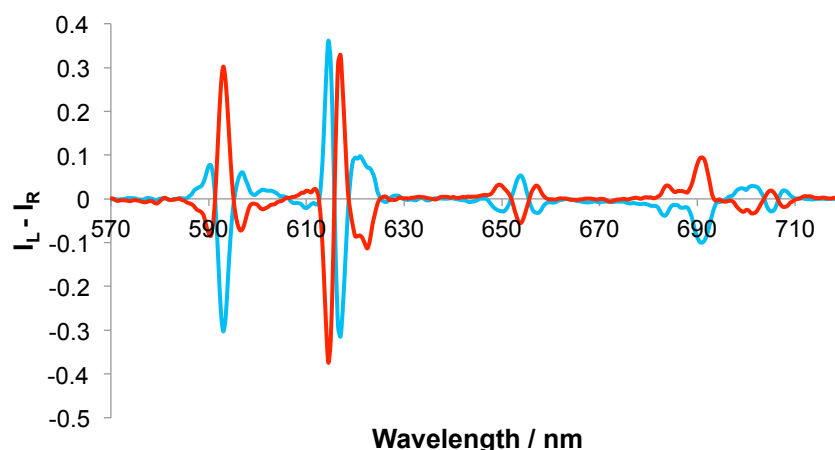
Figure 4 Induced CPL spectra of [\text{Eu.L}^3]^+ following the addition of 2 mM R - (red) and S -lactate (blue); g_{\text{em}}(593 \text{ nm}) = \pm 0.05 , g_{\text{em}}(654 \text{ nm}) = \pm 0.07 (5 \mu\text{M} complex, \lambda_{\text{exc}} = 356 \text{ nm} , MeOH, 295 K).
