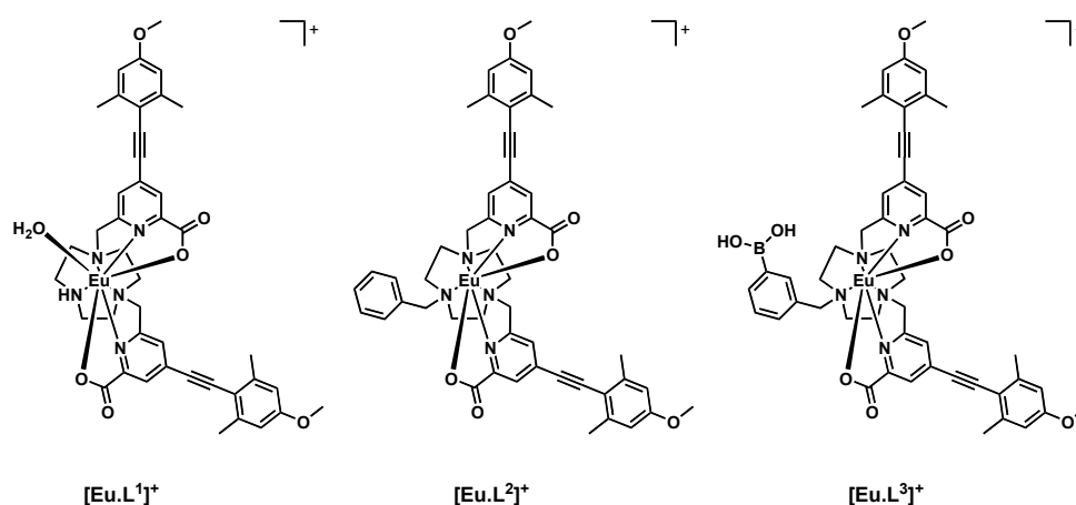
Figure 2 Structures of the Eu (III) complexes of \text{L}^{1-3} .
