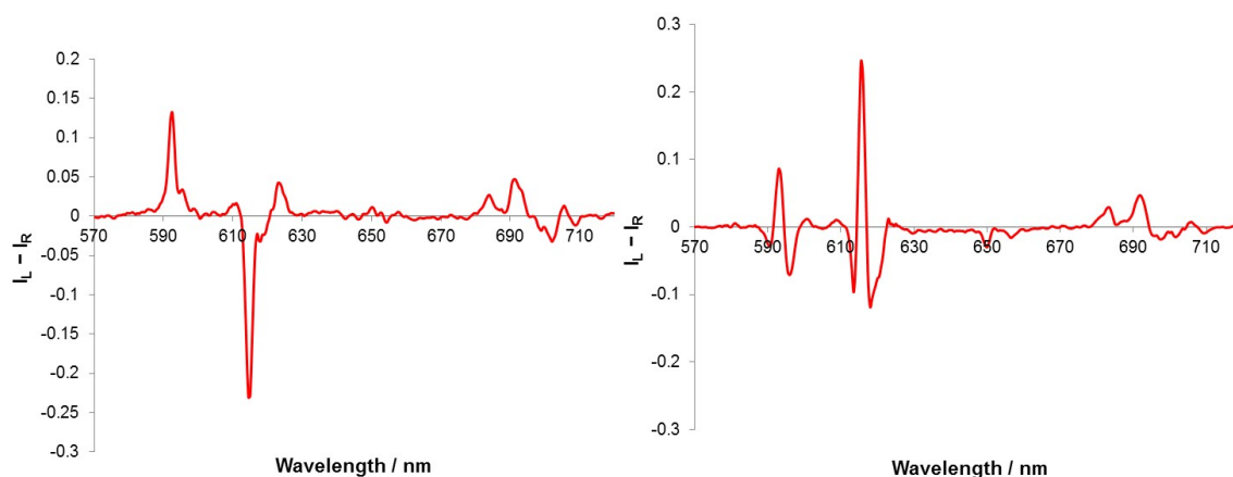
Figure 6 CPL spectra of [\text{Eu.L}^1]^+ following addition of R -lactate ( left ) and sialic acid ( right ). ( 5\ \mu\text{M} complex, 50\ \mu\text{M} anion, \lambda_{\text{exc}} = 352\ \text{nm} , MeOH).
