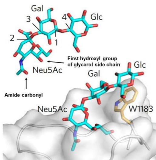
Figure 13 The sialic acid derivative binding site of the serum protein complement factor H, showing the orientation of the amide carbonyl oxygen and the first glycerol hydroxyl group to allow a cooperative binding interaction. 21
