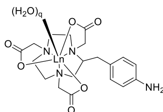
Figure 3 Partial structure of a [\text{Ln}.\text{ABNOTA}] complex; q = 2 or 3 . 9
