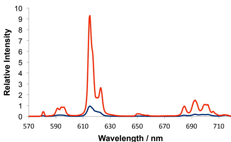
Figure 3 – Total emission spectra of [\text{Eu.L}^3]^+ (blue) and following addition of 2 mM S -lactate (red) (5 \mu\text{M} complex, \lambda_{\text{exc}} = 356 \text{ nm} , MeOH, 295 K).
