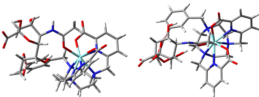
Figure 14 Views of the hypothetical binding of the glycerol diol group to boron and cooperative ligation of the amide carbonyl oxygen to the metal ion in an optimised model geometry for the complex [\text{Eu.L}^3.\text{sialic acid}] . 11,12
