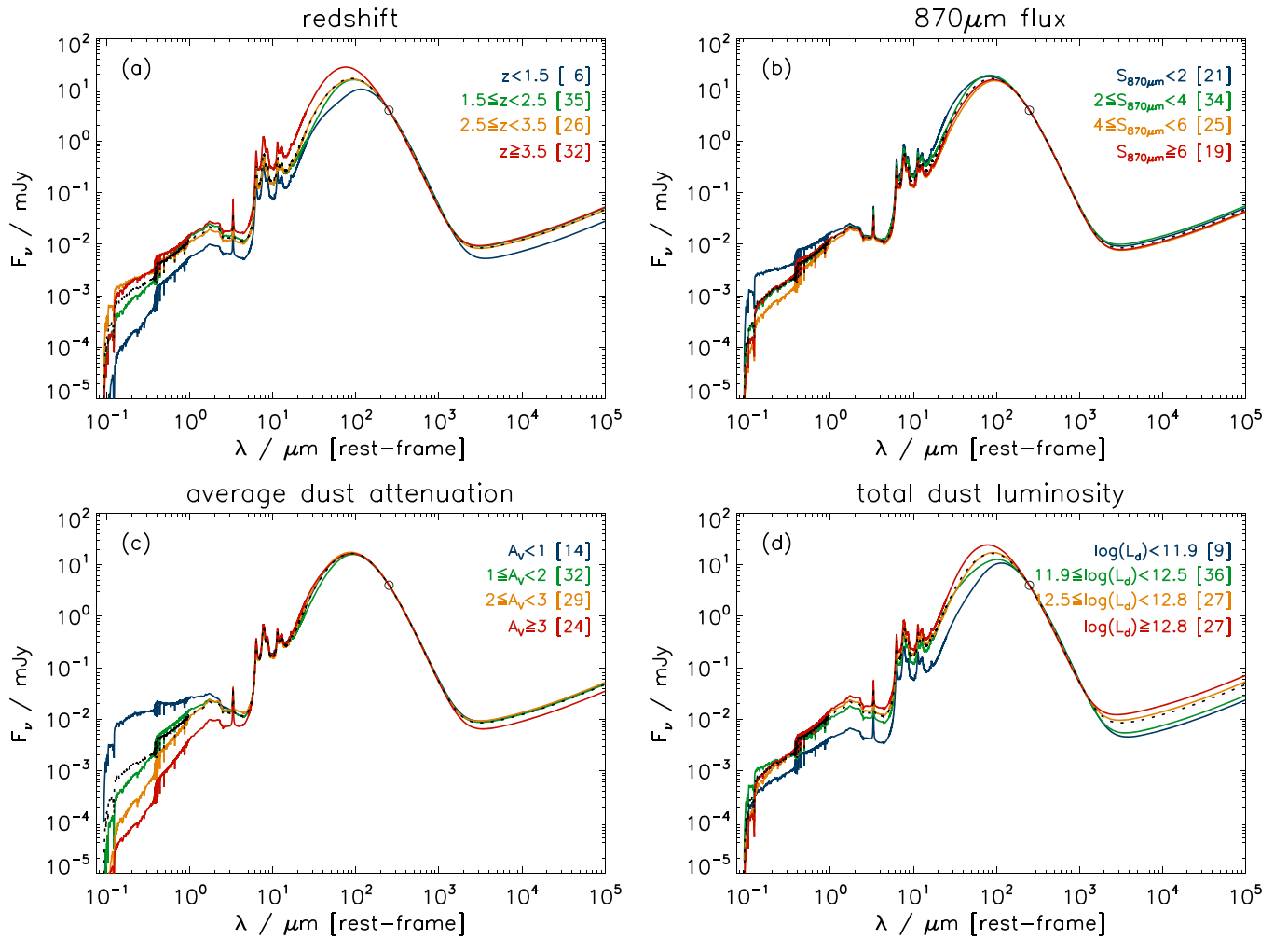
Figure 13. Variation of the intrinsic SED shapes of the 99 ALESS SMGs with different properties: (a) redshift; (b) observed 870\,\mu\text{m} flux measured with ALMA (in mJy); (c) average V-band dust attenuation; (d) total dust infrared luminosity (in L_\odot ). In each panel, we plot the average SED in four different bins of the parameter being considered, indicated in the top right-hand corner (the number in brackets indicates the number of sources falling in each bin). For reference, we also plot the average SED of all the sources (shown in Figure 11(a)) as a black dotted line. All the SEDs are normalized to the average ALMA 870\,\mu\text{m} flux of the sample, 4 mJy, at rest-frame 250\,\mu\text{m} , which corresponds to observed wavelength 870\,\mu\text{m} for a source at z = 2.5 (indicated by the black circle).
