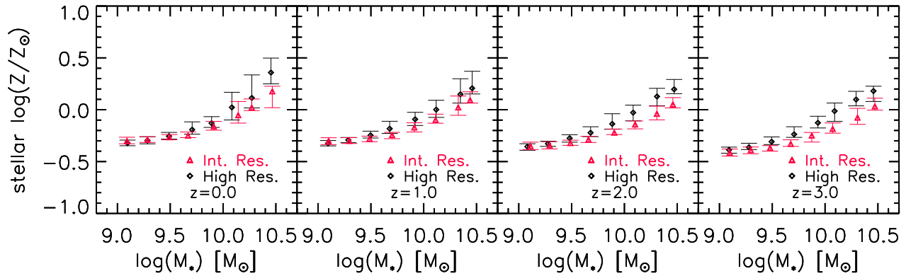
Figure A2. Stellar metallicity as a function of stellar mass at z \geq 0 for central galaxies in the high-resolution run (black) and intermediate-resolution run (red). The different curves with error bars depict the median relation with the 15th and 85th percentiles. Convergence is good, with a small tendency for higher values of Z at higher resolution.
