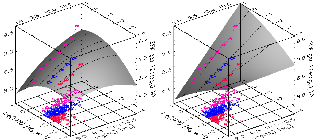
Figure 2. Location of observed galaxies in M_* –SFR–O/H space from Mannucci et al. (2010) (left panel) and of GIMIC galaxies (right panel). The shaded area in the left panel represents the best-fitting 2D surface to a Fundamental Plane taken from Mannucci et al. (2010); the right panel gives our fit to GIMIC galaxies. Lines with symbols depict the median M_* –O/H relations for bins in SFR from Fig. 1 (right panel); black lines trace the shaded surface at the centre of each SFR bin. The relation between M_* and SFR in the simulations is shown by the symbols in the M_* –SFR plane.
