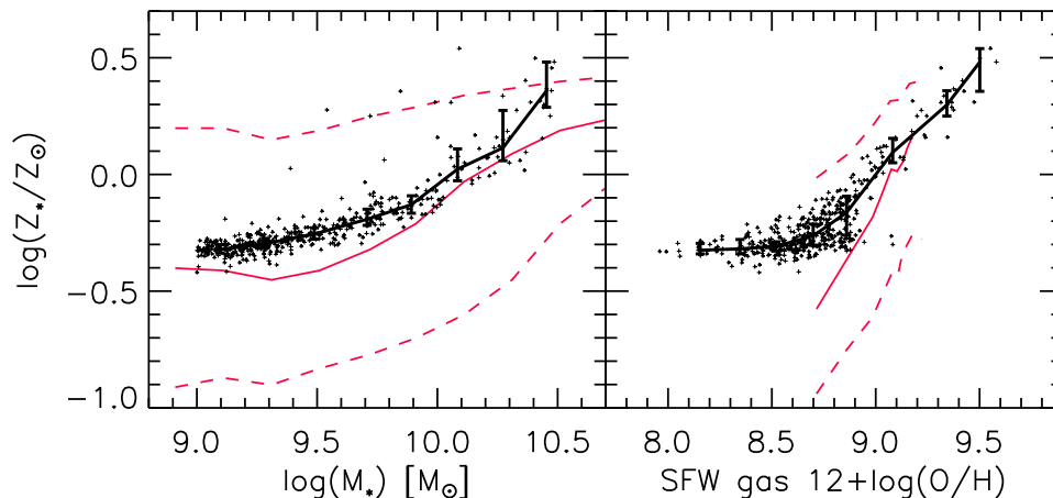
Figure 4. Median stellar metallicity as a function of stellar mass (left panel), and as a function of SFR-weighted gas O/H (right panel). GIMIC metallicities are shown as symbols, with black line showing the median relation, and the 25th and 75th percentiles indicated as error bars. Observational data from Gallazzi et al. (2005) are shown as full red lines (median), with dashed lines encompassing the 25th and 75th percentiles. The simulated relation follows the observed relation well in the left panel, but the most massive simulated galaxies are more metal rich as noted before; the scatter in the data is larger than in the simulation. The observed relation in the right panel is steeper than in the simulation, with simulated galaxies reaching a plateau of \log(Z_*/Z_\odot) \sim -0.4 at low gas abundance, which is not apparent in the data.
