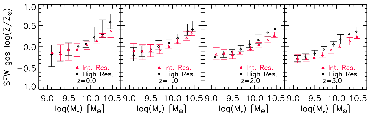
Figure A1. SFR-weighted gas-phase metallicity as a function of stellar mass at z \geq 0 for central galaxies in the high-resolution run (black) and intermediate-resolution run (red). The different curves with error bars depict the median relation with the 15th and 85th percentiles. The level of numerical convergence is good.
