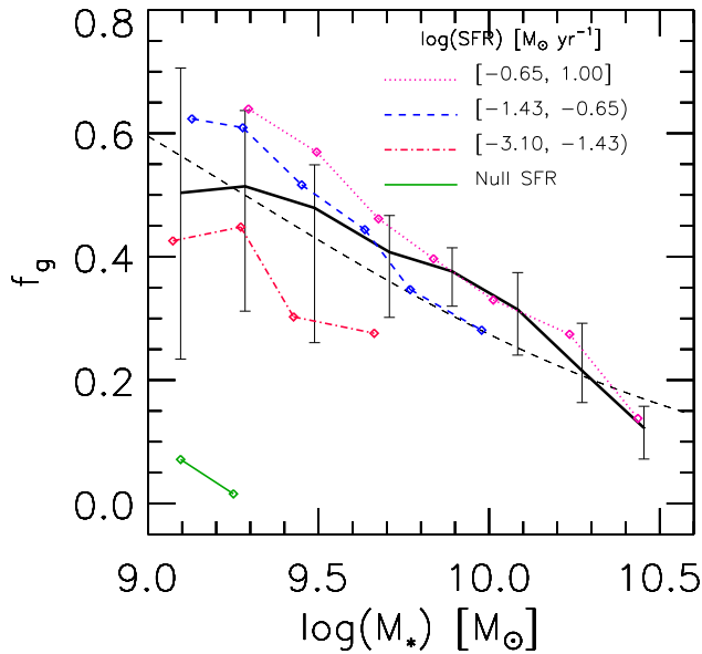
Figure 3. Median warm gas fraction, f_g \equiv M_g(T < 15000\text{K})/M_b , as a function of M_* at redshift z = 0 , M_b is the galaxy’s baryon mass (black solid line), with error bars indicating the 25th and 75th percentiles. The trend is in good agreement with the observed fraction from Stewart et al. (2009) (dashed black line). Coloured lines show the median of f_g in the simulation for bins in star formation rate (see legend). At given stellar mass, galaxies with higher gas fractions have higher SFR.
