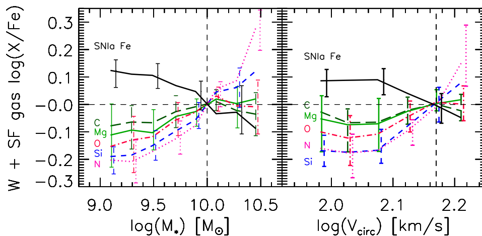
Figure 8. Median abundance of X/Fe for various elements X ( X = N, Si, O, Mg, C and Fe from Type Ia SNe only, as indicated in the legend), in star-forming gas at redshift z = 0 as a function of stellar mass M_* and circular velocity V_{\text{circ}} (left and right panels, respectively); error bars denote the 25th and 75th percentiles. For the sake of clarity, not all error bars are shown and we applied a small offset in the horizontal direction between some error bars to improve visibility. Abundances are off-set vertically by a constant W chosen such that they are all equal at M_* = 10^{10} M_{\odot} ( V_{\text{circ}} = 150 \text{ km s}^{-1} in the right panel), W = -0.685 (C), 0.127 (Mg), -1.08 (O), -0.14 (Si), 0.03 (N) and 0.36 (Fe from SNIa only). The ratio N/Fe increases dramatically with increasing M_* or V_{\text{circ}} , whereas the contribution of Fe from Type I SNe decreases; these two elements bracket the behaviour of the others.
