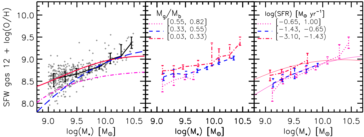
Figure 1. SFR-weighted gas-phase oxygen abundance, O/H , as a function of galaxy stellar mass, M_* , at redshift z = 0 . Left panel: full GIMIC sample of central galaxies (small symbols) with mean and 25 and 75th percentiles shown as black solid line with error bars. The red solid, blue dashed and pink dot-dashed lines are observational fits from Mannucci et al. (2010), Lara-López et al. (2010) and Sánchez et al. (2013), respectively. There are significant systematic differences between the observational fits, both in amplitude and in shape. The simulated abundances are consistent with the data at lower masses but may be slightly higher at the most massive end, M_* \approx 10^{10.5} M_\odot . Middle panel: same as left panel but for GIMIC galaxies binned in gas fraction, f_g = M_g/(M_g + M_*) = M_g/M_b . At given M_* , gas-rich galaxies have lower O/H . Right panel: same as left panel, but for galaxies binned in SFR, \dot{M}_* . At given M_* , galaxies with higher \dot{M}_* have lower O/H , consistent with the observed trend from Mannucci et al. (2010) shown for \log(\text{SFR}) = -2 and 0 as red and pink line, respectively.
