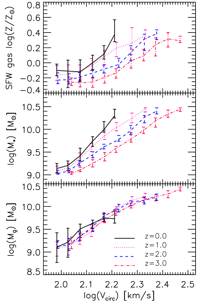
Figure 7. SFR-weighted gas-phase metallicity (upper panel), stellar mass (middle panel) and gas mass (lower panel) as a function V_{\text{circ}} at various redshifts indicated in the legend. Curves denote median relations, with error bars depicting the 25th and 75th percentiles. At a given V_{\text{circ}} , galaxies tend to have higher metallicities and higher stellar masses, at lower z , but similar gas masses.
