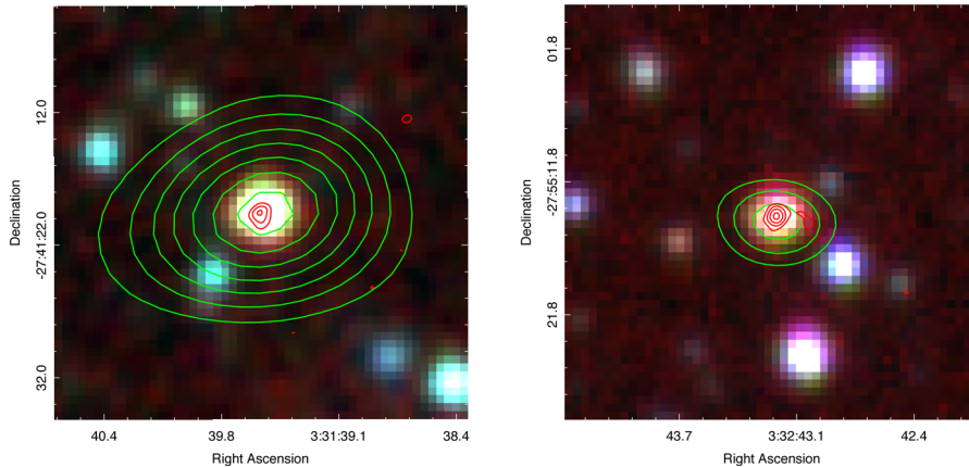
Figure 2. False-colour images made from Spitzer Infrared Array Camera (IRAC) images of Damen et al. (2011) 1 for ALESS 122.1(left) and ALESS 67.1 (right). Green contours indicate the CO(1–0) emission from the 600 \text{ km s}^{-1} cube at 3, 5, 7... \times \sigma . The red contours are from the ALMA 870 \mu\text{m} continuum map (Hodge et al. 2013) at 3, 5, 7... \times \sigma . The postage stamp images are 30 \times 30 arcsec.
