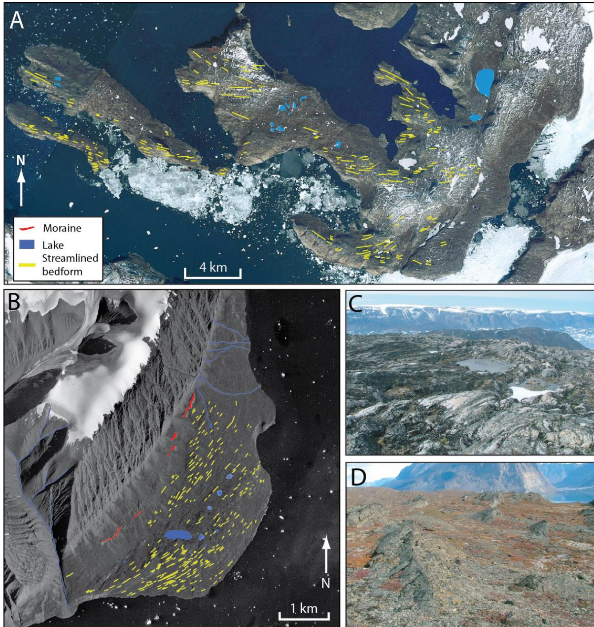
Fig. 4. A. Areally scoured topography from the southern Uummannaq region, with large lineations/macro-scale bedforms mapped. B. Areally scoured terrain from the northern Uummannaq region, with erosional bedforms mapped. C. Photograph of the areally scoured topography from the south of the Uummannaq region, showing classic knock and lochan topography. D. Photograph of areally scoured topography in the north of the Uummannaq region, with long, angular bedforms evident.
