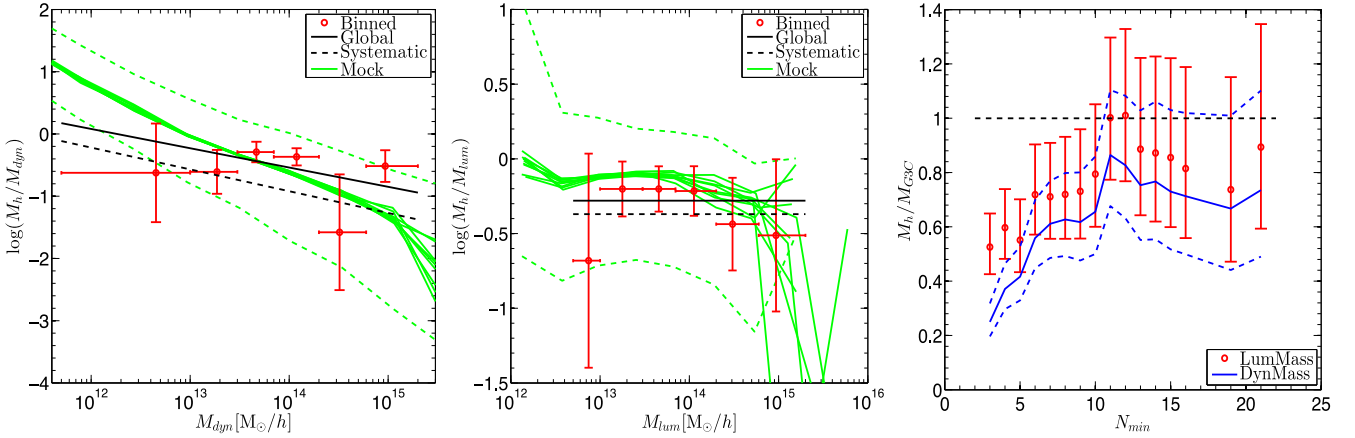
Figure 10. Left-hand and middle panels: the biases of HM with respect to the G^3Cv5 mass estimates, where G^3Cv5 mass refers to dynamical (left-hand) and luminosity (middle) mass in the two panels. In both cases, the red data points are the MLWL measured mass ratio within each G^3Cv5 mass bin; the black solid line is a power-law MLWL fit to the mass ratio- G^3Cv5 mass relation in the whole sample; the black dashed line is the fit with systematic corrections; the green solid lines are the median relations in the nine mock catalogues, while the green dashed lines mark the typical 16th and 84th (i.e. \pm 1\sigma ) percentiles in one mock. Note that for luminosity mass the power-law fit gives a slope so close to zero that we have fixed it to be zero. Right-hand panel: the measured bias of the G^3Cv5 mass estimates adopting different multiplicity cuts N_{min} . The red points with error bars show the bias of the G^3Cv5 luminosity mass. The blue solid line is the measured bias of the G^3Cv5 dynamical mass, and the blue dashed lines are the error bounds.
