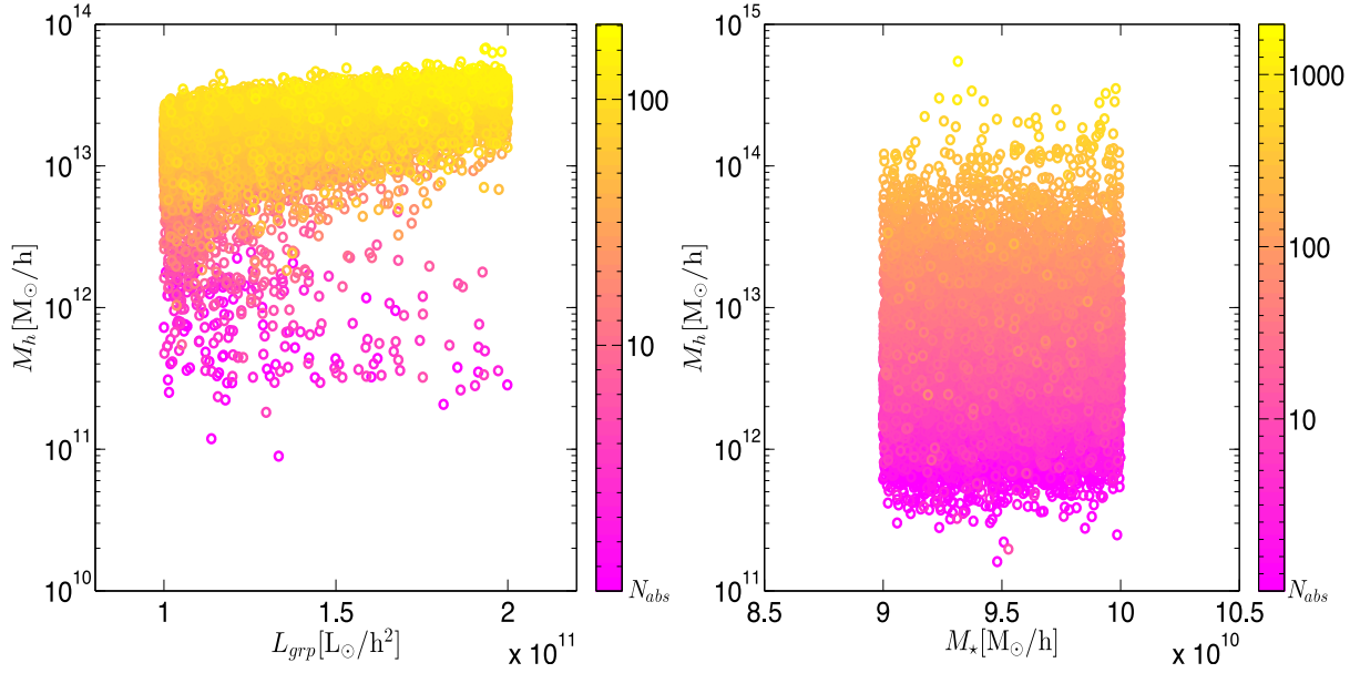
Figure B2. The role of group absolute multiplicity in the mass-observable relations. In the left-hand panel, we plot the HM–luminosity relation for all haloes with 10^{11} h^{-2} L_{\odot} < L_{\text{grp}} < 2 \times 10^{11} h^{-2} L_{\odot} , colour-coded by N_{\text{abs}} . The right-hand panel is similar but for the HM–central galaxy SM relation of systems with central galaxy SM in the range 9 \times 10^{10} h^{-2} M_{\odot} < M_{*} < 10^{11} h^{-2} M_{\odot} .
