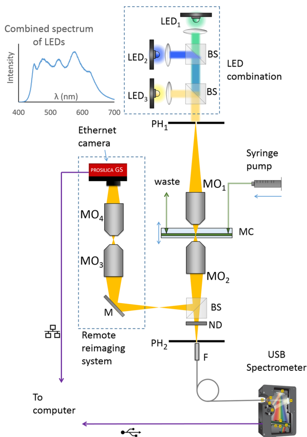
Fig. 2 A schematic of the experimental set-up, for each channel. Abbreviations BS = 50:50 beam splitter, ND = neutral density filter (OD=0.2), F = 0.22NA fibre, PH 1 /PH 2 = 200 μm (for channel a) or 400 μm (for channel b) diameter pinhole, M = mirror, MC = microfluidic channel
