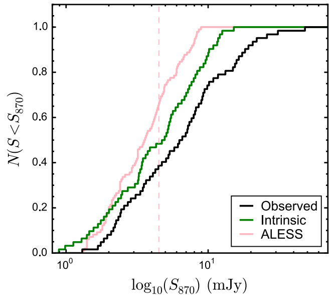
Figure 5. Cumulative distribution functions showing the effect of lensing on the inferred flux densities of the Herschel -ALMA sample. The median flux density in the Herschel -ALMA sample drops by a factor of 1.3 when lensing is taken into account. For comparison we also show the flux density distribution from ALESS (pink line), with the completeness limit of the ALESS survey indicated by a dashed pink line.
