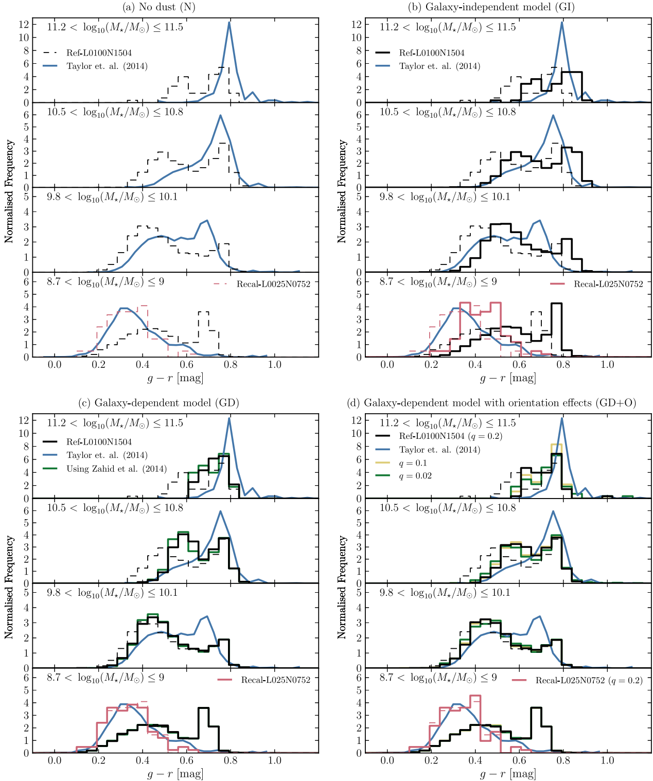
Figure 1. Rest-frame g-r colour distributions for EAGLE galaxies at redshift z = 0.1 , using four different models (panels a–d) for four non-contiguous ranges in stellar mass as indicated in the legend (top to bottom). Black lines indicate the fiducial Ref-100 galaxy population, while red lines indicate the higher resolution Recal-25 simulation. Dashed lines denote the unobscured SED (model N); these are repeated in each panel for comparison. Models shown are: model N without dust (panel a, see Section 3.1.5), model GI with galaxy independent dust (panel b, see Section 3.2.1), model GD where the dust obscuration depends on gas fraction and metallicity (panel c, Section 3.2.2), and model GD+O that in addition takes into account orientation effects (panel d, Section 3.2.3). Green and yellow lines show model variations in panels (c) and (d) (see sections 3.2.2–3.2.3 for details). Blue lines represent observed galaxy colours for the volume-limited sample of GAMA galaxies from Taylor et al. (2015). The figure shows the subtle quantitative effects that our different dust models have on the colour distributions of EAGLE galaxies in various M_* regimes, as is discussed further in the text.
