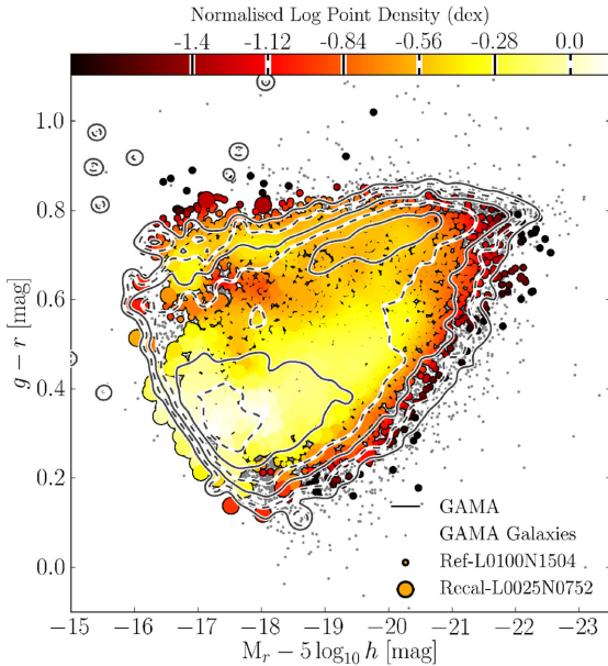
Figure 4. Rest-frame g-r colour as a function of r -band absolute magnitude for EAGLE galaxies (colours) compared to a volume-limited sample of GAMA galaxies (Taylor et al. 2015, contour lines). Contours and point shading is the same as in Fig 2, with the normalized contour levels indicated on the colour bar. EAGLE photometry is obtained using the GD+O model. A composite EAGLE galaxy population is used, consisting of galaxies from Ref-100 at M_* > 10^9 M_\odot and Recal-25 at M_* < 10^9 M_\odot as in the right-hand panel of Fig 2. There is general agreement between EAGLE and GAMA in the location and slope of the red-sequence ( g-r \approx 0.7 at M_r - 5 \log_{10} h = -20 ), the appearance of a blue cloud of galaxies with g-r \sim 0.45 at that magnitude, which becomes increasingly blue ( g-r \sim 0.3 ) for the fainter galaxies with M_r - 5 \log h \sim -17.5 .
