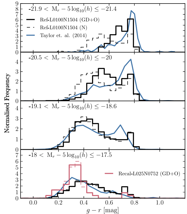
Figure 5. Rest-frame g-r colour distributions for EAGLE galaxies at redshift z = 0.1 for four non-contiguous ranges in r -band magnitude as indicated in the legend (top to bottom). Black lines indicate the fiducial Ref-100 galaxy population, while red lines indicate the higher resolution Recal-25 simulation. Dashed lines denote the N photometry with solid lines representing the fiducial GD+O. Blue lines represent observed galaxy colours for the volume-limited sample of GAMA galaxies from Taylor et al. (2015).
