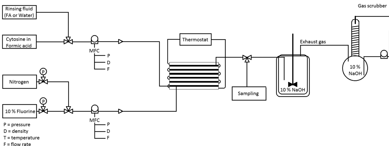
Figure 2. Continuous flow reactor system for the manufacture of flucytosine.
