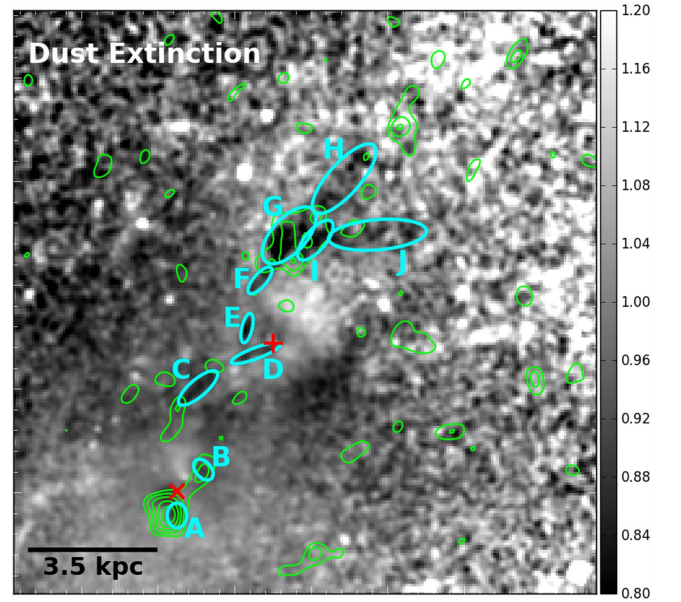
Figure 12. Dust extinction map of the HST F606W image. Regions with significant dust extinction are identified by the green ellipses, with statistics shown in Table 4. The BCG and companion galaxy centroids are identified by the red × and +, respectively. The image is shown in the same field of view as the ALMA CO(1–0) image (Figures 1 and 9). The CO(1–0) contours from Figure 1 have been overlaid for reference.
