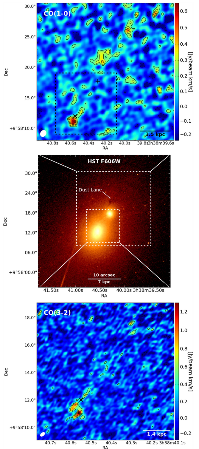
Figure 1. Top: integrated flux of the CO(1–0) ALMA image. The contours are -2, 2, 3, 4, 5\sigma, \dots where \sigma = 0.095 \text{ Jy beam}^{-1} \text{ km s}^{-1} . The \times indicates the position of a radio AGN determined from VLBI (Sanders et al. 2009), and the + indicates the flux centroid of the companion galaxy determined from the HST F606W image. The 1.13 \times 0.92 \text{ arcsec} (PA -35^\circ ) synthesized beam is shown in white in the lower left corner. The box indicates the CO(3–2) frame shown in the bottom panel. Middle: HST WFPC2 F606W optical image of the 2A 0335+096 BCG and the nearby companion galaxy. Bottom: integrated flux of the CO(3–2) ALMA image, with contours set at -3, 3, 5, 7, and 9\sigma , where \sigma = 0.145 \text{ Jy beam}^{-1} \text{ km s}^{-1} . The 0.32 \times 0.20 \text{ arcsec} beam is shown in white in the lower left corner.
