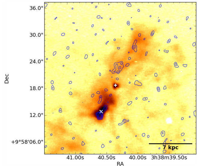
Figure 13. H\alpha emission from Donahue (2007) overlaid with the CO(1–0) contours from Figure 1. The \times and + indicate the nuclei of the BCG and companion galaxy, respectively. The coordinate reconstruction of the H\alpha image is accurate to \sim 1'' .
