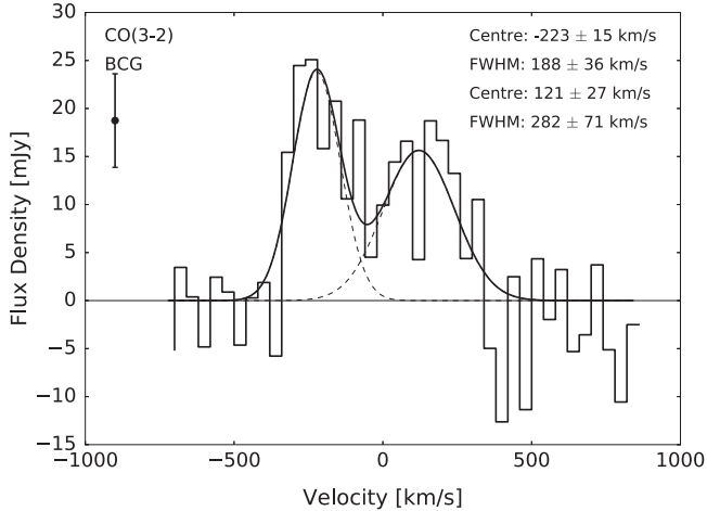
Figure 4. CO(3–2) spectrum of the BCG extracted from the same region as Figure 3 (top panel). The best-fit parameters are given in Table 1. The error bar indicates the rms variation in the line-free channels.
