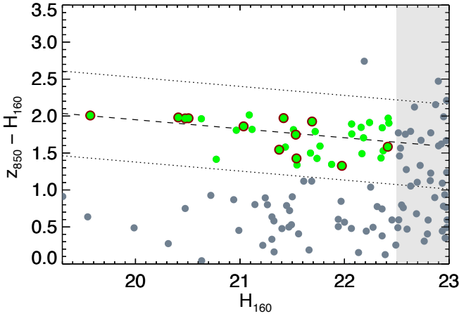
Figure 1. Colour-magnitude diagram of the cluster XMMUJ2235. WFC3 H_{160} magnitudes are MAG_AUTO magnitudes while the z_{850} - H_{160} colour are 1'' aperture magnitudes. The dashed line corresponds to the fitted red sequence and the dotted lines are \pm 2\sigma . Green circles correspond to objects that are included in our sample, which are within the dotted line and are not in the shaded area (i.e. H_{160} < 22.5 ). Objects that are spectroscopically confirmed cluster members from the catalogue of Grützbauch et al. (2012) are circled in dark red.
