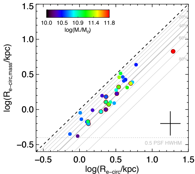
Figure 12. Comparison between mass-weighted size R_{e-circ,mass} and light-weighted size R_{e-circ} of passive galaxies in the cluster XMMUJ2235-2557. Spectroscopically confirmed objects are circled in dark red. The dashed line is the one-to-one relation. Each successive grey line represents a 10% decrement to the one-to-one relation. 50% decrement are marked with a thick grey line. The galaxies are colour coded with their integrated mass. The cross shows the median uncertainty of the light-weighted sizes and mass-weighted sizes. Note that the two uncertainties are correlated to some extent.
