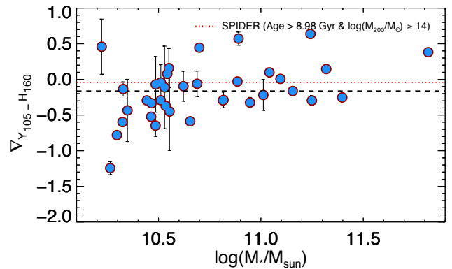
Figure E1. Y_{105} - H_{160} colour gradients in the cluster XMMUJ2235-2557. At redshift 1.39, this roughly corresponds to rest-frame g - r colour gradient. The red dotted line shows the median local g - r gradient from the SPIDER cluster sample. The black dashed line shows the median Y_{105} - H_{160} colour gradients.
