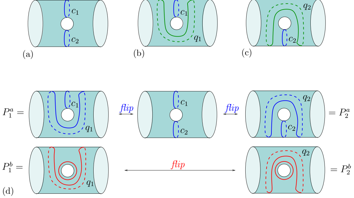
FIGURE 5. To the proof of Case 3.2.
