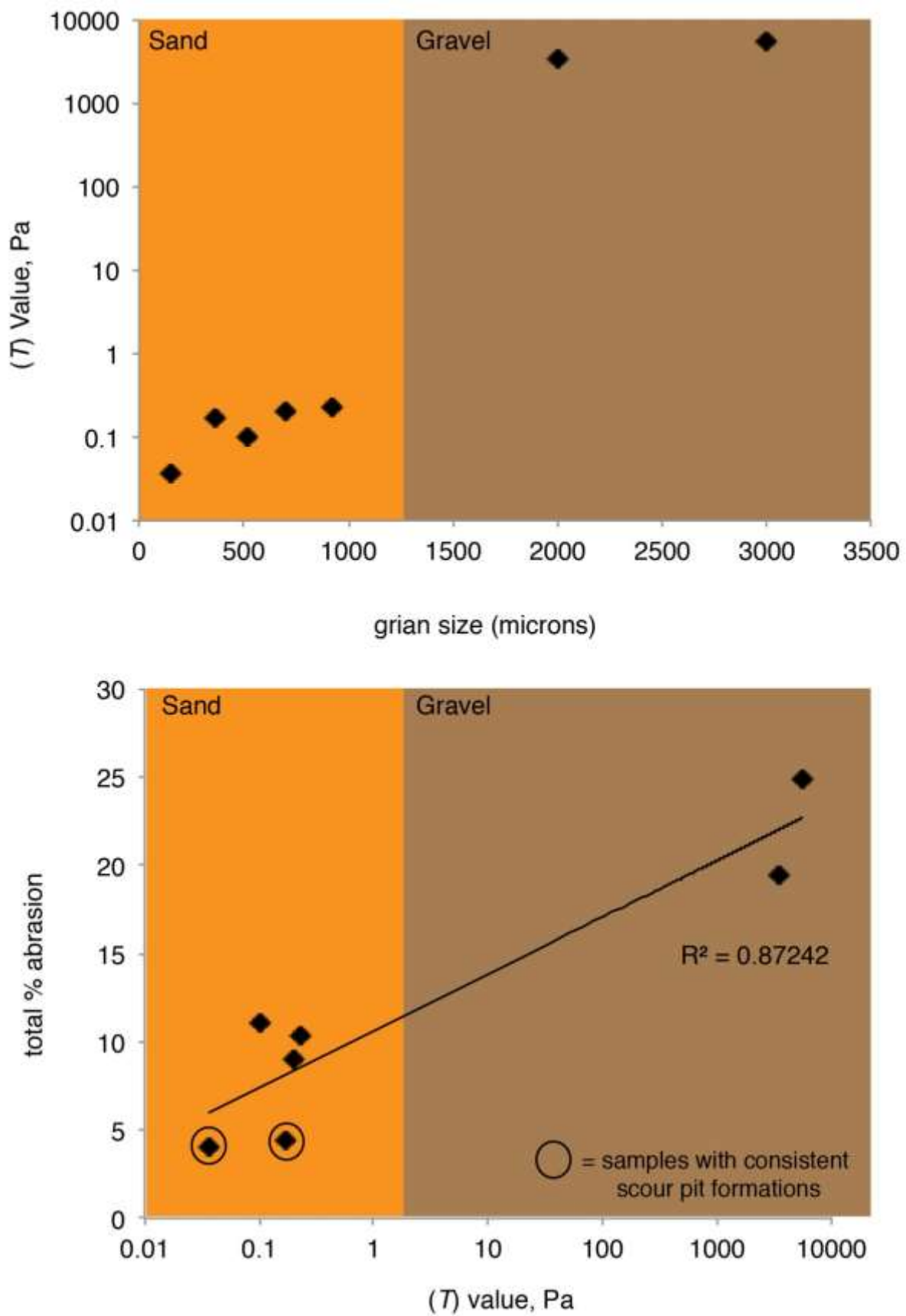
Figure 7. Top: Relationship between grain size and (T) Value. Bottom: Total % abrasion vs (T) value (Note total abrasion data points are averaged from 270 image cells).
