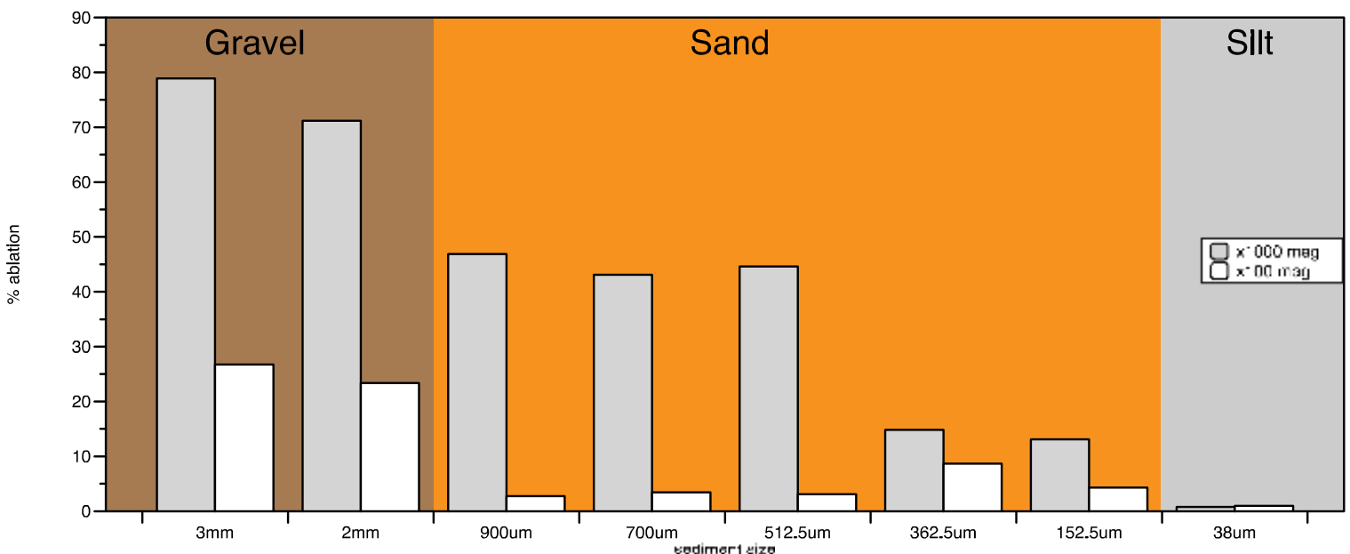
Figure 8. Percentage ablation recorded at both magnifications with sand showing minimal abrasion at \times 100 mag.
