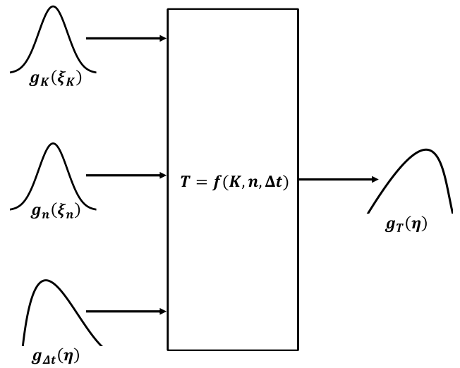
Figure 17. PDF propagation of K , n and \Delta t to provide the PDF of T through the zebra tape torque meter model (Adapted with permission from [30]. Permission to reproduce extracts from ISO publications is granted by BSI Standards Limited (BSI) on behalf of International Organization for Standardization (ISO). No other use of this material is permitted.)
