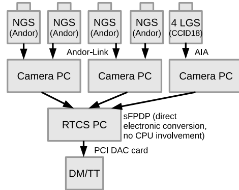
Figure 3. Phase B2 of CANARY showing the camera and DM connectivity.
