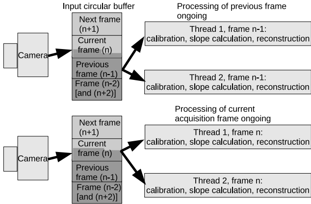
Figure 7. A figure showing how pixel data is handled in DARC. Camera pixels are directed to a small circular buffer which is then read by the sub-aperture processing threads. In the upper half, these threads are processing a completed frame, and in the lower half, the threads have moved on to begin processing the next, currently incomplete, frame.
