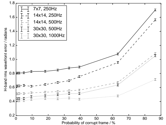
Figure 8. A figure showing AO performance (rms residual wavefront error) as a function of probability of a corrupt WFS frame (for any given frame). For CANARY, this probability is well below 1%.
