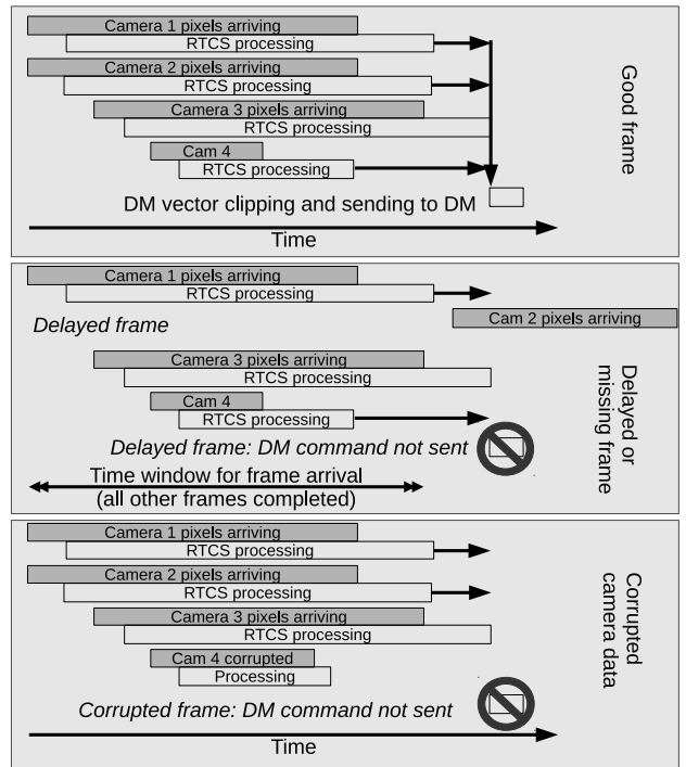
Figure 6. A figure showing three cases for pixel arrival. The top portion shows a good frame with all pixels arriving as expected. The middle case shows the action taken if one camera is delayed to beyond all others being finished (or fails to arrive). The third case shows arrival of a corrupted frame.
