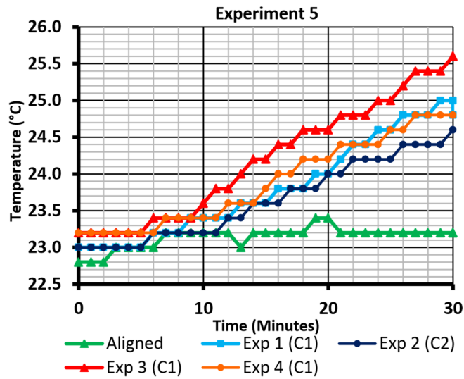
Figure 16 – Temperature plot – Exp 5 at 22 °C
