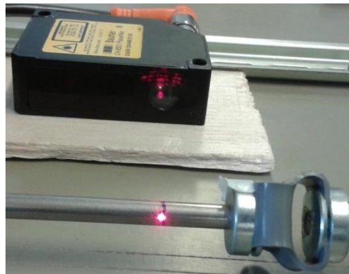
Figure 4 – Laser distance measurement
