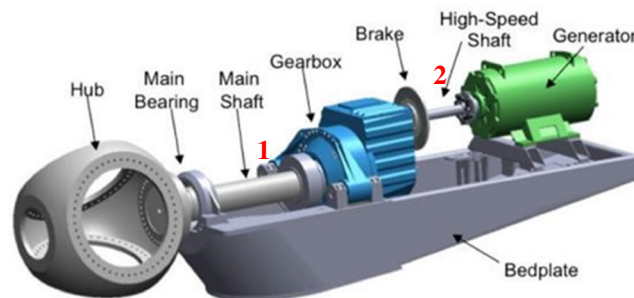
Figure 2 – Typical drivetrain layout
