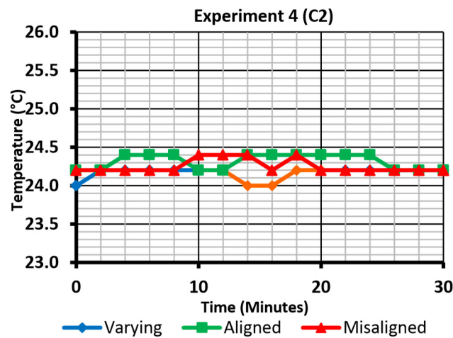
Figure 15 – Temperature plot – Exp 4 (C2) at 21 °C
