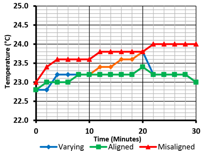
Figure 11 – Temperature plot – Exp 1 (C2) at 20 °C
