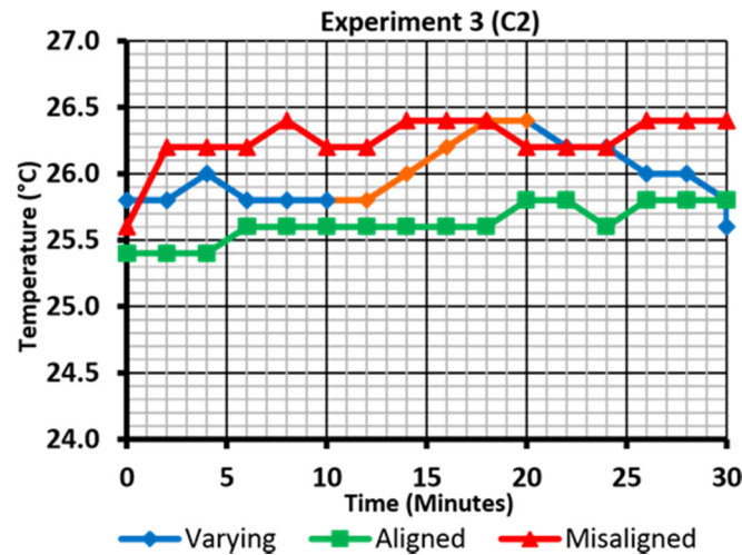
Figure 14 – Temperature plot – Exp 3 (C2) at 24 °C
