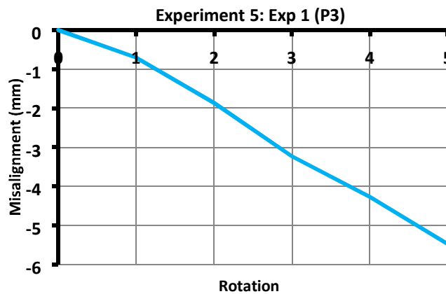
Figure 8 – Misalignment against rotation (left laser)
