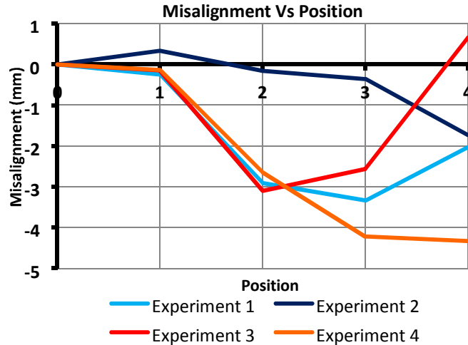
Figure 7 – Misalignment against position (left laser)
