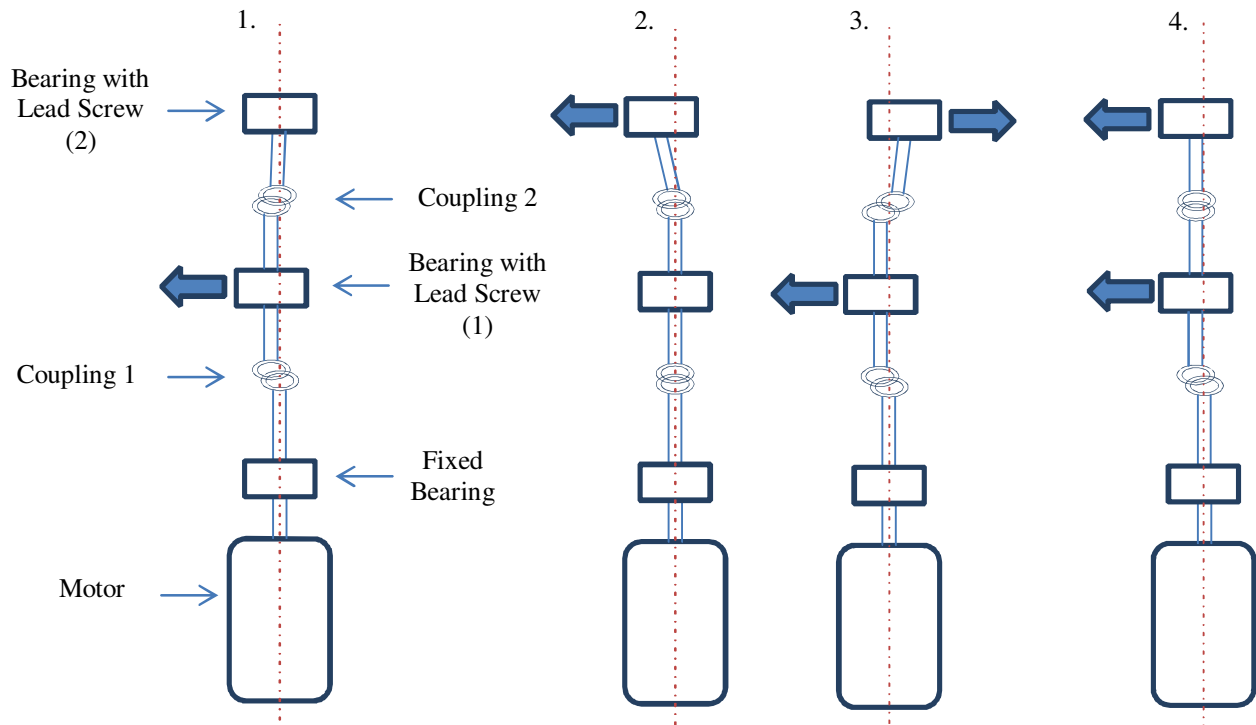
Figure 5 – Misalignment mode diagrams
