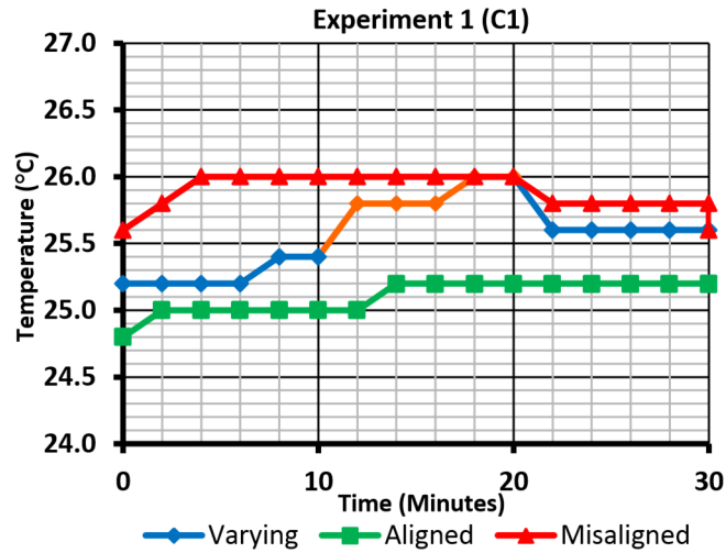
Figure 10 – Temperature plot – Exp 1 (C1) at 24 °C
