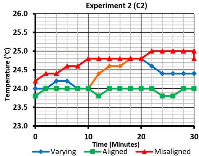
Figure 12 – Temperature plot – Exp 2 (C2) at 21 °C
