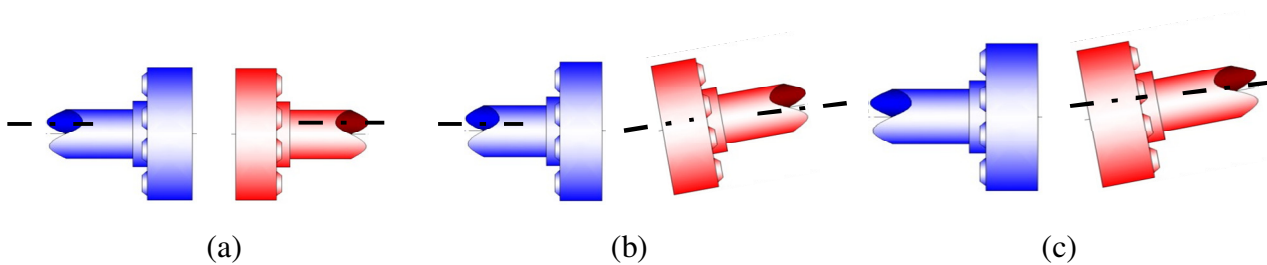
Figure 1 – Types of misalignment: (a) offset, (b) Angular and (c) combination of both
