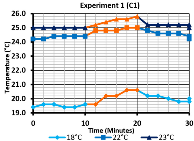
Figure 18 – Temperature plot – Exp 1 (C1) at different ambient temperatures
