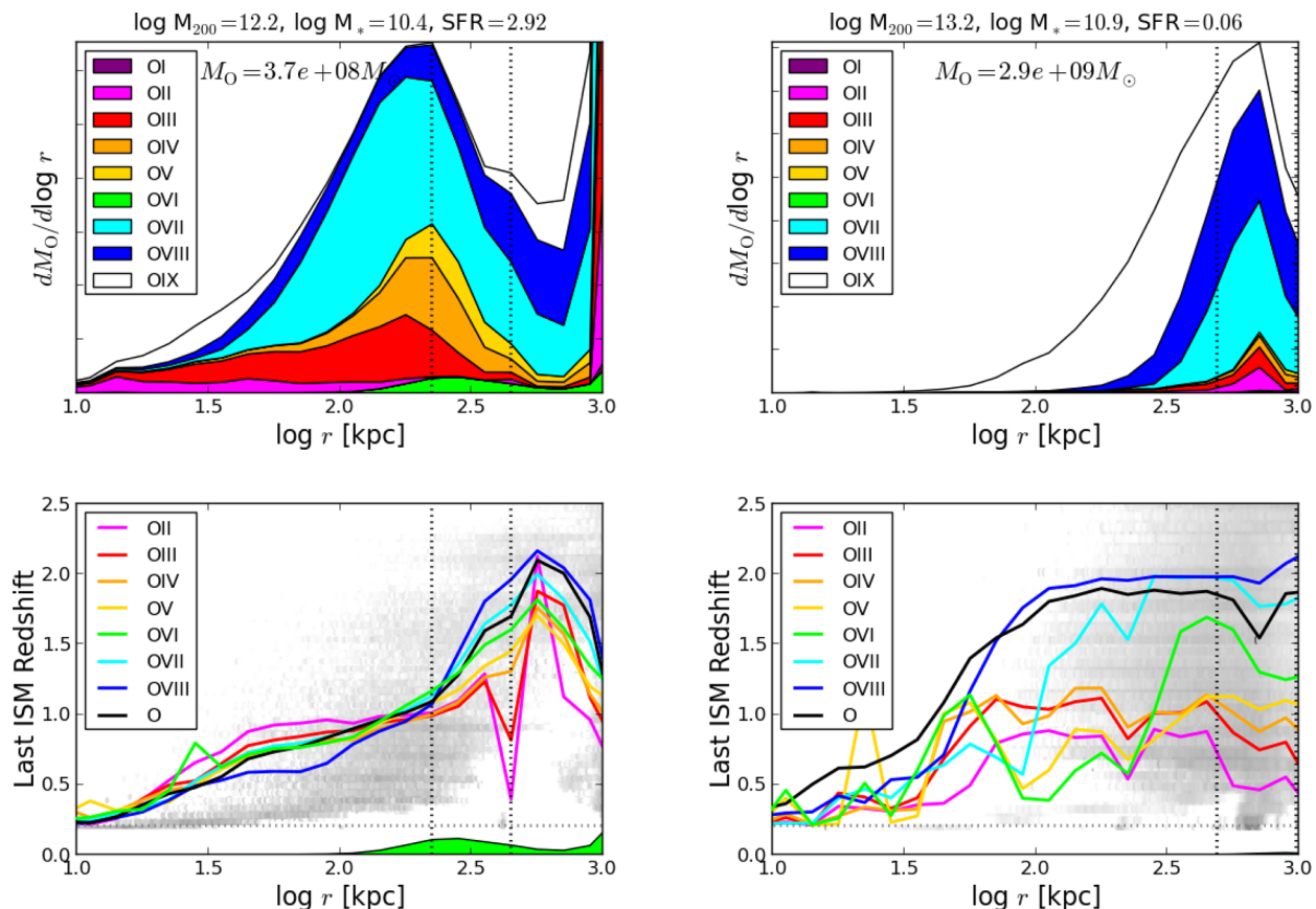
Figure 6. CGM oxygen as a function of radius is plotted in the top panels for the Gal005 L^* halo (left, M_{200} = 10^{12.2} M_{\odot} ) and the Grp008 group-sized halo (right, M_{200} = 10^{13.2} M_{\odot} ). The top solid line indicates the total oxygen content as a function of radius on a linear scale (y-axis values not specified). The total CGM oxygen content in each panel between 10^{1.05} and 10^{2.95} kpc is 3.7 \times 10^8 and 2.9 \times 10^9 M_{\odot} for the L^* and group haloes, respectively (listed on the top of each panel). The dotted vertical lines indicate R_{200} and 2R_{200} . The bottom panels indicate the age distribution of oxygen in grey shading, where we define age as the last redshift an SPH particle was in the ISM. The mean ages of oxygen species (coloured lines) and total oxygen (black line) are also shown. The grey horizontal dotted line is the redshift of the snapshot. We also repeat the O VI shading from the top panels in the age panels. O VI in L^* haloes primarily resides outside R_{200} and is greater than 5 Gyr old ( z > 1 ). Group-sized haloes enrich a more extended region at earlier times ( z \sim 2 ).
