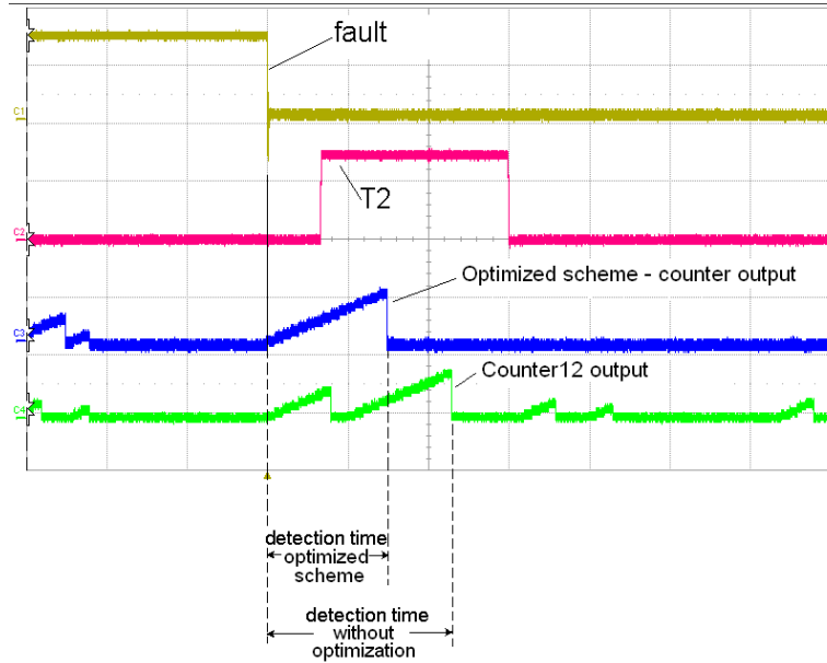
Fig. 17. Comparison of the fault detection times without and with the optimization for a fault in S1 and a transition in T2 during the fault detection. (y-axis from top to bottom: 10 V/div, 10 V/div, 33/div, 33/div; x-axis: 20 \mu\text{s}/\text{div} )
