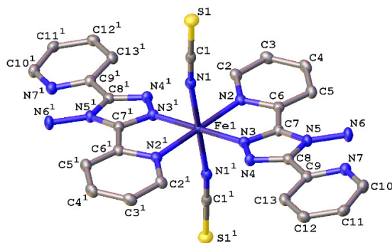
Figure 2 - Ellipsoid plot of [\text{Fe}(\text{abpt})_2(\text{NCS})_2] polymorph A at 120 K with the ellipsoids depicted at 50% probability level. The asymmetric unit (asu) consists of half a molecule and '1' represents the other half of the molecule which is symmetry generated by the operator 1-x, 1-y, 1-z . Hydrogen atoms have been omitted for clarity.
