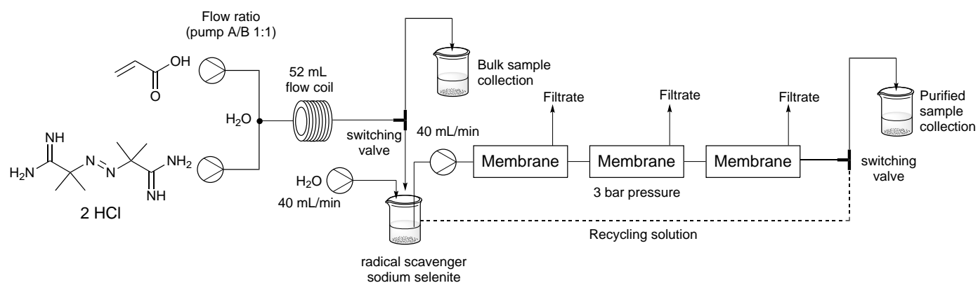
Fig. 8 a) System for the synthesis and purification of poly(acrylic acid) b) A: Reagent feed lines, B: Piston pumps, C: Mixer, D: Reactor, E: Back-pressure regulator, F: Sample collection, G: Peristaltic pump to feed membranes, H: Ultrafiltration membranes, I: Pressure regulator, J: Filtrate of purification, K: HPLC pump used to maintain the sample volume.
