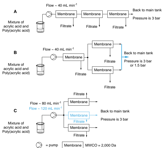
Fig. 2 A: Three membranes in series with the outlet connected to the polymer reservoir. B: Combination of two membranes in parallel and series, outlet(s) is/ are separated or combined. The outlet(s) is/are connected to the polymer reservoir. C: Two or three membranes in parallel, outlets are connected to the polymer reservoir.
