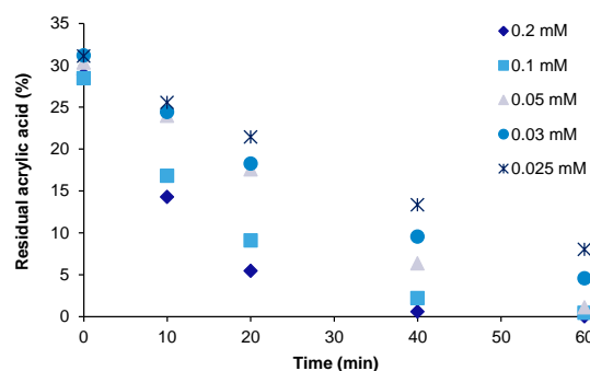
Fig. 6 Extraction rates for different concentration and volumes (Table 2) of residual acrylic acid performed using three membranes in series as shown in Figure 2A.
